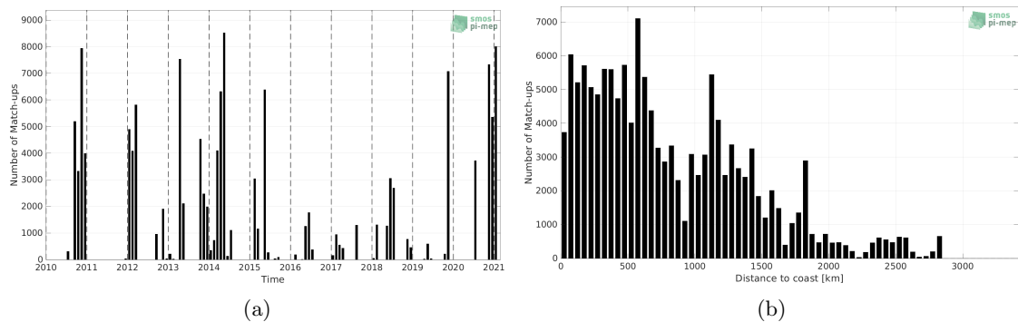
Figure 1: Number of match-ups between TSG (GOSUD-Sailing-ship) and SMOS SSS L2 v700 (ESA) SSS as a function of time (a) and as function of the distance to coast (b) over the Atlantic Ocean Pi-MEP region and for the full satellite product period.
