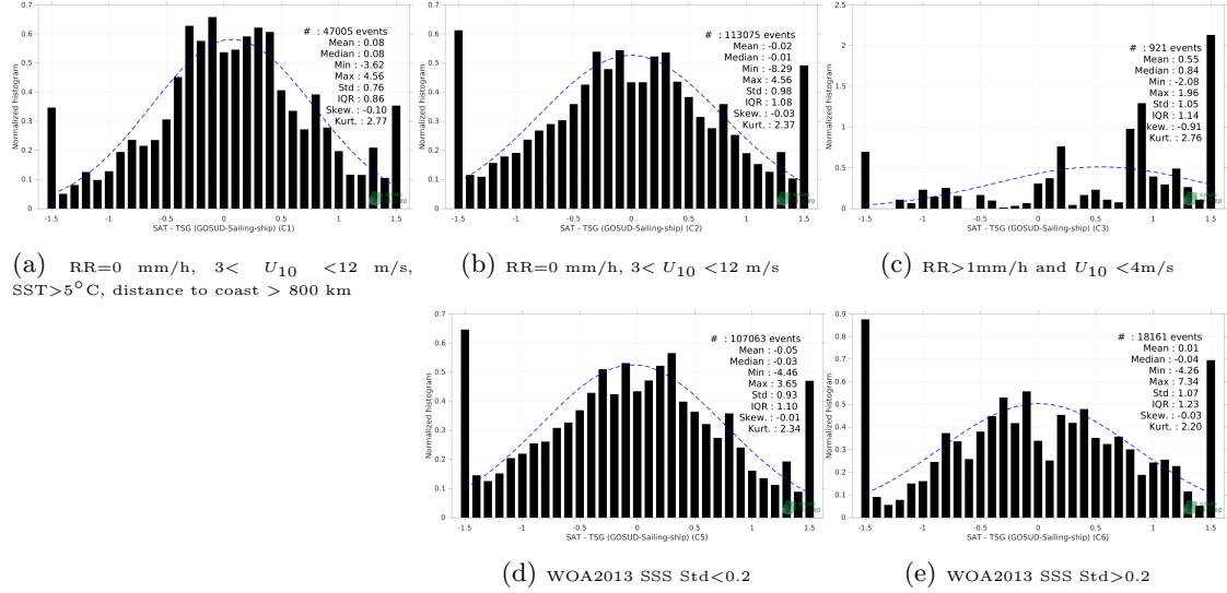
Figure 13: Normalized histogram of \Delta\text{SSS} (SMOS SSS L2 v700 (ESA) - TSG (GOSUD-Sailing-ship)) for 5 different subdatasets corresponding to: RR=0 mm/h, 3 < U_{10} < 12 m/s, SST>5°C, distance to coast > 800 km (a), RR=0 mm/h, 3 < U_{10} < 12 m/s (b), RR>1mm/h and U_{10} < 4 m/s (c), WOA2013 SSS Std<0.2 (d), WOA2013 SSS Std>0.2 (e).
