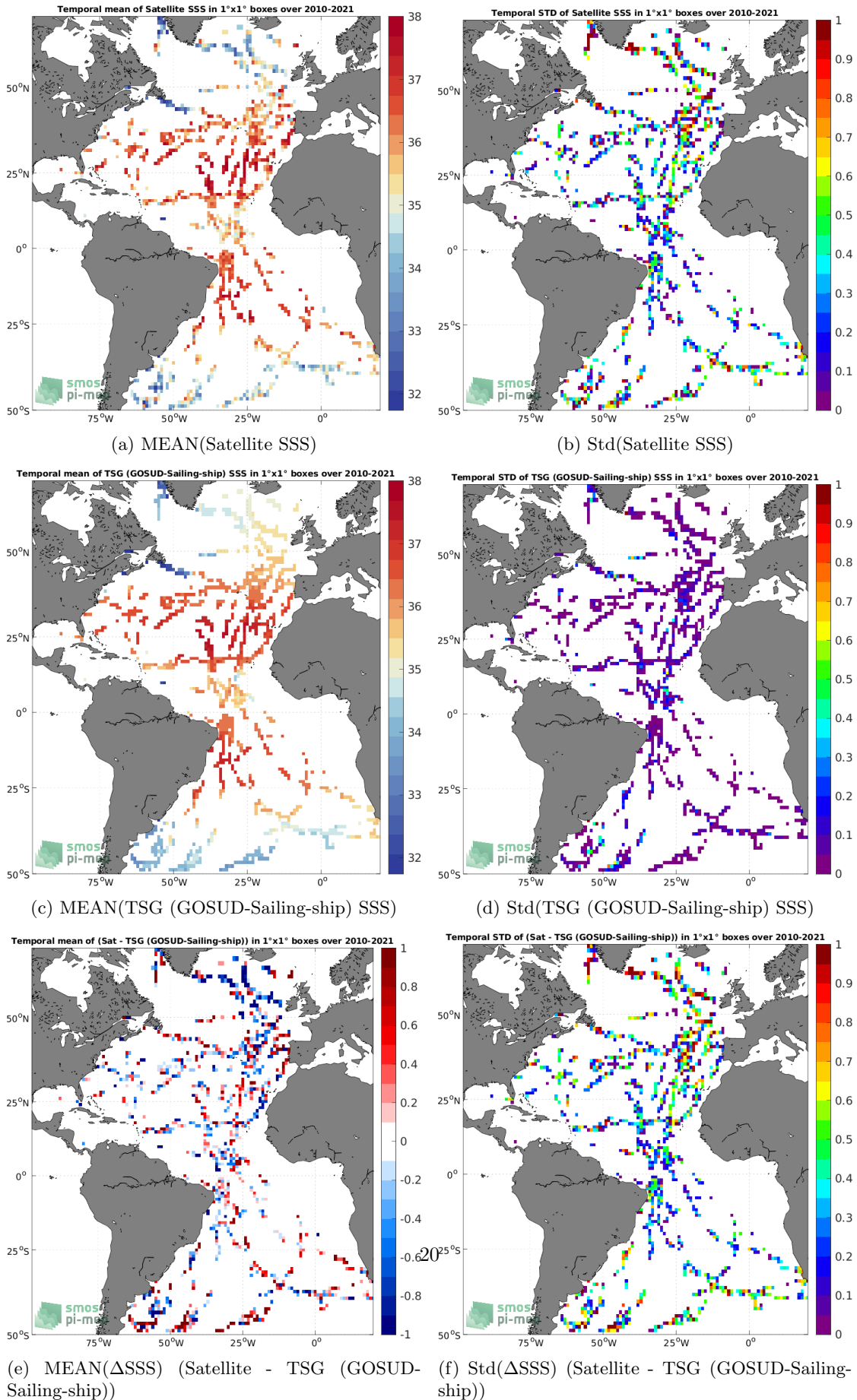
Figure 6: Temporal mean (left) and Std (right) of SSS from SMOS SSS L2 v700 (ESA) (top), TSG (GOSUD-Sailing-ship) (middle), and of \Delta SSS (Satellite - TSG (GOSUD-Sailing-ship)). Only match-up pairs are used to generate these maps.
