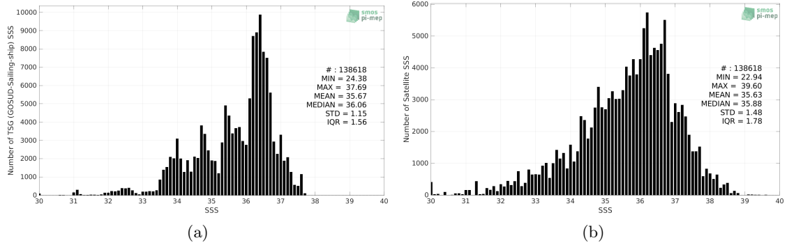
Figure 2: Histograms of SSS from TSG (GOSUD-Sailing-ship) (a) and SMOS SSS L2 v700 (ESA) (b) considering all match-up pairs per bins of 0.1 over the Atlantic Ocean Pi-MEP region and for the full satellite product period.
