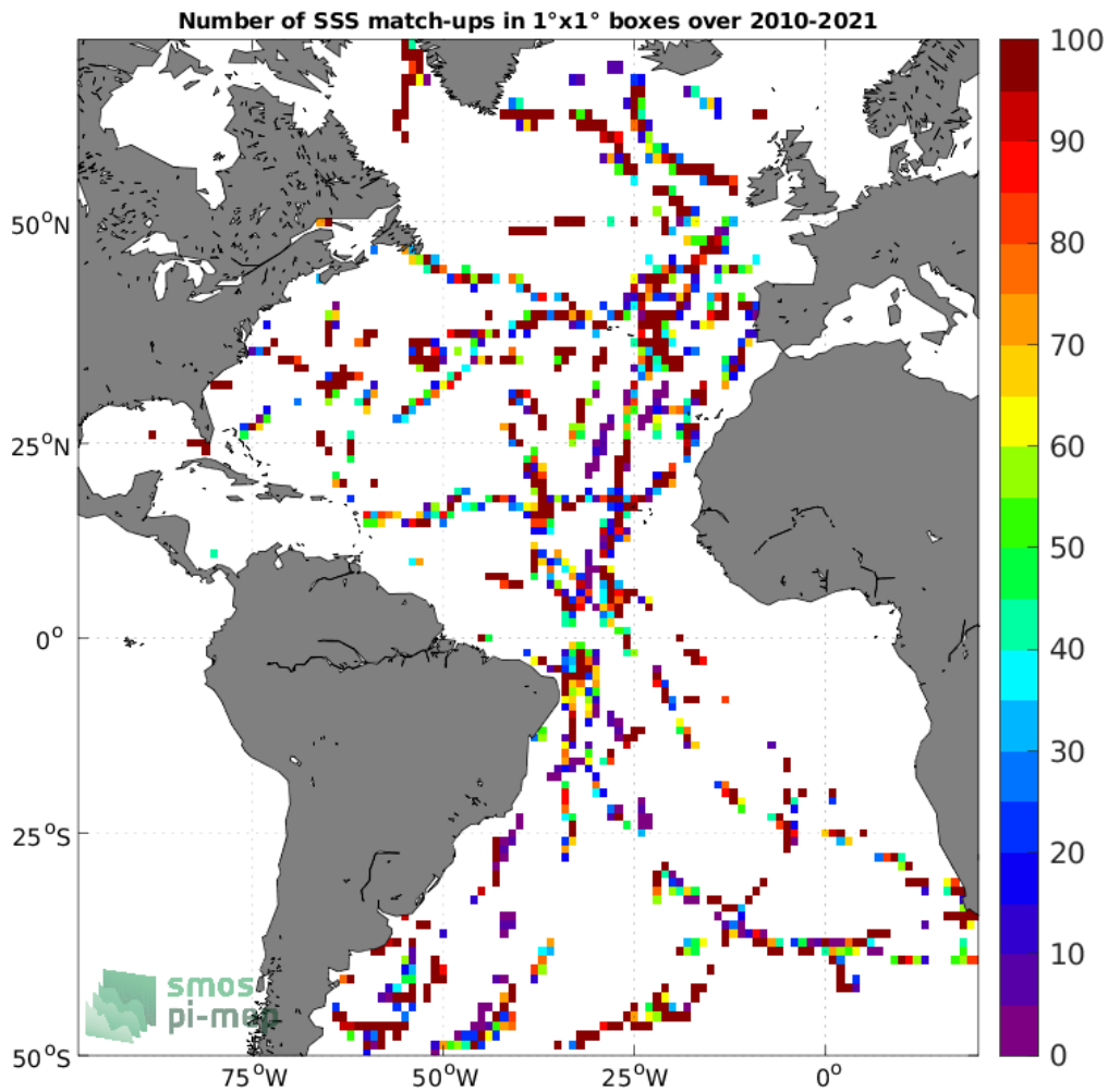
Figure 4: Number of SSS match-ups between TSG (GOSUD-Sailing-ship) SSS and the SMOS SSS L2 v700 (ESA) SSS product for the Atlantic Ocean Pi-MEP region over 1°x1° boxes and for the full satellite product period.
