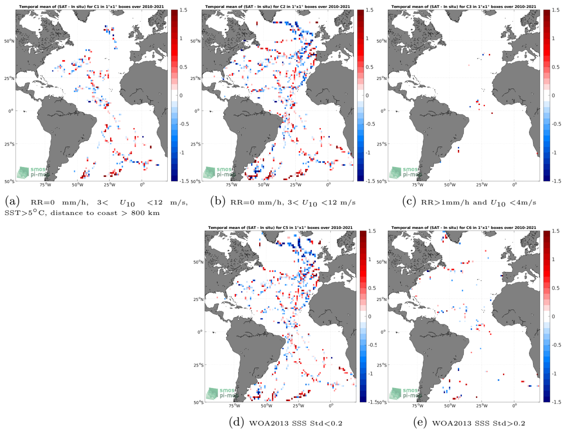
Figure 12: Temporal mean gridded over spatial boxes of size 1^\circ \times 1^\circ of \Delta SSS (SMOS SSS L2 v700 (ESA) - TSG (GOSUD-Sailing-ship)) for 5 different subdatasets corresponding to:RR=0 mm/h, 3 < U_{10} < 12 m/s, SST>5°C, distance to coast > 800 km (a), RR=0 mm/h, 3 < U_{10} < 12 m/s (b), RR>1mm/h and U_{10} < 4 m/s (c), WOA2013 SSS Std<0.2 (d), WOA2013 SSS Std>0.2 (e).
