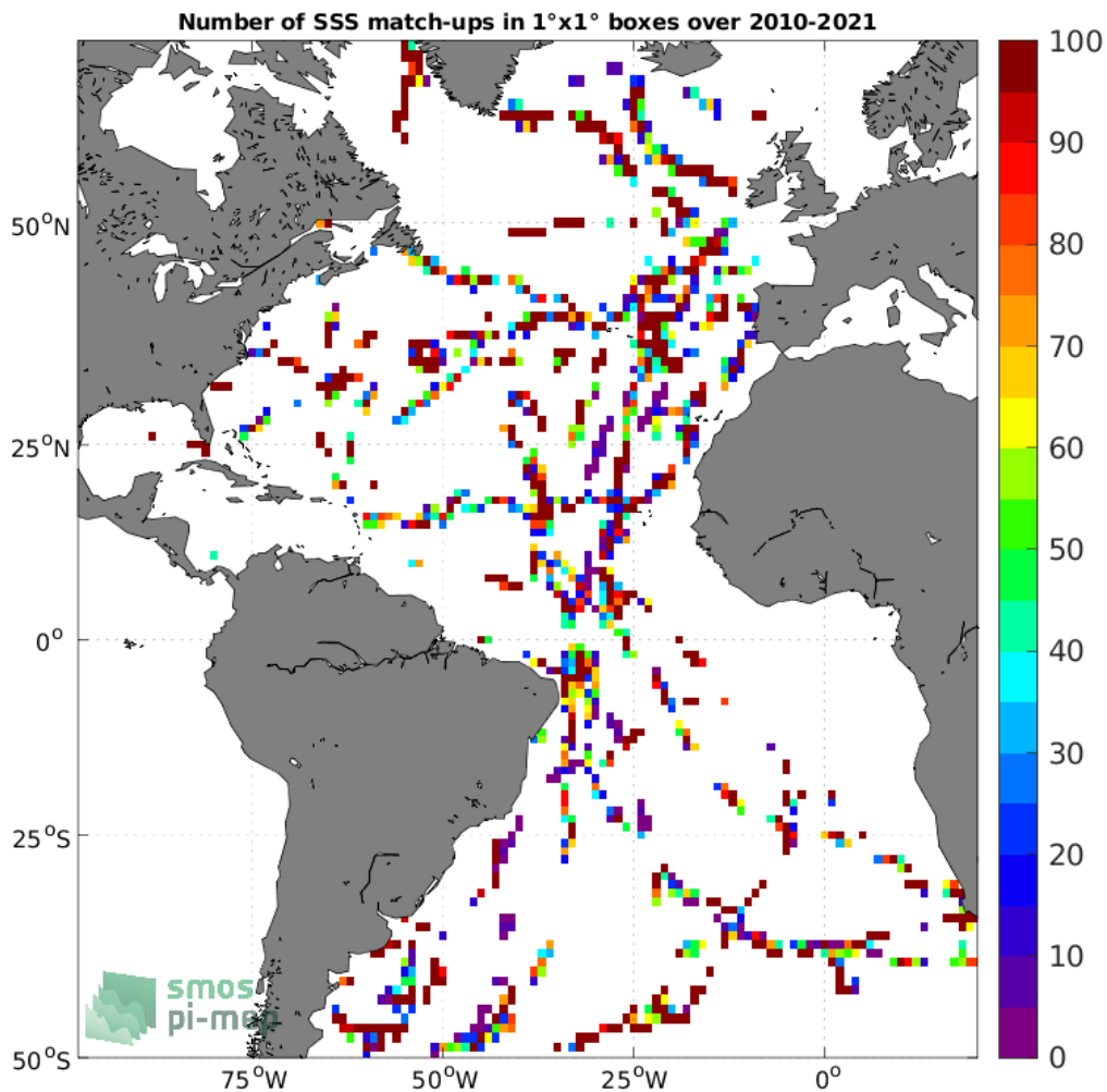
Figure 4: Number of SSS match-ups between TSG (GOSUD-Sailing-ship) SSS and the SMOS SSS L2 v700 (ESA) SSS product for the Atlantic Ocean Pi-MEP region over 1^\circ \times 1^\circ boxes and for the full satellite product period.
