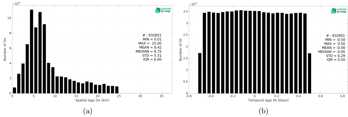
Figure 6: Histograms of the spatial (a) and temporal (b) lags between the location/time of the TSG (GOSUD-Research-vessel) measurement and the date of the corresponding SMOS SSS L2 v700 (ESA) SSS pixel.
