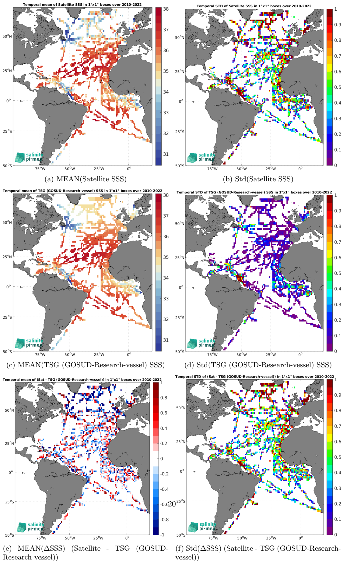
Figure 7: Temporal mean (left) and Std (right) of SSS from SMOS SSS L2 v700 (ESA) (top), TSG (GOSUD-Research-vessel) (middle), and of \Delta SSS (Satellite - TSG (GOSUD-Research-vessel)). Only match-up pairs are used to generate these maps.
