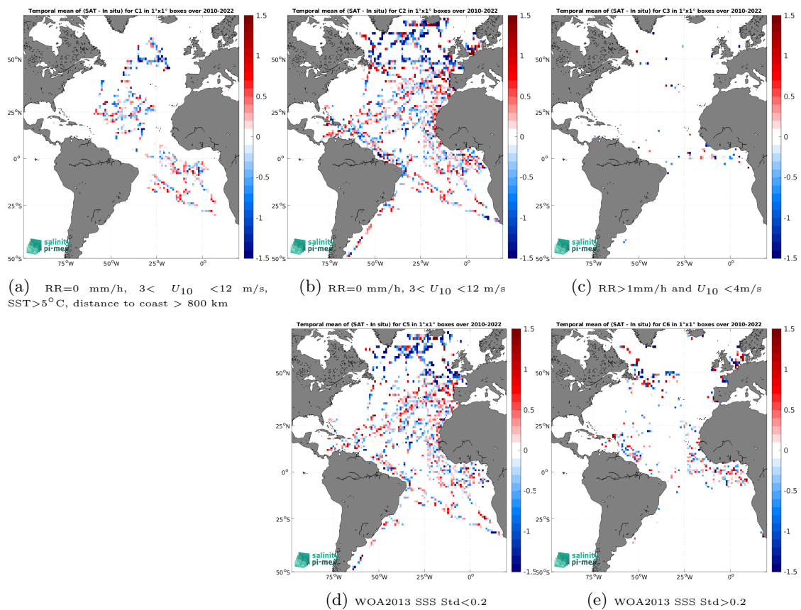
Figure 14: Temporal mean gridded over spatial boxes of size 1^\circ \times 1^\circ of \Delta\text{SSS} (SMOS SSS L2 v700 (ESA) - TSG (GOSUD-Research-vessel)) for 5 different subdatasets corresponding to:RR=0 mm/h, 3 < U_{10} < 12 m/s, SST>5°C, distance to coast > 800 km (a), RR=0 mm/h, 3 < U_{10} < 12 m/s (b), RR>1mm/h and U_{10} < 4 m/s (c), WOA2013 SSS Std<0.2 (d), WOA2013 SSS Std>0.2 (e).
