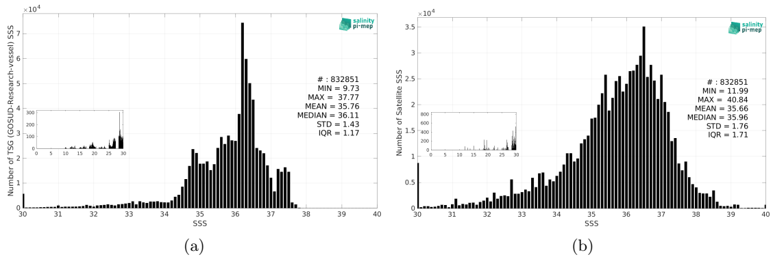
Figure 3: Histograms of SSS from TSG (GOSUD-Research-vessel) (a) and SMOS SSS L2 v700 (ESA) (b) considering all match-up pairs per bins of 0.1 over the Atlantic Ocean Pi-MEP region and for the full satellite product period.
