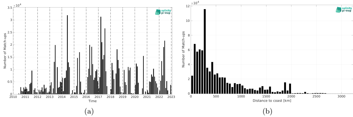
Figure 2: Number of match-ups between TSG (GOSUD-Research-vessel) and SMOS SSS L2 v700 (ESA) SSS as a function of time (a) and as function of the distance to coast (b) over the Atlantic Ocean Pi-MEP region and for the full satellite product period.
