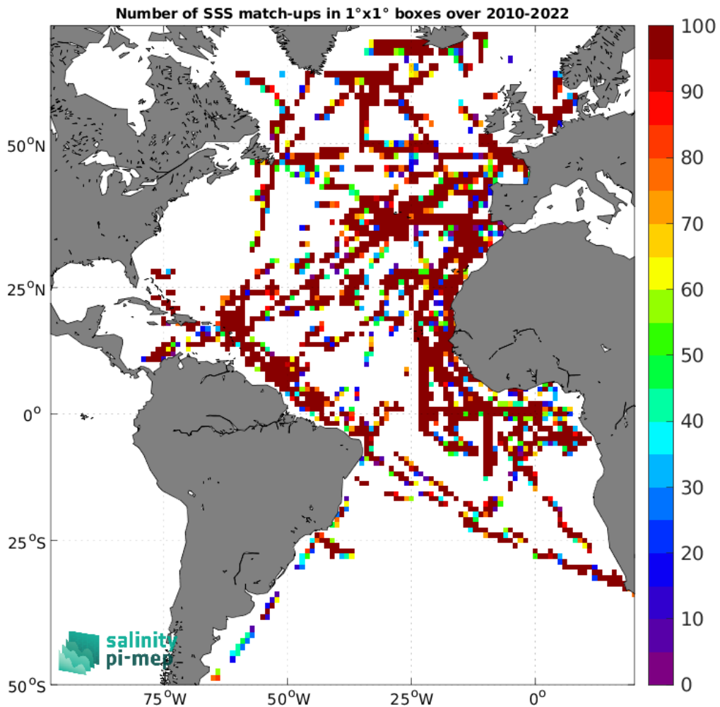
Figure 5: Number of SSS match-ups between TSG (GOSUD-Research-vessel) SSS and the SMOS SSS L2 v700 (ESA) SSS product for the Atlantic Ocean Pi-MEP region over 1°x1° boxes and for the full satellite product period.
