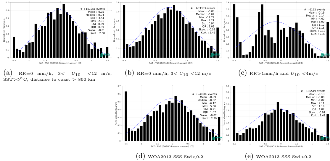
Figure 13: Normalized histogram of \Delta SSS (SMOS SSS L2 v700 (ESA) - TSG (GOSUD-Research-vessel)) for 5 different subdatasets corresponding to: RR=0 mm/h, 3 < U_{10} < 12 m/s, SST >5^{\circ} C, distance to coast > 800 km (a), RR=0 mm/h, 3 < U_{10} < 12 m/s (b), RR >1 mm/h and U_{10} < 4 m/s (c), WOA2013 SSS Std <0.2 (d), WOA2013 SSS Std >0.2 (e).
