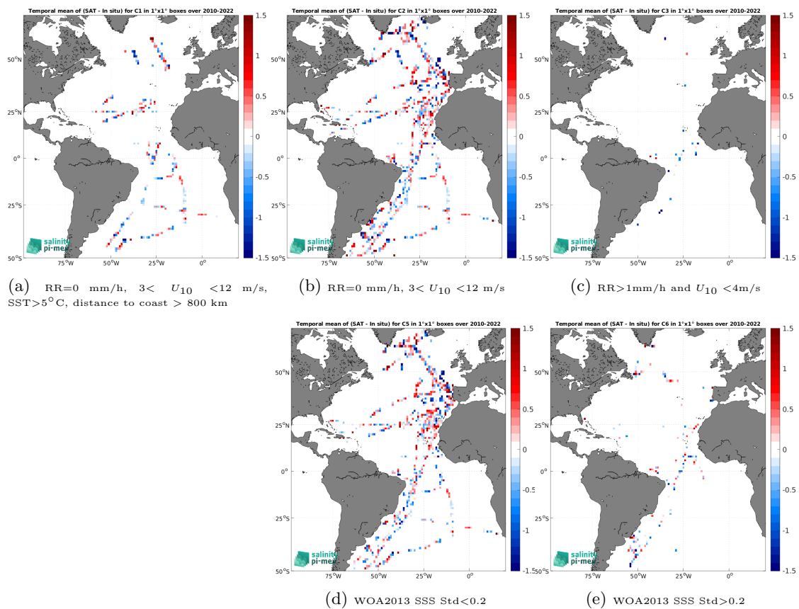
Figure 14: Temporal mean gridded over spatial boxes of size 1^\circ \times 1^\circ of \Delta\text{SSS} (SMOS SSS L2 v700 (ESA) - TSG (CSIC-UTM)) for 5 different subdatasets corresponding to:RR=0 mm/h, 3 < U_{10} < 12 m/s, SST>5°C, distance to coast > 800 km (a), RR=0 mm/h, 3 < U_{10} < 12 m/s (b), RR>1mm/h and U_{10} < 4 m/s (c), WOA2013 SSS Std<0.2 (d), WOA2013 SSS Std>0.2 (e).
