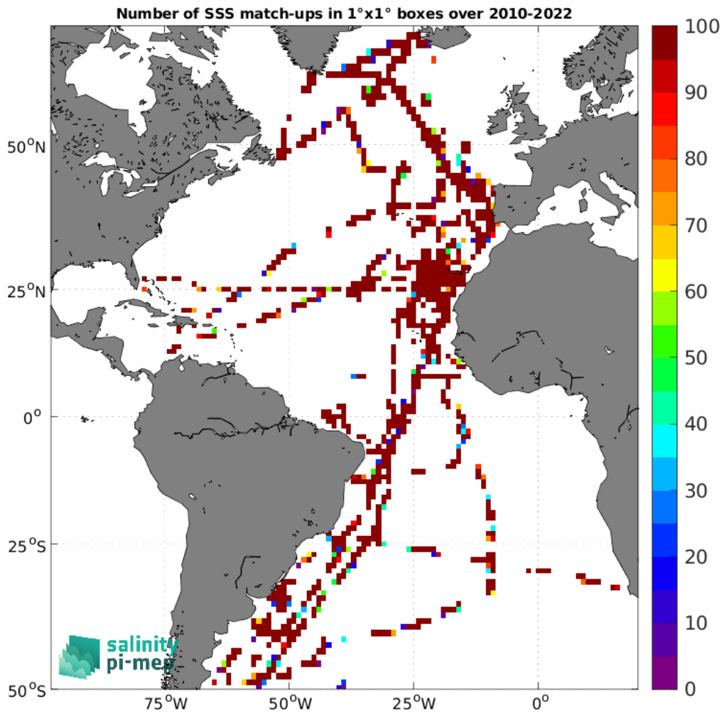
Figure 5: Number of SSS match-ups between TSG (CSIC-UTM) SSS and the SMOS SSS L2 v700 (ESA) SSS product for the Atlantic Ocean Pi-MEP region over 1°×1° boxes and for the full satellite product period.
