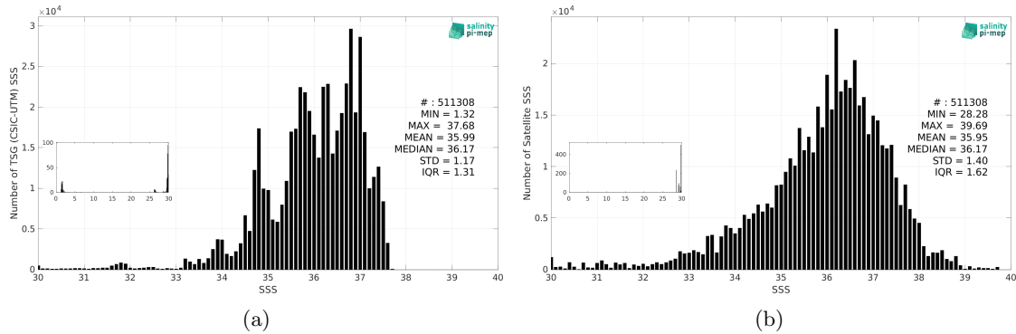
Figure 3: Histograms of SSS from TSG (CSIC-UTM) (a) and SMOS SSS L2 v700 (ESA) (b) considering all match-up pairs per bins of 0.1 over the Atlantic Ocean Pi-MEP region and for the full satellite product period.
