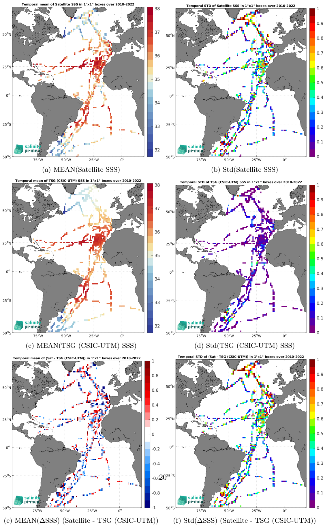
Figure 7: Temporal mean (left) and Std (right) of SSS from SMOS SSS L2 v700 (ESA) (top), TSG (CSIC-UTM) (middle), and of \Delta SSS (Satellite - TSG (CSIC-UTM)). Only match-up pairs are used to generate these maps.
