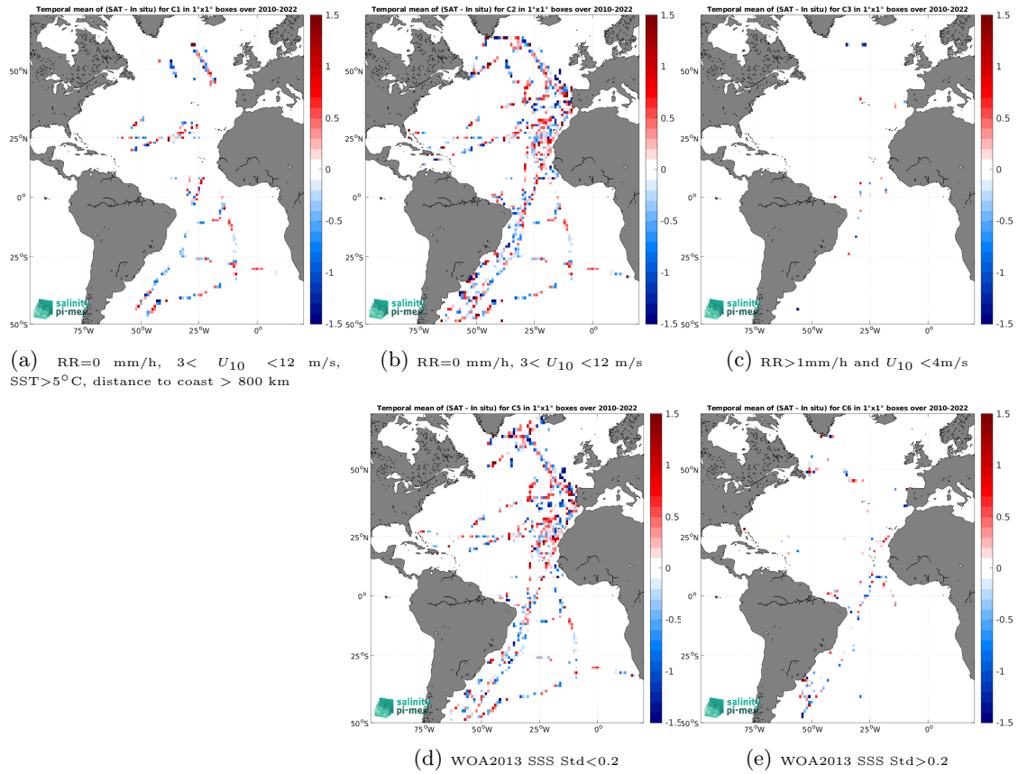
Figure 12: Temporal mean gridded over spatial boxes of size 1^\circ \times 1^\circ of \Delta SSS (SMOS SSS L2 v700 (ESA) - TSG (CSIC-UTM)) for 5 different subdatasets corresponding to:RR=0 mm/h, 3 < U_{10} < 12 m/s, SST >5^\circ\text{C} , distance to coast > 800 km (a), RR=0 mm/h, 3 < U_{10} < 12 m/s (b), RR >1 mm/h and U_{10} < 4 m/s (c), WOA2013 SSS Std <0.2 (d), WOA2013 SSS Std >0.2 (e).
