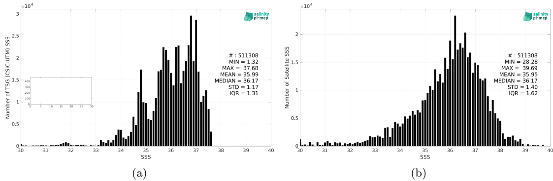
Figure 2: Histograms of SSS from TSG (CSIC-UTM) (a) and SMOS SSS L2 v700 (ESA) (b) considering all match-up pairs per bins of 0.1 over the Atlantic Ocean Pi-MEP region and for the full satellite product period.
