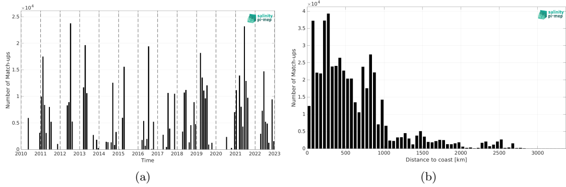
Figure 1: Number of match-ups between TSG (CSIC-UTM) and SMOS SSS L2 v700 (ESA) SSS as a function of time (a) and as function of the distance to coast (b) over the Atlantic Ocean Pi-MEP region and for the full satellite product period.
