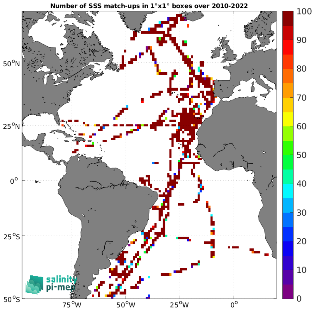
Figure 4: Number of SSS match-ups between TSG (CSIC-UTM) SSS and the SMOS SSS L2 v700 (ESA) SSS product for the Atlantic Ocean Pi-MEP region over 1^\circ \times 1^\circ boxes and for the full satellite product period.
