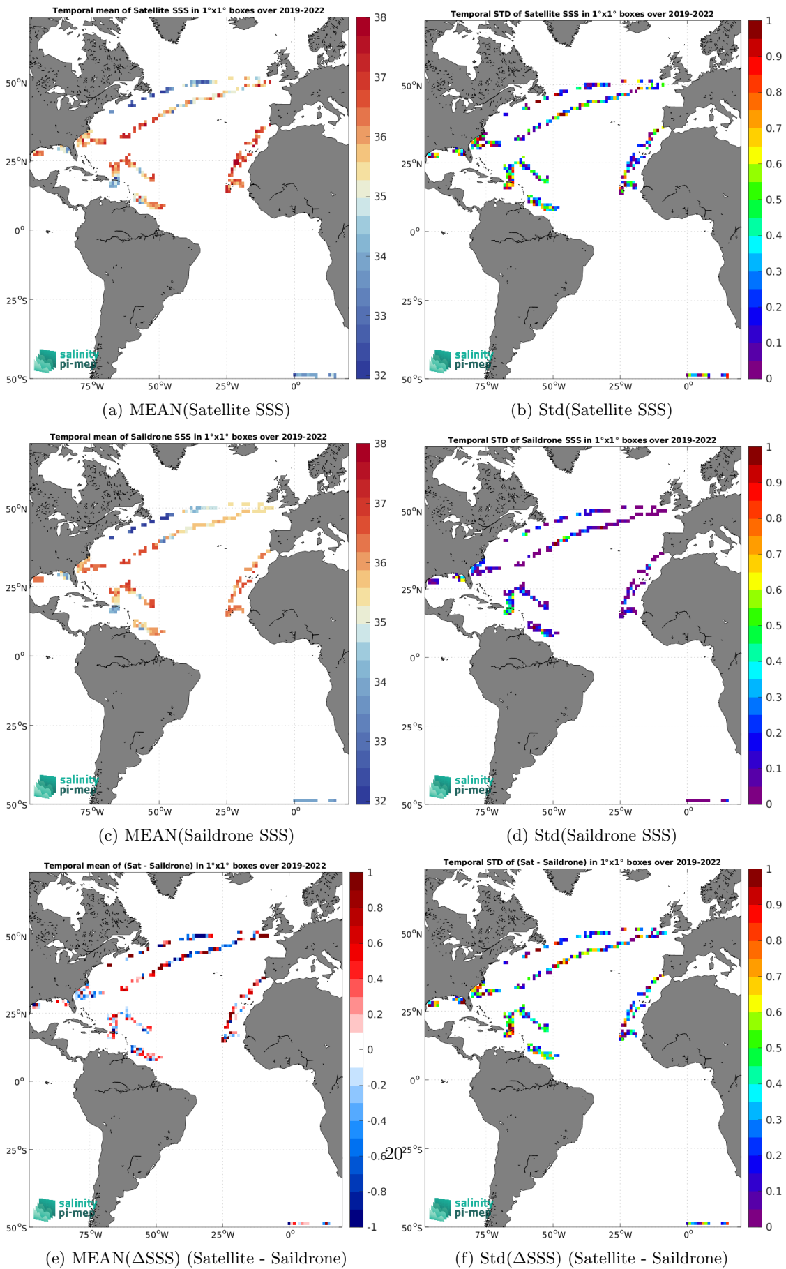
Figure 7: Temporal mean (left) and Std (right) of SSS from SMOS SSS L2 v700 (ESA) (top), Saildrone (middle), and of \Delta SSS (Satellite - Saildrone). Only match-up pairs are used to generate these maps.
