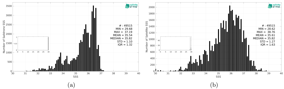
Figure 3: Histograms of SSS from Sairdrone (a) and SMOS SSS L2 v700 (ESA) (b) considering all match-up pairs per bins of 0.1 over the Atlantic Ocean Pi-MEP region and for the full satellite product period.
