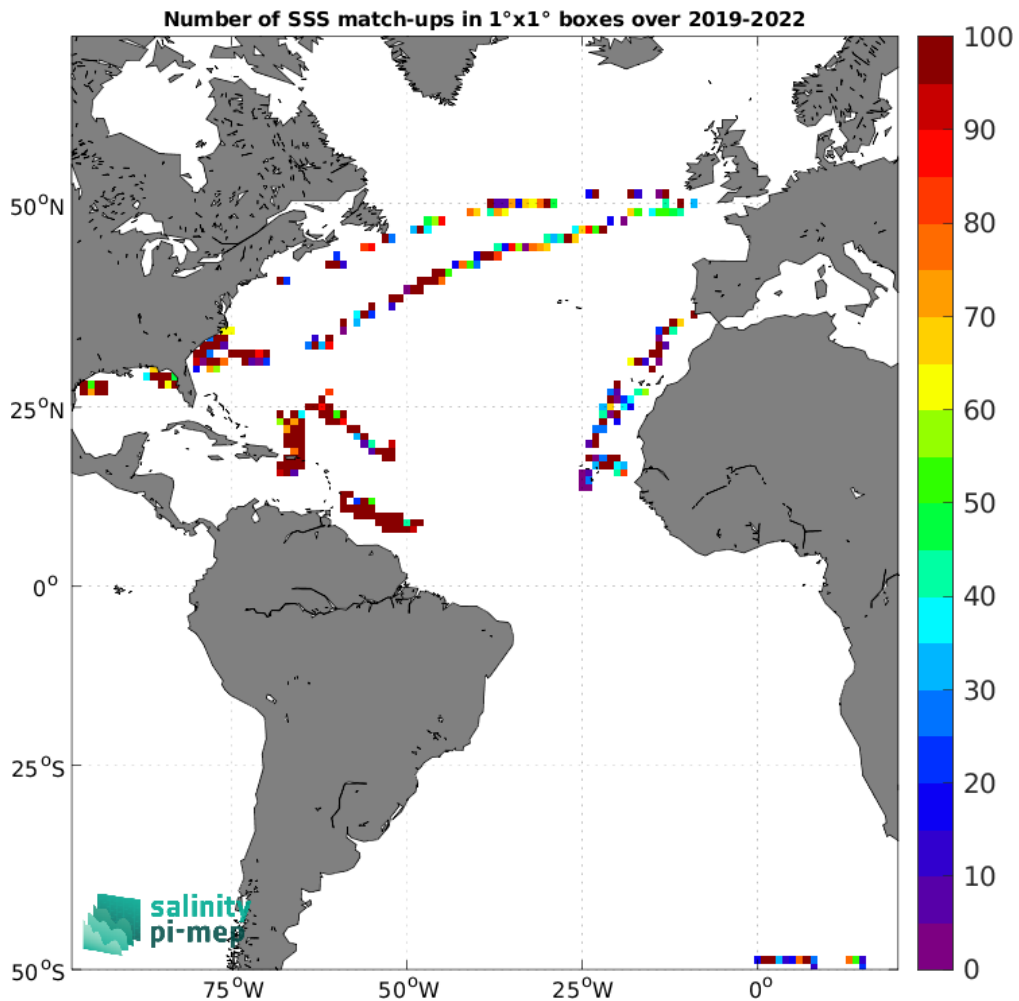
Figure 5: Number of SSS match-ups between Saildrone SSS and the SMOS SSS L2 v700 (ESA) SSS product for the Atlantic Ocean Pi-MEP region over 1°x1° boxes and for the full satellite product period.
