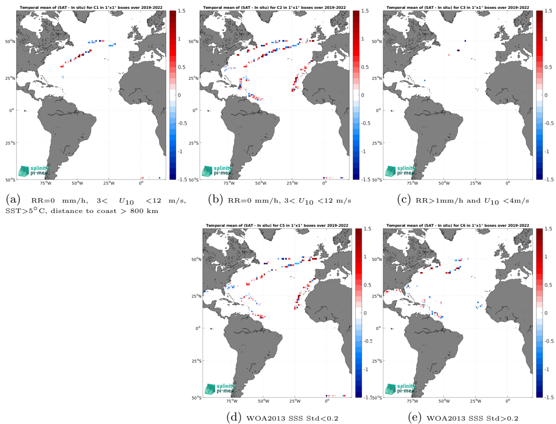
Figure 14: Temporal mean gridded over spatial boxes of size 1^\circ \times 1^\circ of \Delta\text{SSS} (SMOS SSS L2 v700 (ESA) - SAILDRONE) for 5 different subdatasets corresponding to:RR=0 mm/h, 3 < U_{10} < 12 m/s, SST >5^\circ\text{C} , distance to coast > 800 km (a), RR=0 mm/h, 3 < U_{10} < 12 m/s (b), RR >1 mm/h and U_{10} < 4 m/s (c), WOA2013 SSS Std <0.2 (d), WOA2013 SSS Std >0.2 (e).
