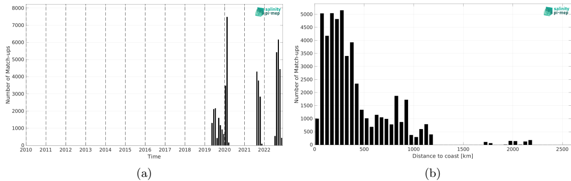
Figure 2: Number of match-ups between Sairdrone and SMOS SSS L2 v700 (ESA) SSS as a function of time (a) and as function of the distance to coast (b) over the Atlantic Ocean Pi-MEP region and for the full satellite product period.
