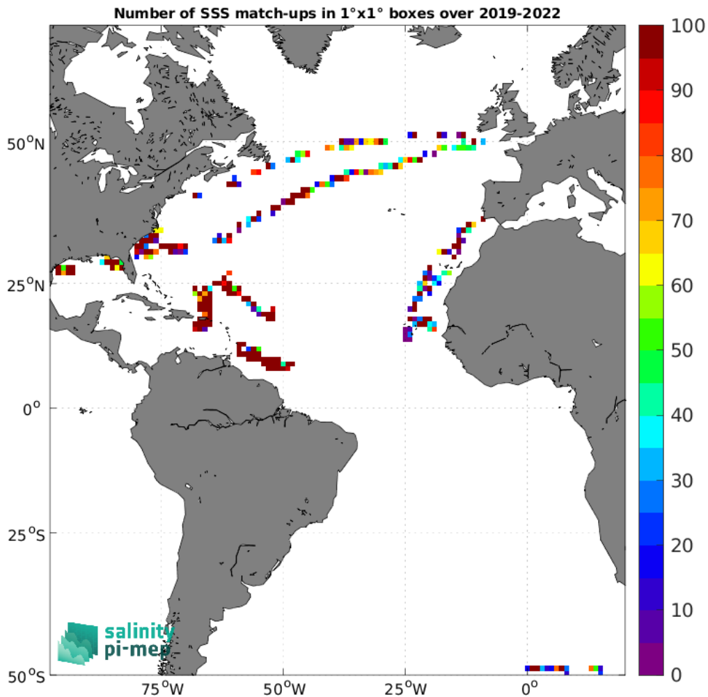
Figure 4: Number of SSS match-ups between Saildrone SSS and the SMOS SSS L2 v700 (ESA) SSS product for the Atlantic Ocean Pi-MEP region over 1°x1° boxes and for the full satellite product period.
