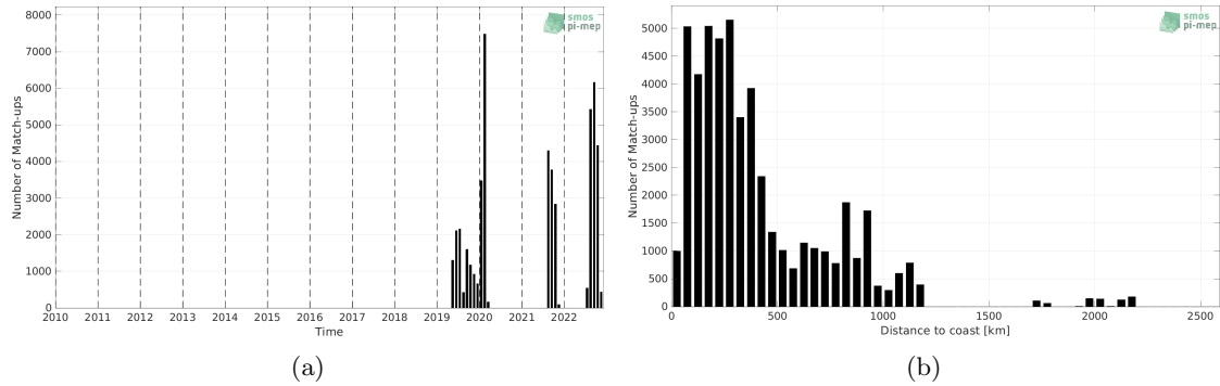
Figure 1: Number of match-ups between Sairdrone and SMOS SSS L2 v700 (ESA) SSS as a function of time (a) and as function of the distance to coast (b) over the Atlantic Ocean Pi-MEP region and for the full satellite product period.
