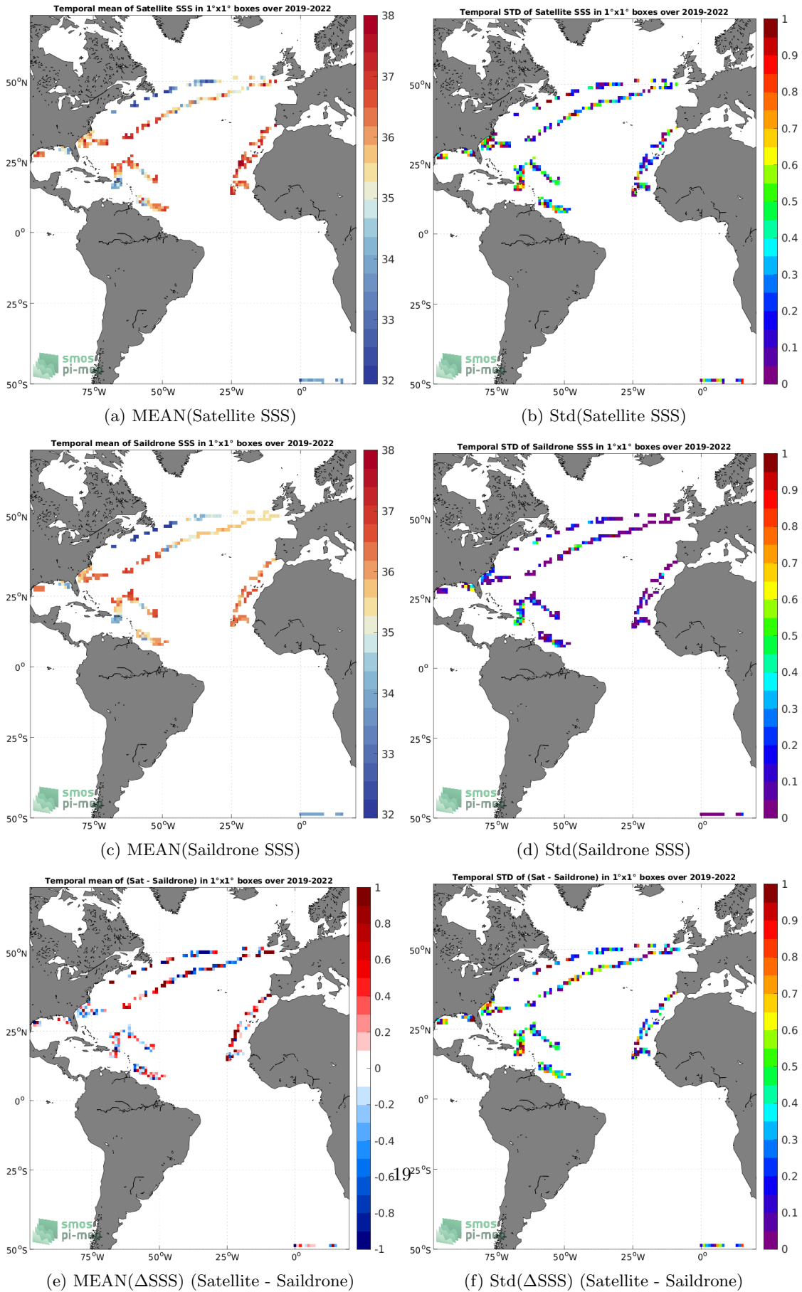
Figure 6: Temporal mean (left) and Std (right) of SSS from SMOS SSS L2 v700 (ESA) (top), Saildrone (middle), and of \Delta SSS (Satellite - Saildrone). Only match-up pairs are used to generate these maps.
