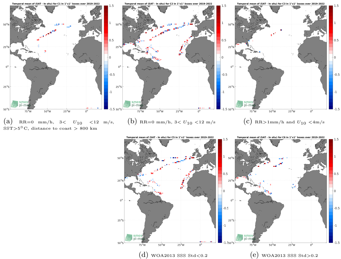
Figure 12: Temporal mean gridded over spatial boxes of size 1^\circ \times 1^\circ of \Delta SSS (SMOS SSS L2 v700 (ESA) - Sairdrone) for 5 different subdatasets corresponding to:RR=0 mm/h, 3 < U_{10} < 12 m/s, SST >5^\circ\text{C} , distance to coast > 800 km (a), RR=0 mm/h, 3 < U_{10} < 12 m/s (b), RR >1 mm/h and U_{10} < 4 m/s (c), WOA2013 SSS Std <0.2 (d), WOA2013 SSS Std >0.2 (e).
