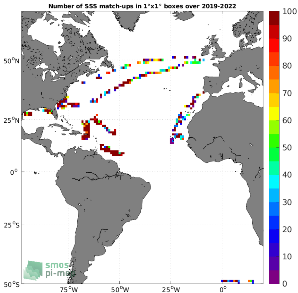
Figure 4: Number of SSS match-ups between Saildrone SSS and the SMOS SSS L2 v700 (ESA) SSS product for the Atlantic Ocean Pi-MEP region over 1°×1° boxes and for the full satellite product period.
