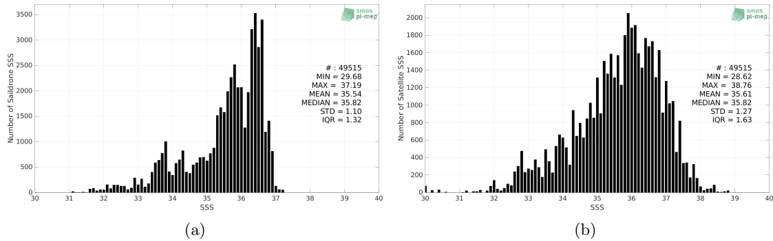
Figure 2: Histograms of SSS from Sairdrone (a) and SMOS SSS L2 v700 (ESA) (b) considering all match-up pairs per bins of 0.1 over the Atlantic Ocean Pi-MEP region and for the full satellite product period.
