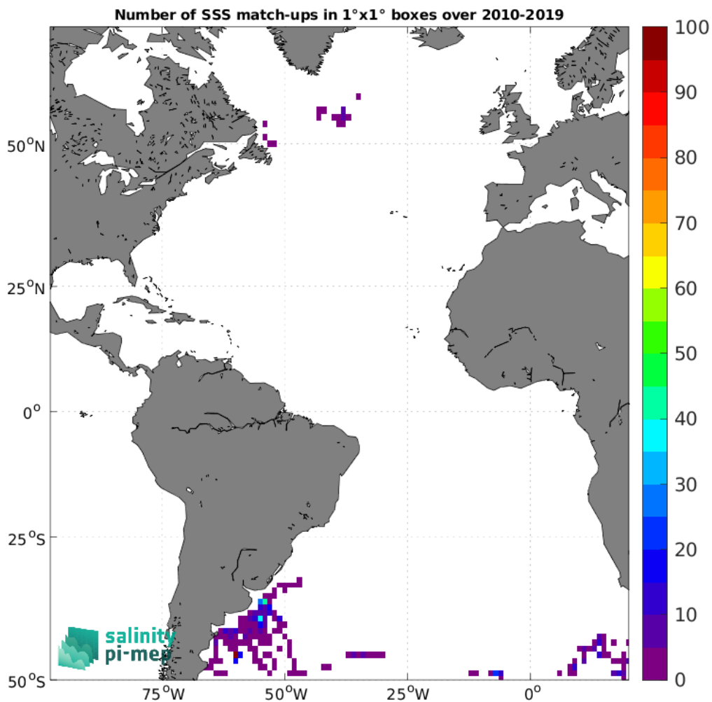
Figure 4: Number of SSS match-ups between Marine mammals SSS and the SMOS SSS L2 v700 (ESA) SSS product for the Atlantic Ocean Pi-MEP region over 1^{\circ} \times 1^{\circ} boxes and for the full satellite product period.
