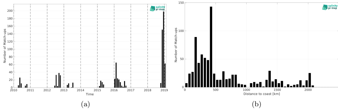
Figure 1: Number of match-ups between Marine mammals and SMOS SSS L2 v700 (ESA) SSS as a function of time (a) and as function of the distance to coast (b) over the Atlantic Ocean Pi-MEP region and for the full satellite product period.
