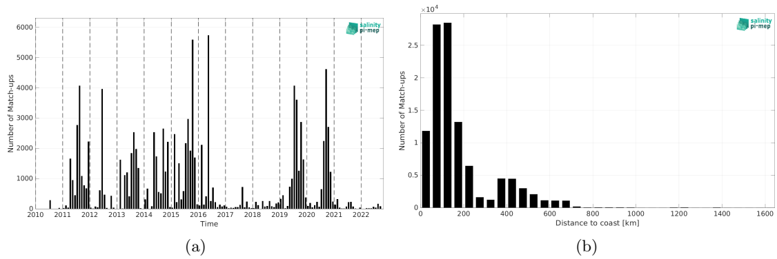
Figure 1: Number of match-ups between ICES and SMOS SSS L2 v700 (ESA) SSS as a function of time (a) and as function of the distance to coast (b) over the Atlantic Ocean Pi-MEP region and for the full satellite product period.
