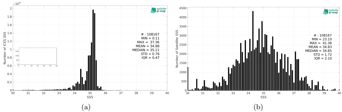
Figure 2: Histograms of SSS from ICES (a) and SMOS SSS L2 v700 (ESA) (b) considering all match-up pairs per bins of 0.1 over the Atlantic Ocean Pi-MEP region and for the full satellite product period.
