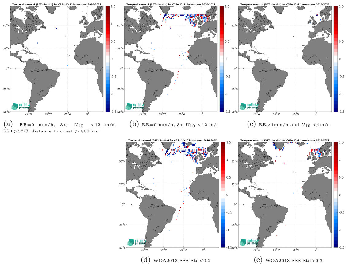
Figure 12: Temporal mean gridded over spatial boxes of size 1^\circ \times 1^\circ of \Delta\text{SSS} (SMOS SSS L2 v700 (ESA) - ICES) for 5 different subdatasets corresponding to:RR=0 mm/h, 3 < U_{10} < 12 m/s, SST >5^\circ\text{C} , distance to coast > 800 km (a), RR=0 mm/h, 3 < U_{10} < 12 m/s (b), RR >1 mm/h and U_{10} < 4 m/s (c), WOA2013 SSS Std <0.2 (d), WOA2013 SSS Std >0.2 (e).
