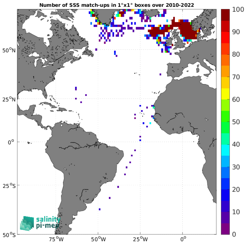
Figure 4: Number of SSS match-ups between ICES SSS and the SMOS SSS L2 v700 (ESA) SSS product for the Atlantic Ocean Pi-MEP region over 1^\circ \times 1^\circ boxes and for the full satellite product period.
