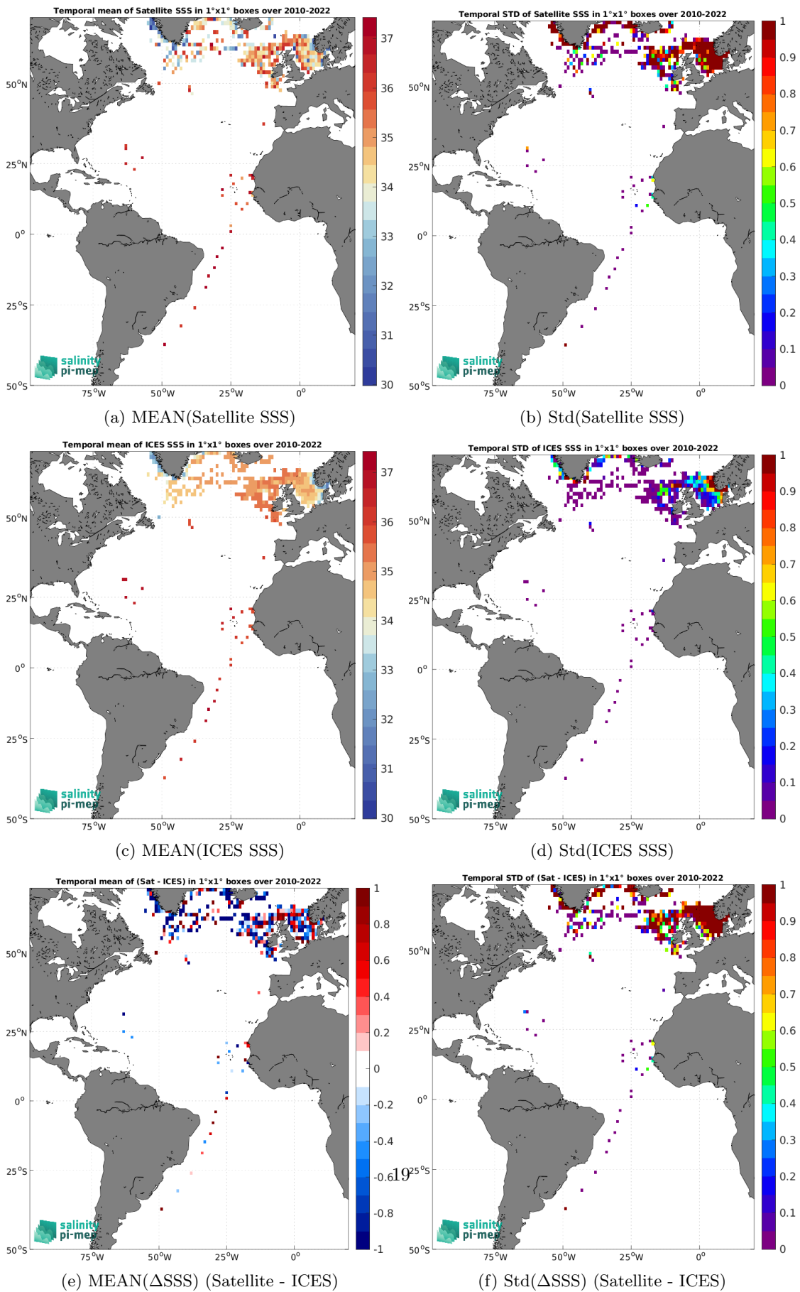
Figure 6: Temporal mean (left) and Std (right) of SSS from SMOS SSS L2 v700 (ESA) (top), ICES (middle), and of \Delta SSS (Satellite - ICES). Only match-up pairs are used to generate these maps.
