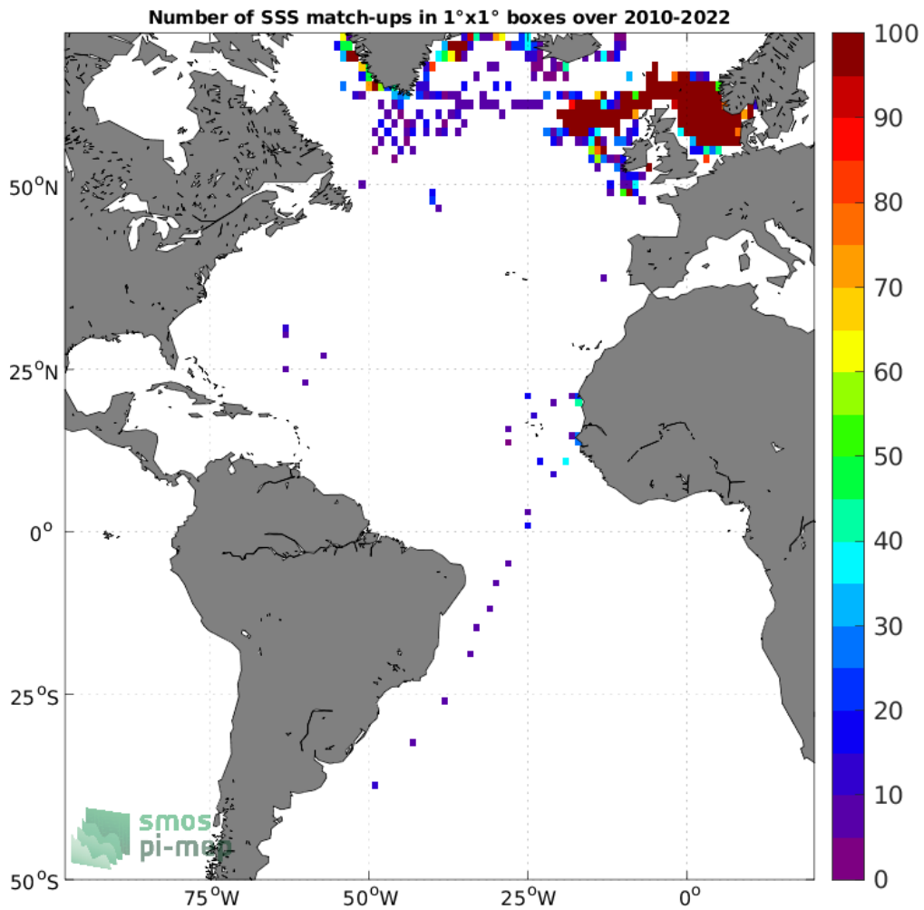
Figure 4: Number of SSS match-ups between ICES SSS and the SMOS SSS L2 v700 (ESA) SSS product for the Atlantic Ocean Pi-MEP region over 1°x1° boxes and for the full satellite product period.
