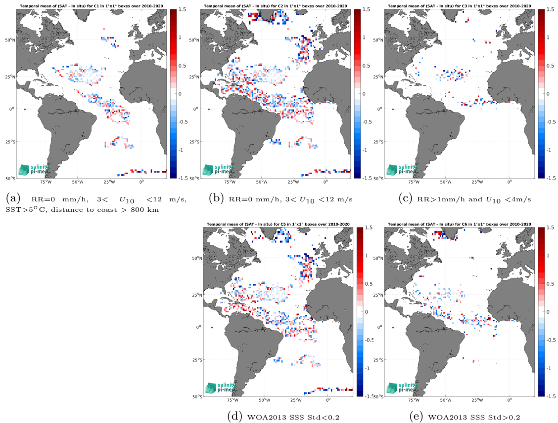
Figure 13: Temporal mean gridded over spatial boxes of size 1^\circ \times 1^\circ of \Delta SSS (SMOS SSS L2 v700 (ESA) - Surface drifters) for 5 different subdatasets corresponding to:RR=0 mm/h, 3 < U_{10} < 12 m/s, SST >5^\circ\text{C} , distance to coast > 800 km (a), RR=0 mm/h, 3 < U_{10} < 12 m/s (b), RR >1 mm/h and U_{10} < 4 m/s (c), WOA2013 SSS Std <0.2 (d), WOA2013 SSS Std >0.2 (e).
