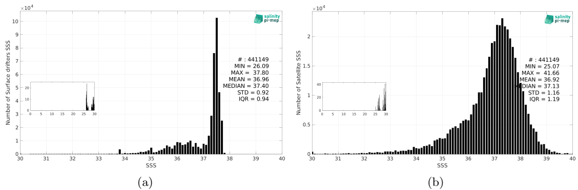
Figure 3: Histograms of SSS from Surface drifters (a) and SMOS SSS L2 v700 (ESA) (b) considering all match-up pairs per bins of 0.1 over the Atlantic Ocean Pi-MEP region and for the full satellite product period.
