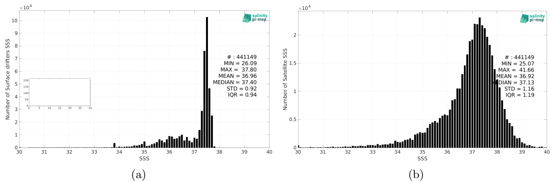
Figure 2: Histograms of SSS from Surface drifters (a) and SMOS SSS L2 v700 (ESA) (b) considering all match-up pairs per bins of 0.1 over the Atlantic Ocean Pi-MEP region and for the full satellite product period.
