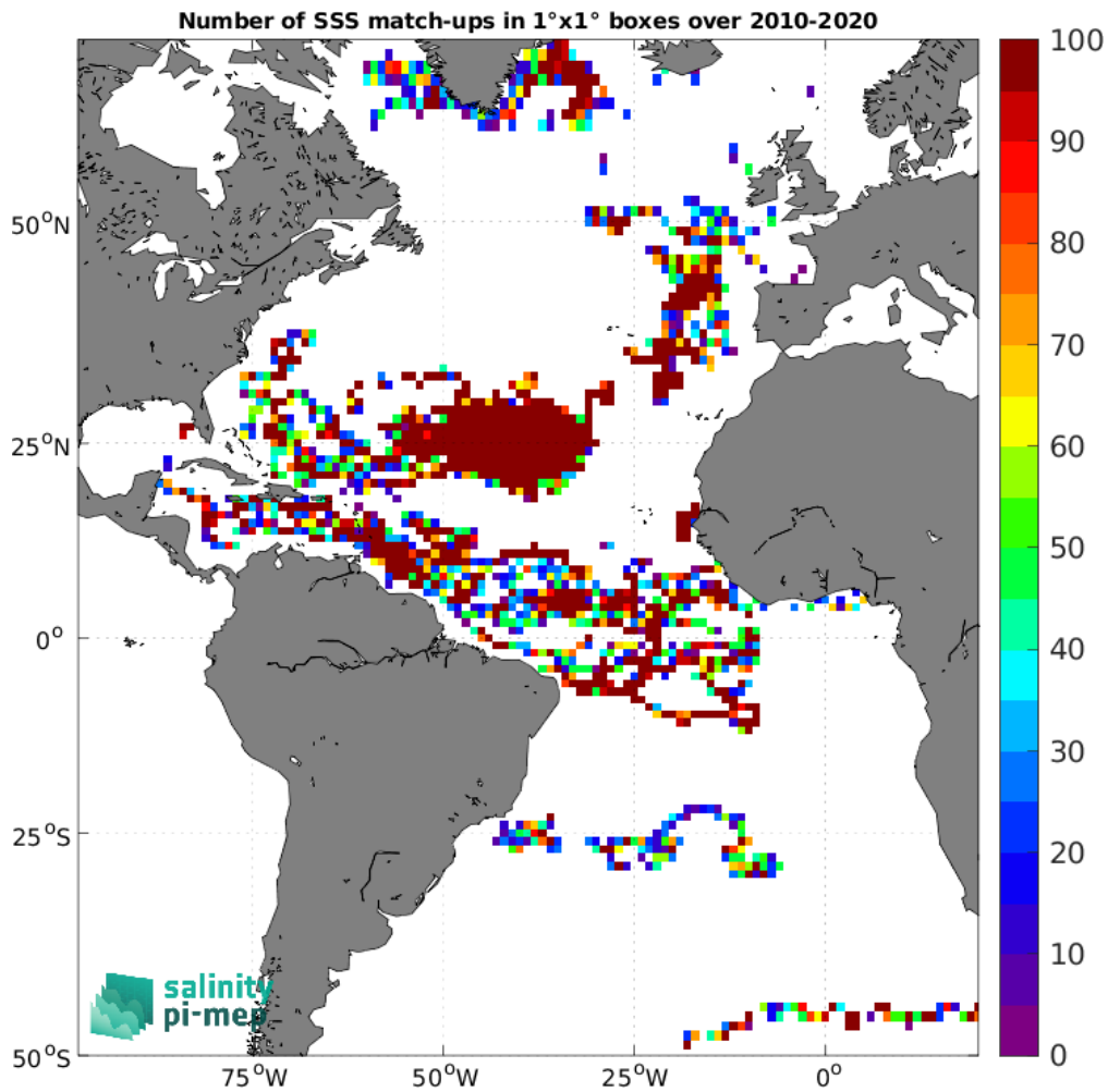
Figure 3: Number of SSS match-ups between Surface drifters SSS and the SMOS SSS L2 v700 (ESA) SSS product for the Atlantic Ocean Pi-MEP region over 1°×1° boxes and for the full satellite product period.
