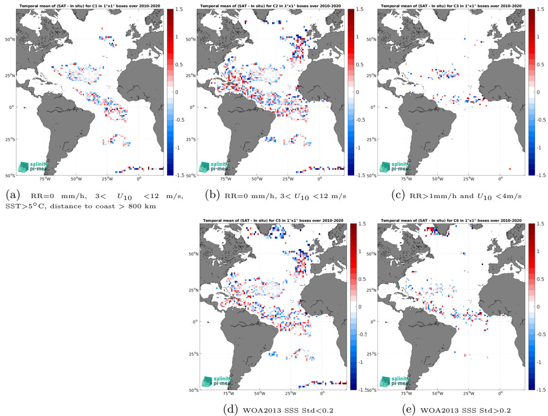
Figure 11: Temporal mean gridded over spatial boxes of size 1^\circ \times 1^\circ of \Delta SSS (SMOS SSS L2 v700 (ESA) - Surface drifters) for 5 different subdatasets corresponding to:RR=0 mm/h, 3 < U_{10} < 12 m/s, SST >5^\circ\text{C} , distance to coast > 800 km (a), RR=0 mm/h, 3 < U_{10} < 12 m/s (b), RR >1 mm/h and U_{10} < 4 m/s (c), WOA2013 SSS Std <0.2 (d), WOA2013 SSS Std >0.2 (e).
