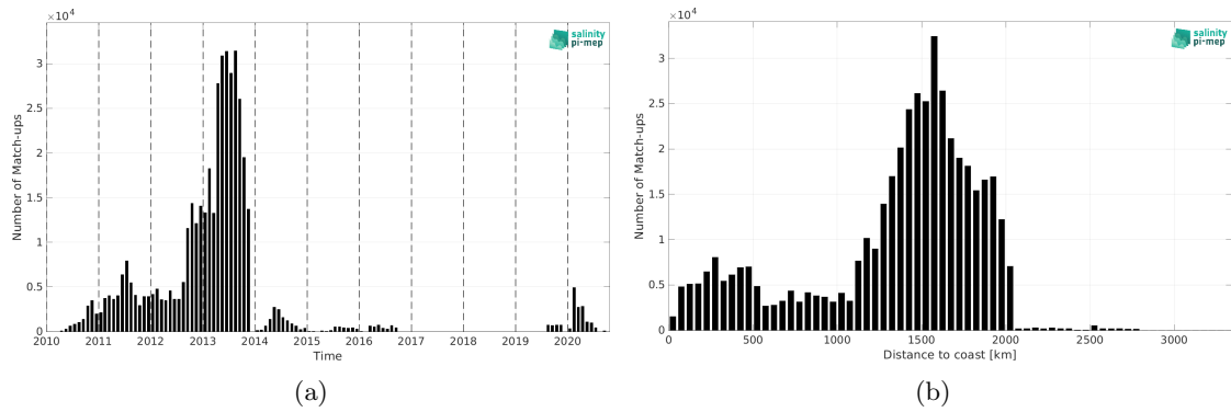
Figure 1: Number of match-ups between Surface drifters and SMOS SSS L2 v700 (ESA) SSS as a function of time (a) and as function of the distance to coast (b) over the Atlantic Ocean Pi-MEP region and for the full satellite product period.
