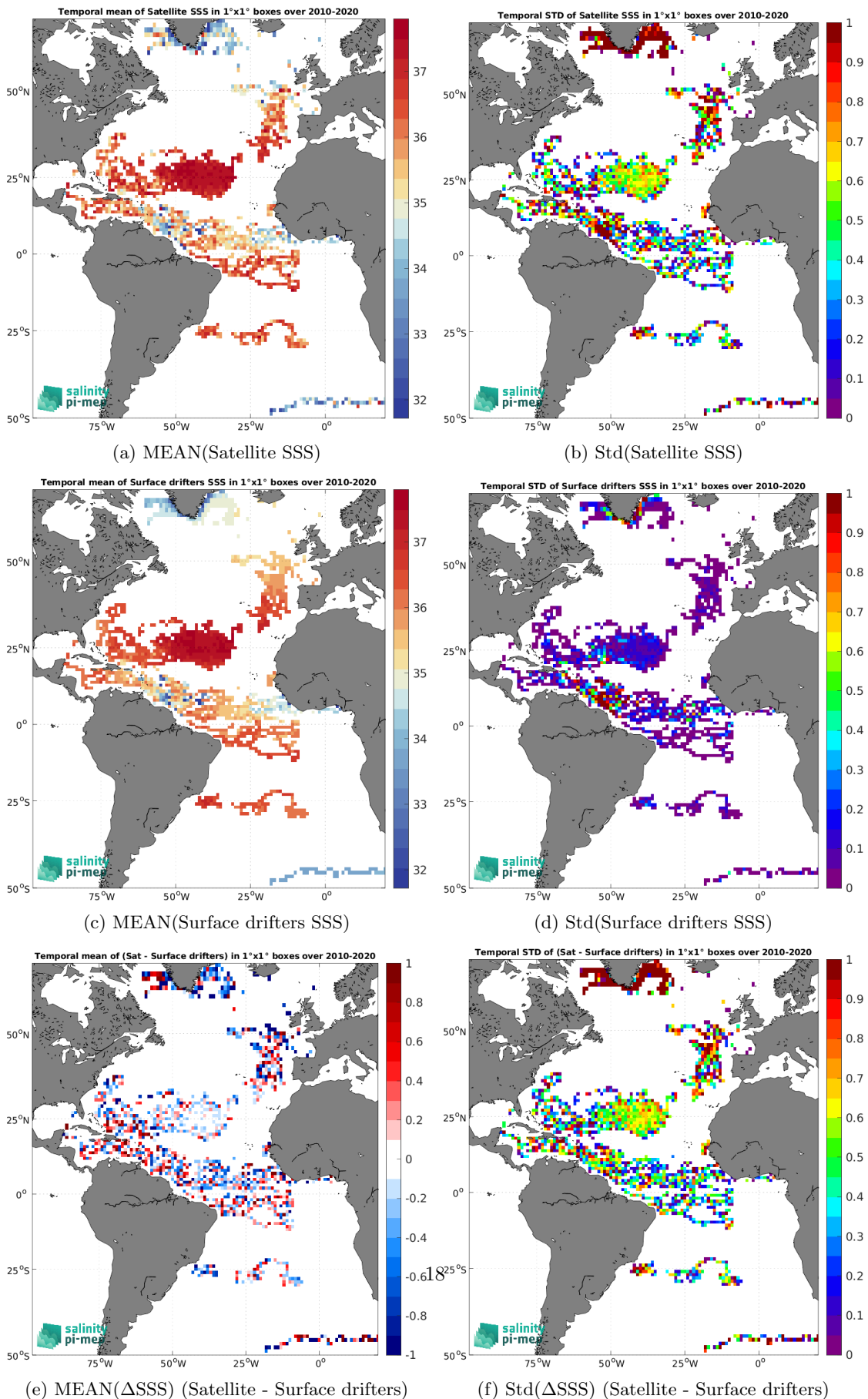
Figure 5: Temporal mean (left) and Std (right) of SSS from SMOS SSS L2 v700 (ESA) (top), Surface drifters (middle), and of \Delta SSS (Satellite - Surface drifters). Only match-up pairs are used to generate these maps.
