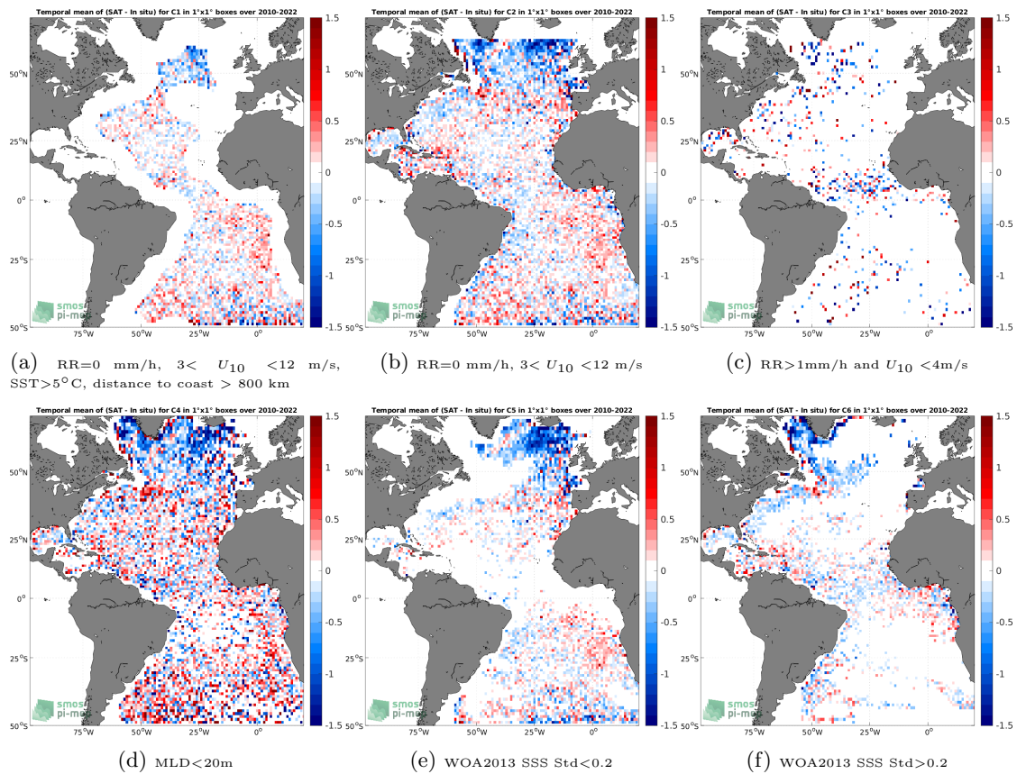
Figure 12: Temporal mean gridded over spatial boxes of size 1^\circ \times 1^\circ of \Delta SSS (SMOS SSS L2 v700 (ESA) - Argo) for 6 different subdatasets corresponding to:RR=0 mm/h, 3 < U_{10} < 12 m/s, SST > 5^\circ\text{C} , distance to coast > 800 km (a), RR=0 mm/h, 3 < U_{10} < 12 m/s (b), RR > 1 mm/h and U_{10} < 4 m/s (c),MLD < 20 m (d),WOA2013 SSS Std < 0.2 (e),WOA2013 SSS Std > 0.2 (f).
