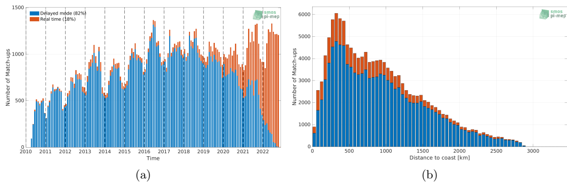
Figure 1: Number of match-ups between Argo and SMOS SSS L2 v700 (ESA) SSS as a function of time (a) and as function of the distance to coast (b) over the Atlantic Ocean Pi-MEP region and for the full satellite product period.
