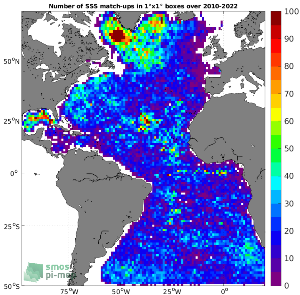
Figure 4: Number of SSS match-ups between Argo SSS and the SMOS SSS L2 v700 (ESA) SSS product for the Atlantic Ocean Pi-MEP region over 1°×1° boxes and for the full satellite product period.
