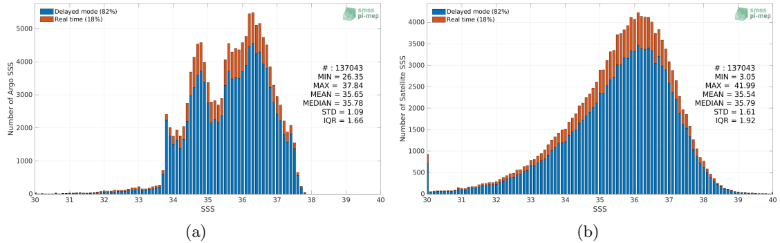
Figure 2: Histograms of SSS from Argo (a) and SMOS SSS L2 v700 (ESA) (b) considering all match-up pairs per bins of 0.1 over the Atlantic Ocean Pi-MEP region and for the full satellite product period.
