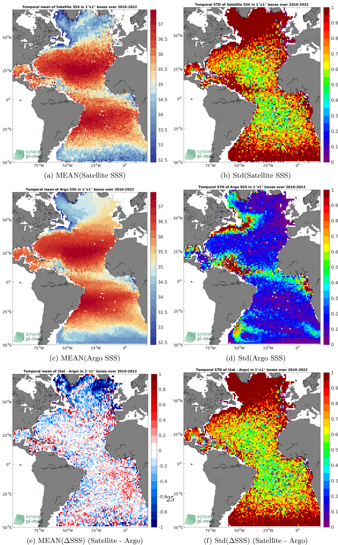
Figure 6: Temporal mean (left) and Std (right) of SSS from SMOS SSS L2 v700 (ESA) (top), Argo (middle), and of \Delta SSS (Satellite - Argo). Only match-up pairs are used to generate these maps.
