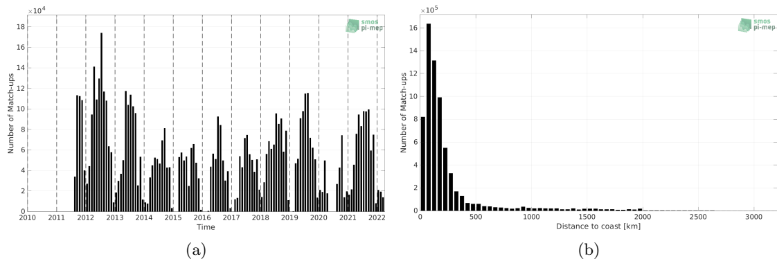
Figure 1: Number of match-ups between TSG (SAMOS) and SMAP SSS L4 OI v1 - 7 Days (IPRC) SSS as a function of time (a) and as function of the distance to coast (b) over the Atlantic Ocean Pi-MEP region and for the full satellite product period.
