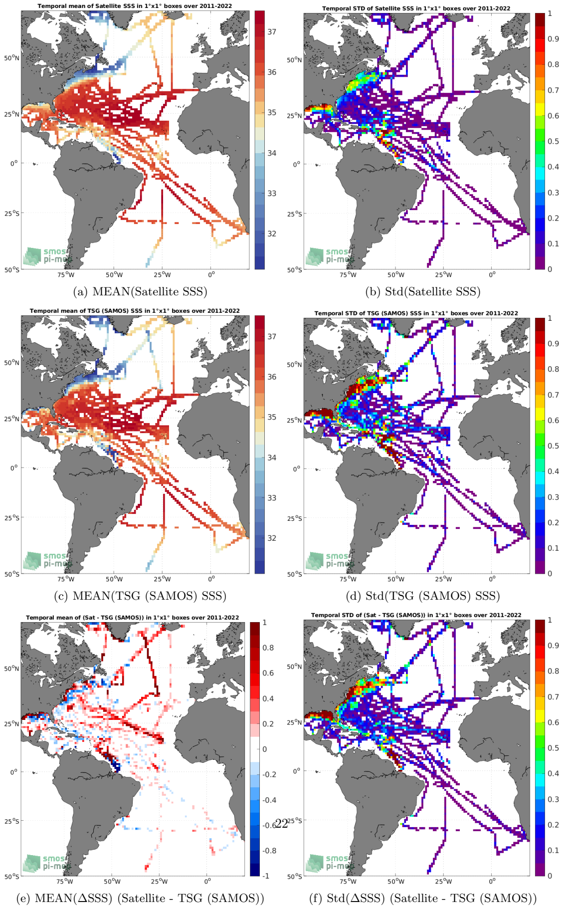
Figure 6: Temporal mean (left) and Std (right) of SSS from SMAP SSS L4 OI v1 - 7 Days (IPRC) (top), TSG (SAMOS) (middle), and of \Delta SSS (Satellite - TSG (SAMOS)). Only match-up pairs are used to generate these maps.
