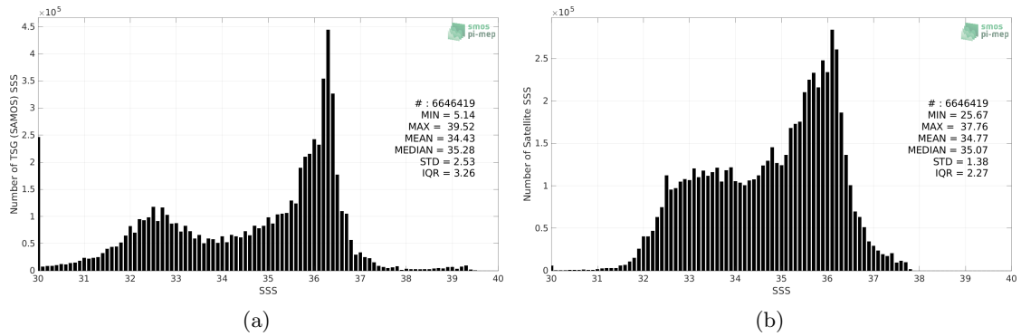
Figure 2: Histograms of SSS from TSG (SAMOS) (a) and SMAP SSS L4 OI v1 - 7 Days (IPRC) (b) considering all match-up pairs per bins of 0.1 over the Atlantic Ocean Pi-MEP region and for the full satellite product period.
