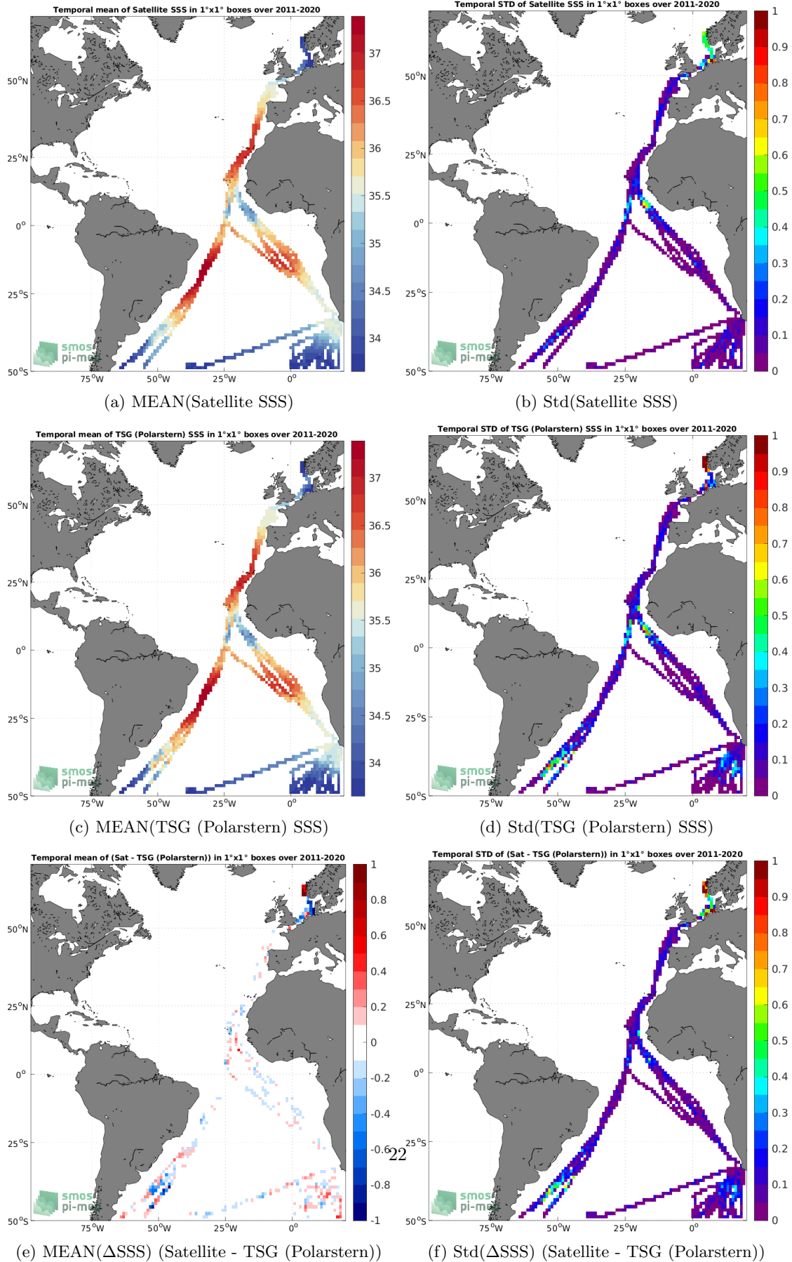
Figure 6: Temporal mean (left) and Std (right) of SSS from SMAP SSS L4 OI v1 - 7 Days (IPRC) (top), TSG (Polarstern) (middle), and of \Delta SSS (Satellite - TSG (Polarstern)). Only match-up pairs are used to generate these maps.
