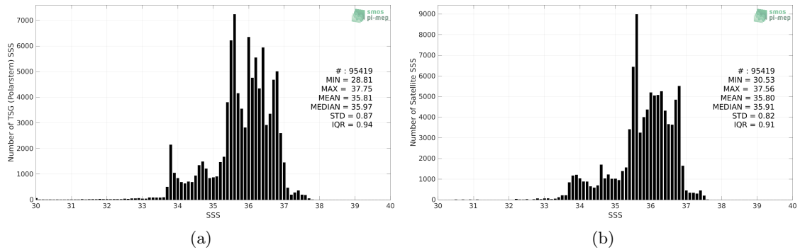
Figure 2: Histograms of SSS from TSG (Polarstern) (a) and SMAP SSS L4 OI v1 - 7 Days (IPRC) (b) considering all match-up pairs per bins of 0.1 over the Atlantic Ocean Pi-MEP region and for the full satellite product period.
