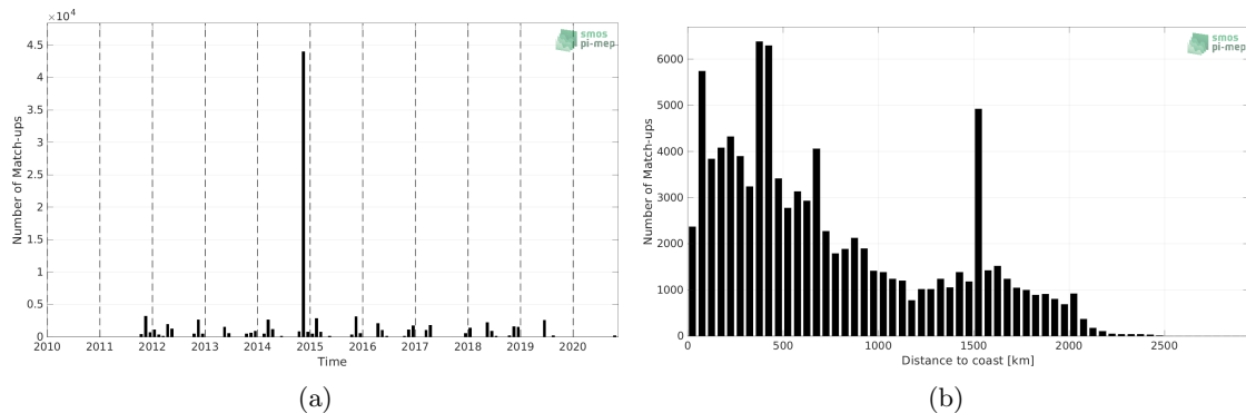
Figure 1: Number of match-ups between TSG (Polarstern) and SMAP SSS L4 OI v1 - 7 Days (IPRC) SSS as a function of time (a) and as function of the distance to coast (b) over the Atlantic Ocean Pi-MEP region and for the full satellite product period.
