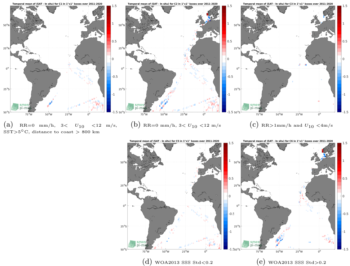
Figure 12: Temporal mean gridded over spatial boxes of size 1^\circ \times 1^\circ of \Delta SSS (SMAP SSS L4 OI v1 - 7 Days (IPRC) - TSG (Polarstern)) for 5 different subdatasets corresponding to:RR=0 mm/h, 3 < U_{10} < 12 m/s, SST >5^\circ\text{C} , distance to coast > 800 km (a), RR=0 mm/h, 3 < U_{10} < 12 m/s (b), RR >1 mm/h and U_{10} < 4 m/s (c), WOA2013 SSS Std <0.2 (d), WOA2013 SSS Std >0.2 (e).
