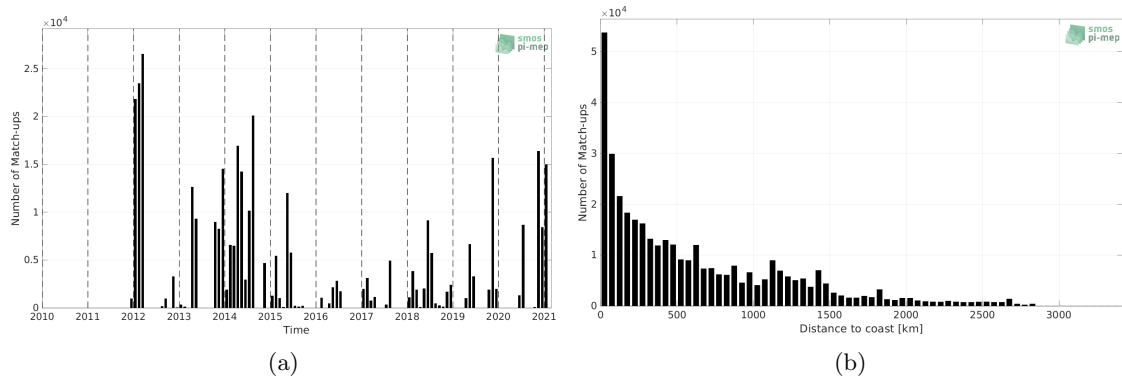
Figure 1: Number of match-ups between TSG (GOSUD-Sailing-ship) and SMAP SSS L4 OI v1 - 7 Days (IPRC) SSS as a function of time (a) and as function of the distance to coast (b) over the Atlantic Ocean Pi-MEP region and for the full satellite product period.
