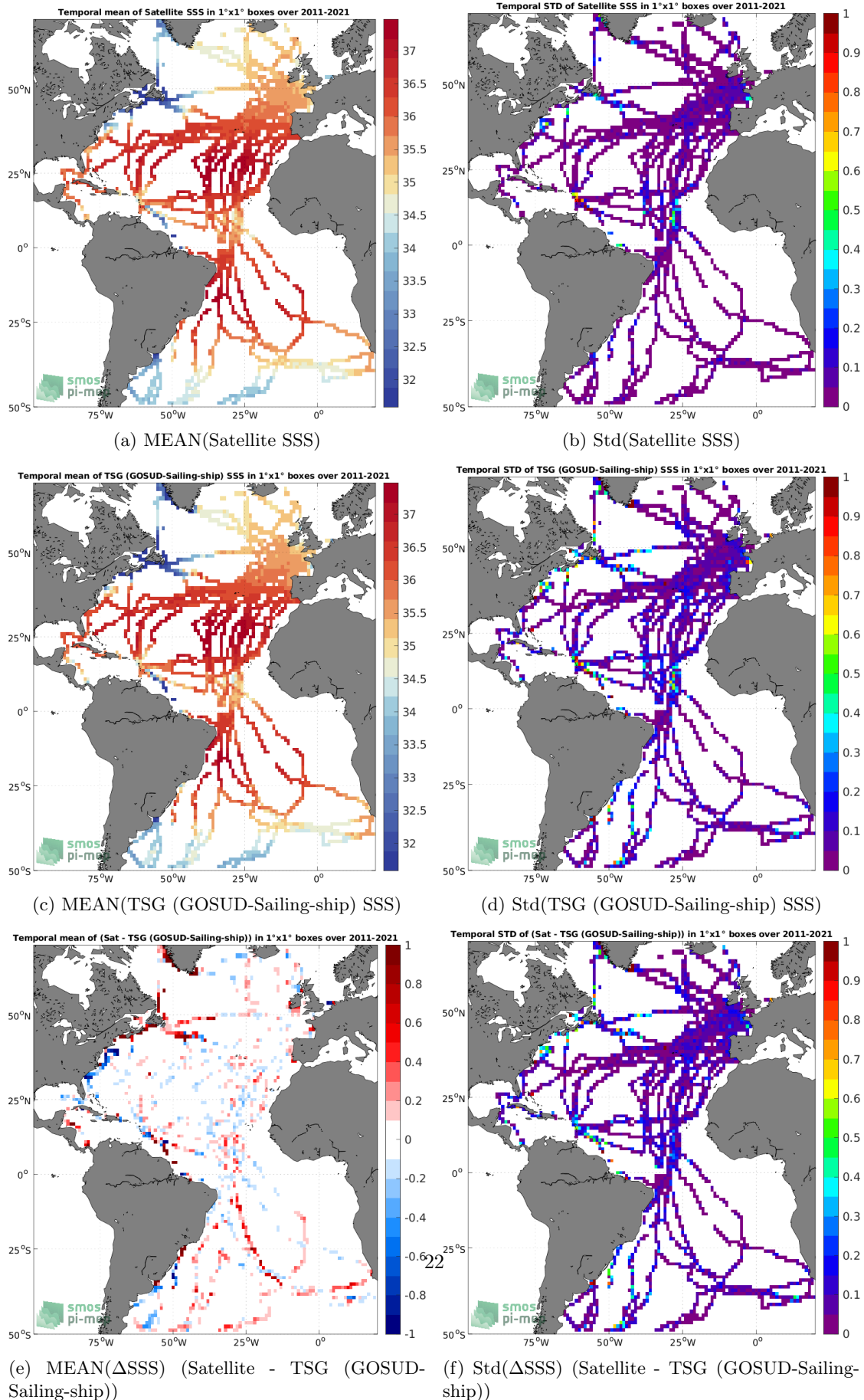
Figure 6: Temporal mean (left) and Std (right) of SSS from SMAP SSS L4 OI v1 - 7 Days (IPRC) (top), TSG (GOSUD-Sailing-ship) (middle), and of \Delta SSS (Satellite - TSG (GOSUD-Sailing-ship)). Only match-up pairs are used to generate these maps.
