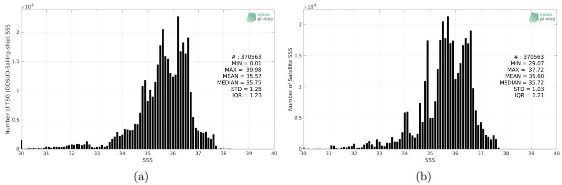
Figure 2: Histograms of SSS from TSG (GOSUD-Sailing-ship) (a) and SMAP SSS L4 OI v1 - 7 Days (IPRC) (b) considering all match-up pairs per bins of 0.1 over the Atlantic Ocean Pi-MEP region and for the full satellite product period.
