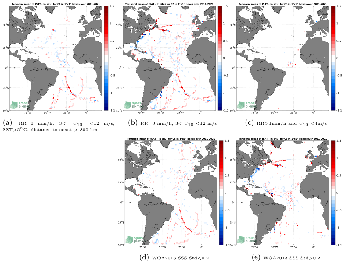
Figure 12: Temporal mean gridded over spatial boxes of size 1^\circ \times 1^\circ of \Delta SSS (SMAP SSS L4 OI v1 - 7 Days (IPRC) - TSG (GOSUD-Sailing-ship)) for 5 different subdatasets corresponding to:RR=0 mm/h, 3 < U_{10} < 12 m/s, SST>5°C, distance to coast > 800 km (a), RR=0 mm/h, 3 < U_{10} < 12 m/s (b), RR>1mm/h and U_{10} < 4 m/s (c), WOA2013 SSS Std<0.2 (d), WOA2013 SSS Std>0.2 (e).
