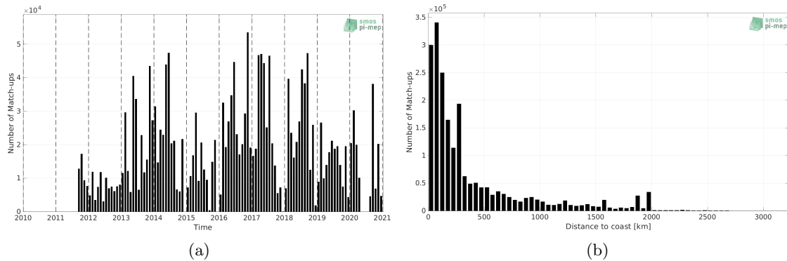
Figure 1: Number of match-ups between TSG (GOSUD-Research-vessel) and SMAP SSS L4 OI v1 - 7 Days (IPRC) SSS as a function of time (a) and as function of the distance to coast (b) over the Atlantic Ocean Pi-MEP region and for the full satellite product period.
