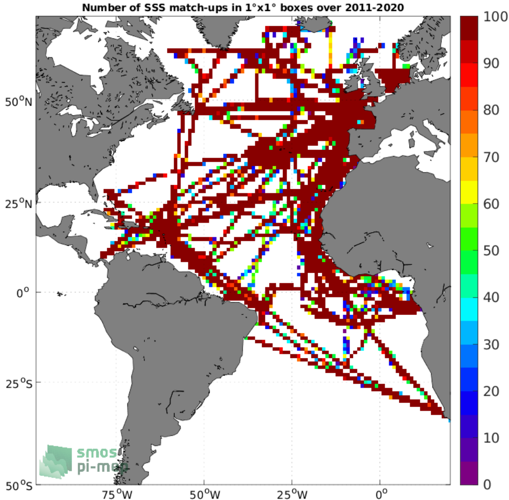
Figure 4: Number of SSS match-ups between TSG (GOSUD-Research-vessel) SSS and the SMAP SSS L4 OI v1 - 7 Days (IPRC) SSS product for the Atlantic Ocean Pi-MEP region over 1^\circ \times 1^\circ boxes and for the full satellite product period.
