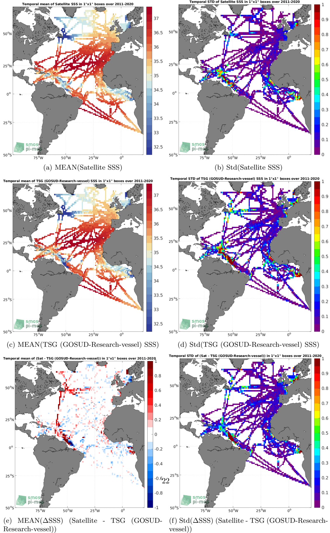
Figure 6: Temporal mean (left) and Std (right) of SSS from SMAP SSS L4 OI v1 - 7 Days (IPRC) (top), TSG (GOSUD-Research-vessel) (middle), and of \Delta SSS (Satellite - TSG (GOSUD-Research-vessel)). Only match-up pairs are used to generate these maps.
