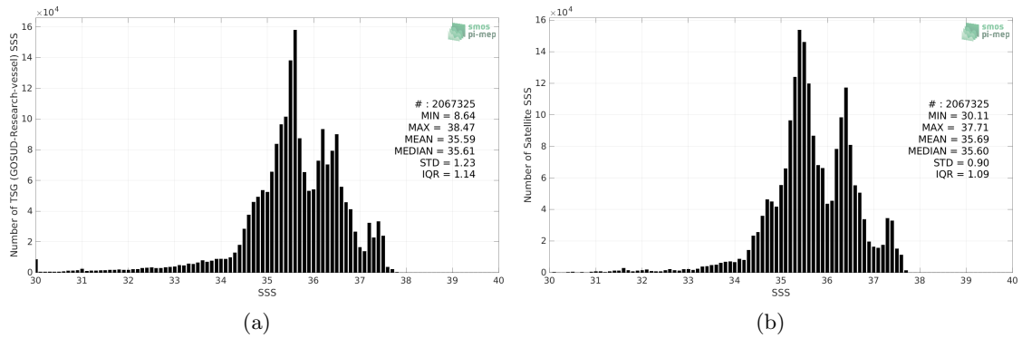
Figure 2: Histograms of SSS from TSG (GOSUD-Research-vessel) (a) and SMAP SSS L4 OI v1 - 7 Days (IPRC) (b) considering all match-up pairs per bins of 0.1 over the Atlantic Ocean Pi-MEP region and for the full satellite product period.
