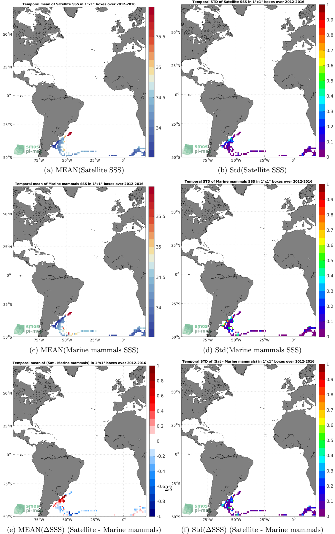
Figure 6: Temporal mean (left) and Std (right) of SSS from SMAP SSS L4 OI v1 - 7 Days (IPRC) (top), Marine mammals (middle), and of \Delta SSS (Satellite - Marine mammals). Only match-up pairs are used to generate these maps.
