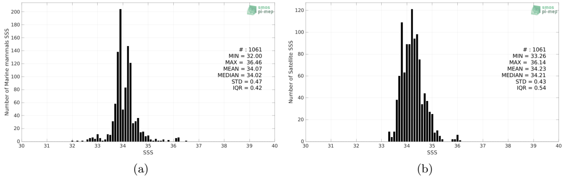
Figure 2: Histograms of SSS from Marine mammals (a) and SMAP SSS L4 OI v1 - 7 Days (IPRC) (b) considering all match-up pairs per bins of 0.1 over the Atlantic Ocean Pi-MEP region and for the full satellite product period.
