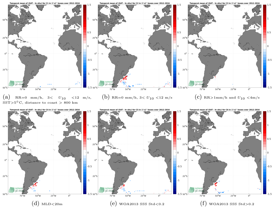
Figure 12: Temporal mean gridded over spatial boxes of size 1^\circ \times 1^\circ of \Delta SSS (SMAP SSS L4 OI v1 - 7 Days (IPRC) - Marine mammals) for 6 different subdatasets corresponding to:RR=0 mm/h, 3 < U_{10} < 12 m/s, SST >5^\circ C, distance to coast > 800 km (a), RR=0 mm/h, 3 < U_{10} < 12 m/s (b), RR >1 mm/h and U_{10} < 4 m/s (c),MLD <20 m (d),WOA2013 SSS Std <0.2 (e),WOA2013 SSS Std >0.2 (f).
