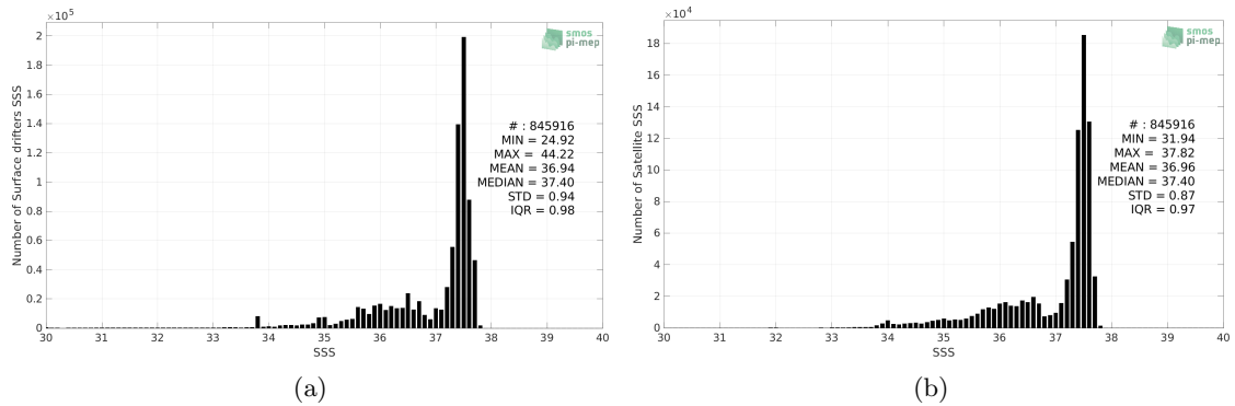
Figure 2: Histograms of SSS from Surface drifters (a) and SMAP SSS L4 OI v1 - 7 Days (IPRC) (b) considering all match-up pairs per bins of 0.1 over the Atlantic Ocean Pi-MEP region and for the full satellite product period.
