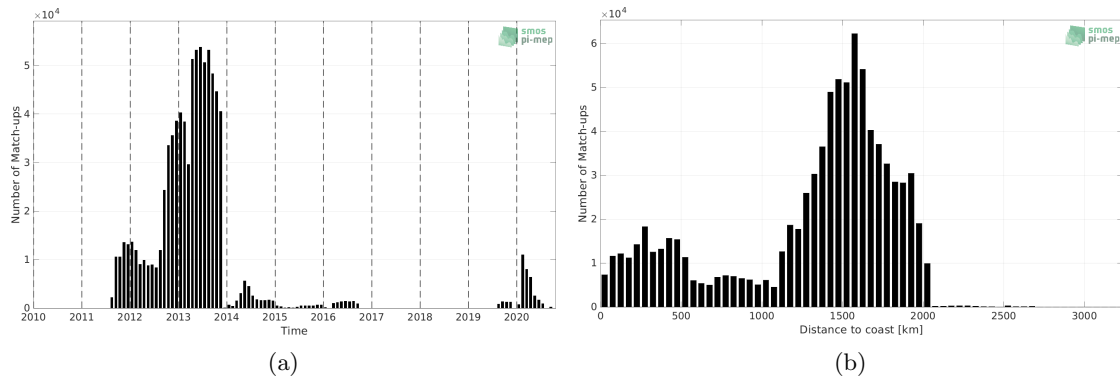
Figure 1: Number of match-ups between Surface drifters and SMAP SSS L4 OI v1 - 7 Days (IPRC) SSS as a function of time (a) and as function of the distance to coast (b) over the Atlantic Ocean Pi-MEP region and for the full satellite product period.
