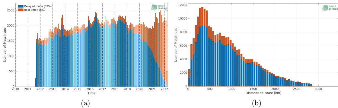
Figure 1: Number of match-ups between Argo and SMAP SSS L4 OI v1 - 7 Days (IPRC) SSS as a function of time (a) and as function of the distance to coast (b) over the Atlantic Ocean Pi-MEP region and for the full satellite product period.
