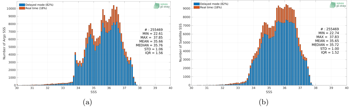
Figure 2: Histograms of SSS from Argo (a) and SMAP SSS L4 OI v1 - 7 Days (IPRC) (b) considering all match-up pairs per bins of 0.1 over the Atlantic Ocean Pi-MEP region and for the full satellite product period.
