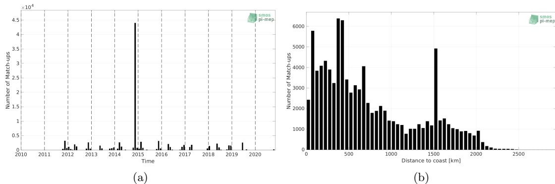
Figure 1: Number of match-ups between TSG (Polarstern) and SMAP SSS L4 OI v1 - Monthly (IPRC) SSS as a function of time (a) and as function of the distance to coast (b) over the Atlantic Ocean Pi-MEP region and for the full satellite product period.
