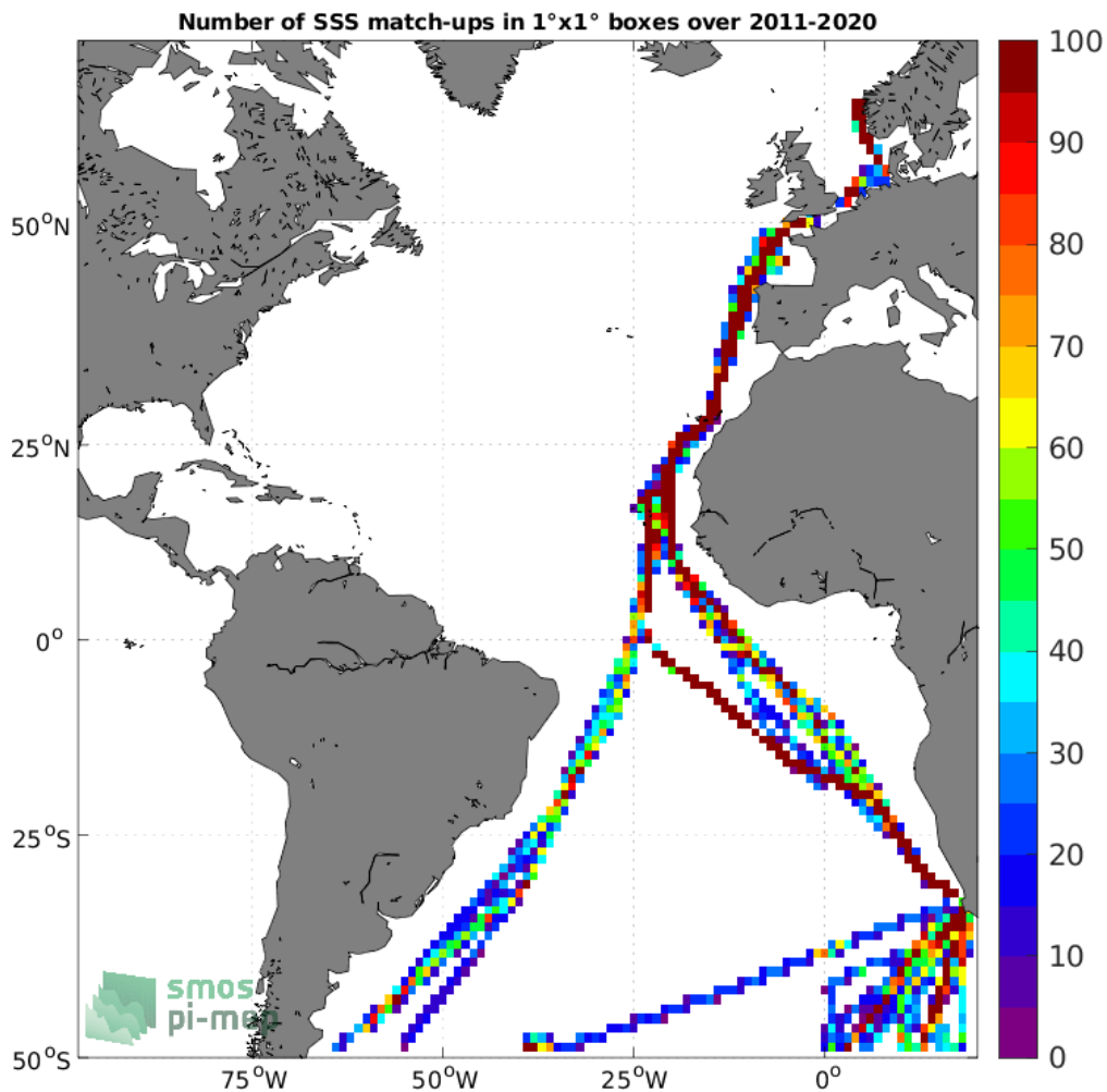
Figure 4: Number of SSS match-ups between TSG (Polarstern) SSS and the SMAP SSS L4 OI v1 - Monthly (IPRC) SSS product for the Atlantic Ocean Pi-MEP region over 1^\circ \times 1^\circ boxes and for the full satellite product period.
