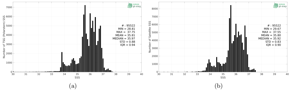
Figure 2: Histograms of SSS from TSG (Polarstern) (a) and SMAP SSS L4 OI v1 - Monthly (IPRC) (b) considering all match-up pairs per bins of 0.1 over the Atlantic Ocean Pi-MEP region and for the full satellite product period.
