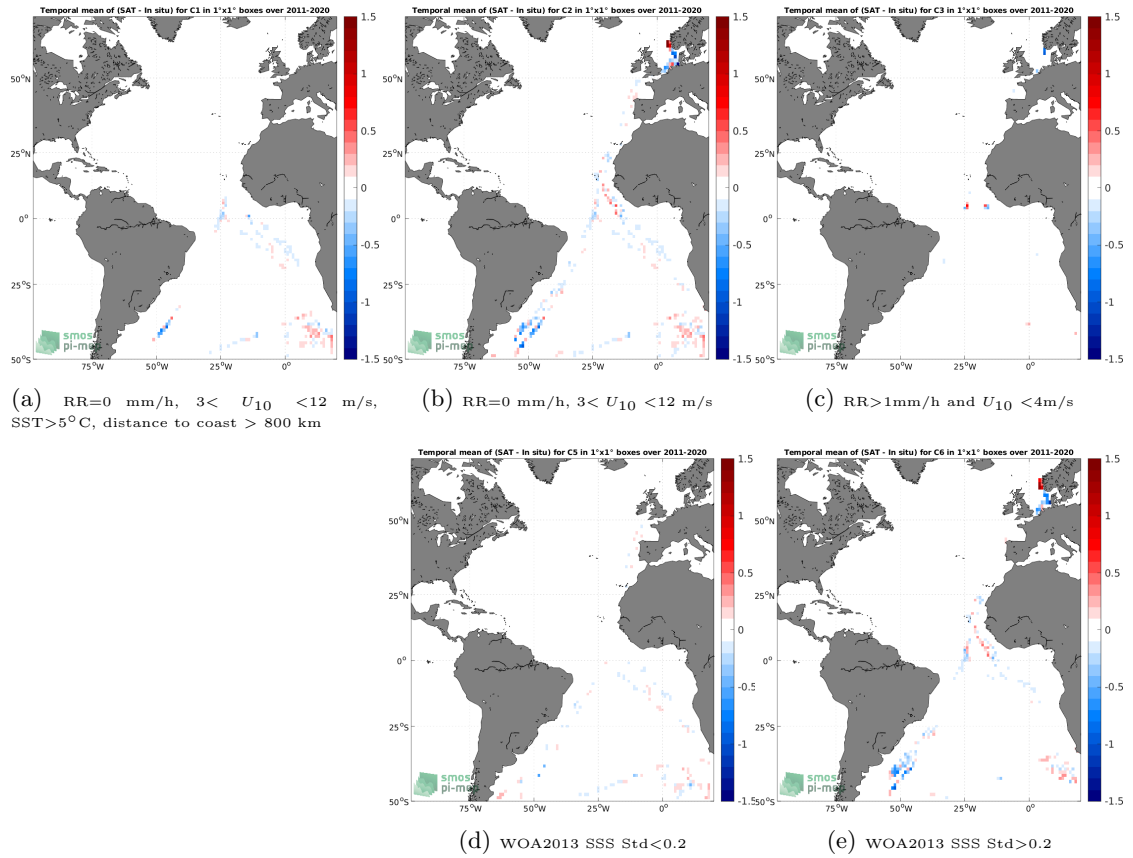
Figure 12: Temporal mean gridded over spatial boxes of size 1^\circ \times 1^\circ of \Delta SSS (SMAP SSS L4 OI v1 - Monthly (IPRC) - TSG (Polarstern)) for 5 different subdatasets corresponding to:RR=0 mm/h, 3 < U_{10} < 12 m/s, SST >5^\circ\text{C} , distance to coast > 800 km (a), RR=0 mm/h, 3 < U_{10} < 12 m/s (b), RR >1 mm/h and U_{10} < 4 m/s (c), WOA2013 SSS Std <0.2 (d), WOA2013 SSS Std >0.2 (e).
