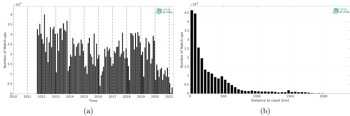
Figure 1: Number of match-ups between TSG (LEGOS-DM) and SMAP SSS L4 OI v1 - Monthly (IPRC) SSS as a function of time (a) and as function of the distance to coast (b) over the Atlantic Ocean Pi-MEP region and for the full satellite product period.
