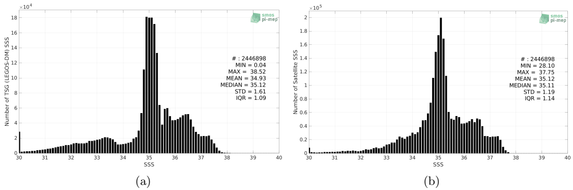
Figure 2: Histograms of SSS from TSG (LEGOS-DM) (a) and SMAP SSS L4 OI v1 - Monthly (IPRC) (b) considering all match-up pairs per bins of 0.1 over the Atlantic Ocean Pi-MEP region and for the full satellite product period.
