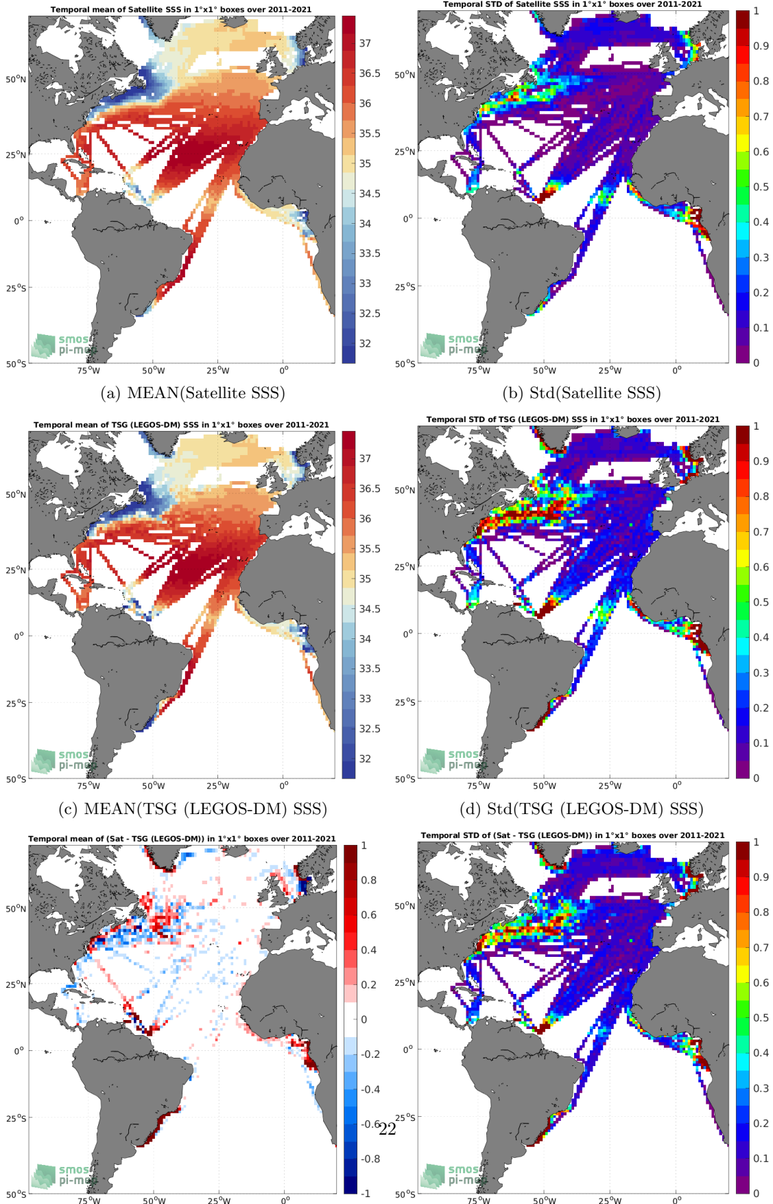
(e) MEAN( \Delta SSS) (Satellite - TSG (LEGOS-DM)) (f) Std( \Delta SSS) (Satellite - TSG (LEGOS-DM)) Figure 6: Temporal mean (left) and Std (right) of SSS from SMAP SSS L4 OI v1 - Monthly (IPRC) (top), TSG (LEGOS-DM) (middle), and of \Delta SSS (Satellite - TSG (LEGOS-DM)). Only match-up pairs are used to generate these maps.
