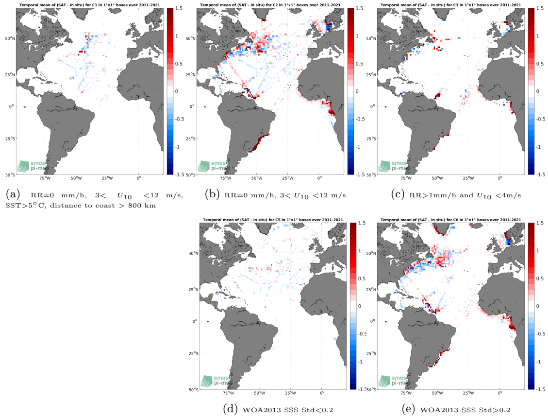
Figure 12: Temporal mean gridded over spatial boxes of size 1^\circ \times 1^\circ of \Delta SSS (SMAP SSS L4 OI v1 - Monthly (IPRC) - TSG (LEGOS-DM)) for 5 different subdatasets corresponding to:RR=0 mm/h, 3 < U_{10} < 12 m/s, SST >5^\circ\text{C} , distance to coast > 800 km (a), RR=0 mm/h, 3 < U_{10} < 12 m/s (b), RR >1 mm/h and U_{10} < 4 m/s (c), WOA2013 SSS Std <0.2 (d), WOA2013 SSS Std >0.2 (e).
