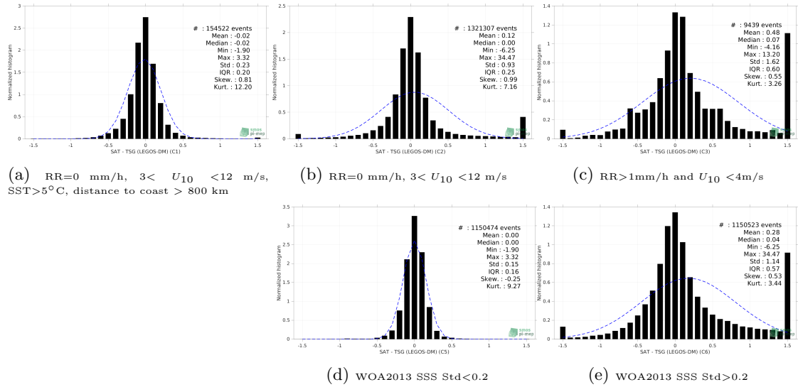
Figure 13: Normalized histogram of \Delta SSS (SMAP SSS L4 OI v1 - Monthly (IPRC) - TSG (LEGOS-DM)) for 5 different subdatasets corresponding to: RR=0 mm/h, 3 < U_{10} < 12 m/s, SST > 5°C, distance to coast > 800 km (a), RR=0 mm/h, 3 < U_{10} < 12 m/s (b), RR > 1mm/h and U_{10} < 4 m/s (c), WOA2013 SSS Std < 0.2 (d), WOA2013 SSS Std > 0.2 (e).
