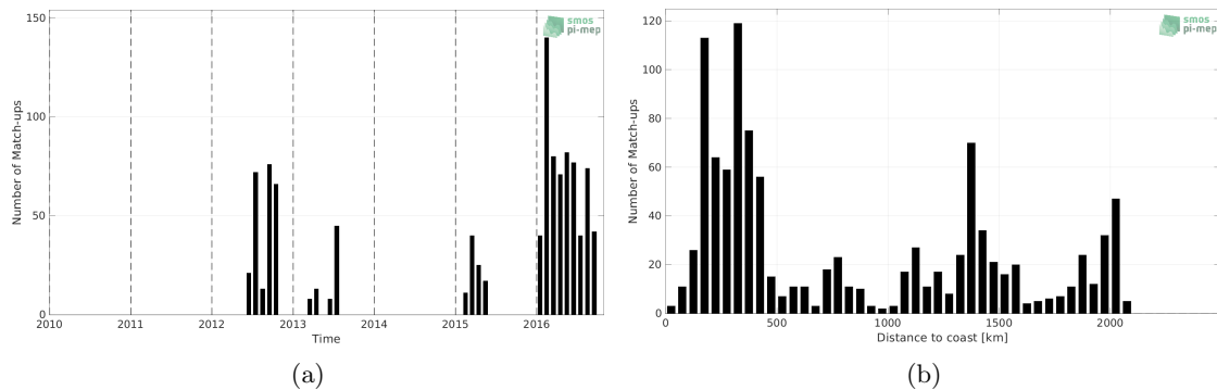
Figure 1: Number of match-ups between Marine mammals and SMAP SSS L4 OI v1 - Monthly (IPRC) SSS as a function of time (a) and as function of the distance to coast (b) over the Atlantic Ocean Pi-MEP region and for the full satellite product period.
