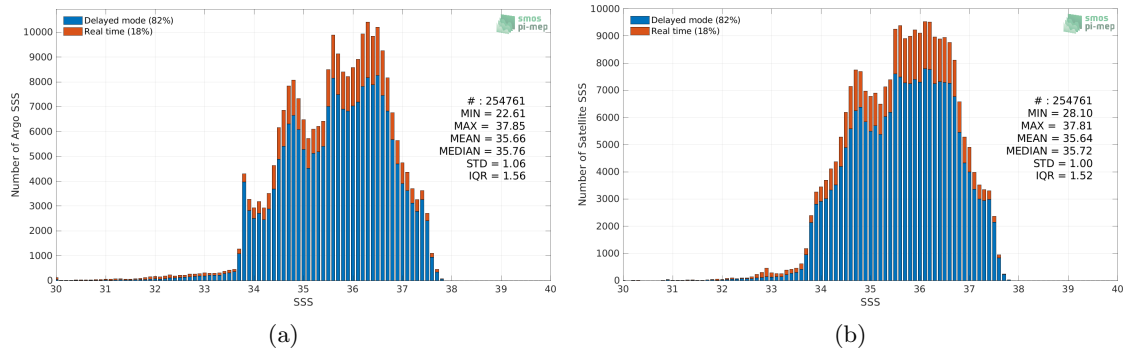
Figure 2: Histograms of SSS from Argo (a) and SMAP SSS L4 OI v1 - Monthly (IPRC) (b) considering all match-up pairs per bins of 0.1 over the Atlantic Ocean Pi-MEP region and for the full satellite product period.
