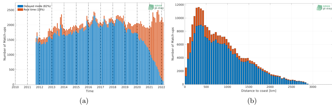
Figure 1: Number of match-ups between Argo and SMAP SSS L4 OI v1 - Monthly (IPRC) SSS as a function of time (a) and as function of the distance to coast (b) over the Atlantic Ocean Pi-MEP region and for the full satellite product period.
