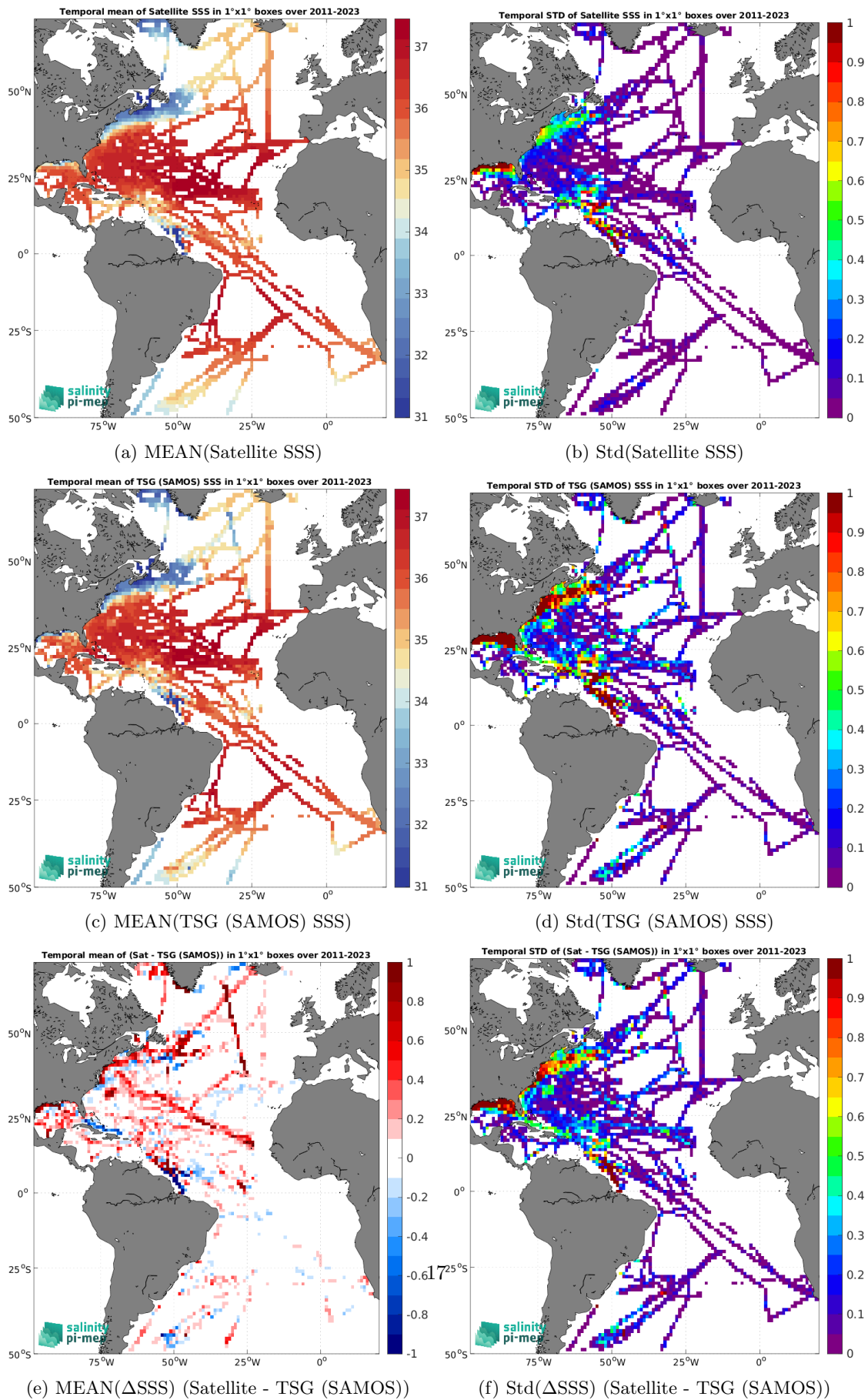
Figure 7: Temporal mean (left) and Std (right) of SSS from SMAP SSS L4 OI v3 - Monthly (ESR) (top), TSG (SAMOS) (middle), and of \Delta SSS (Satellite - TSG (SAMOS)). Only match-up pairs are used to generate these maps.
