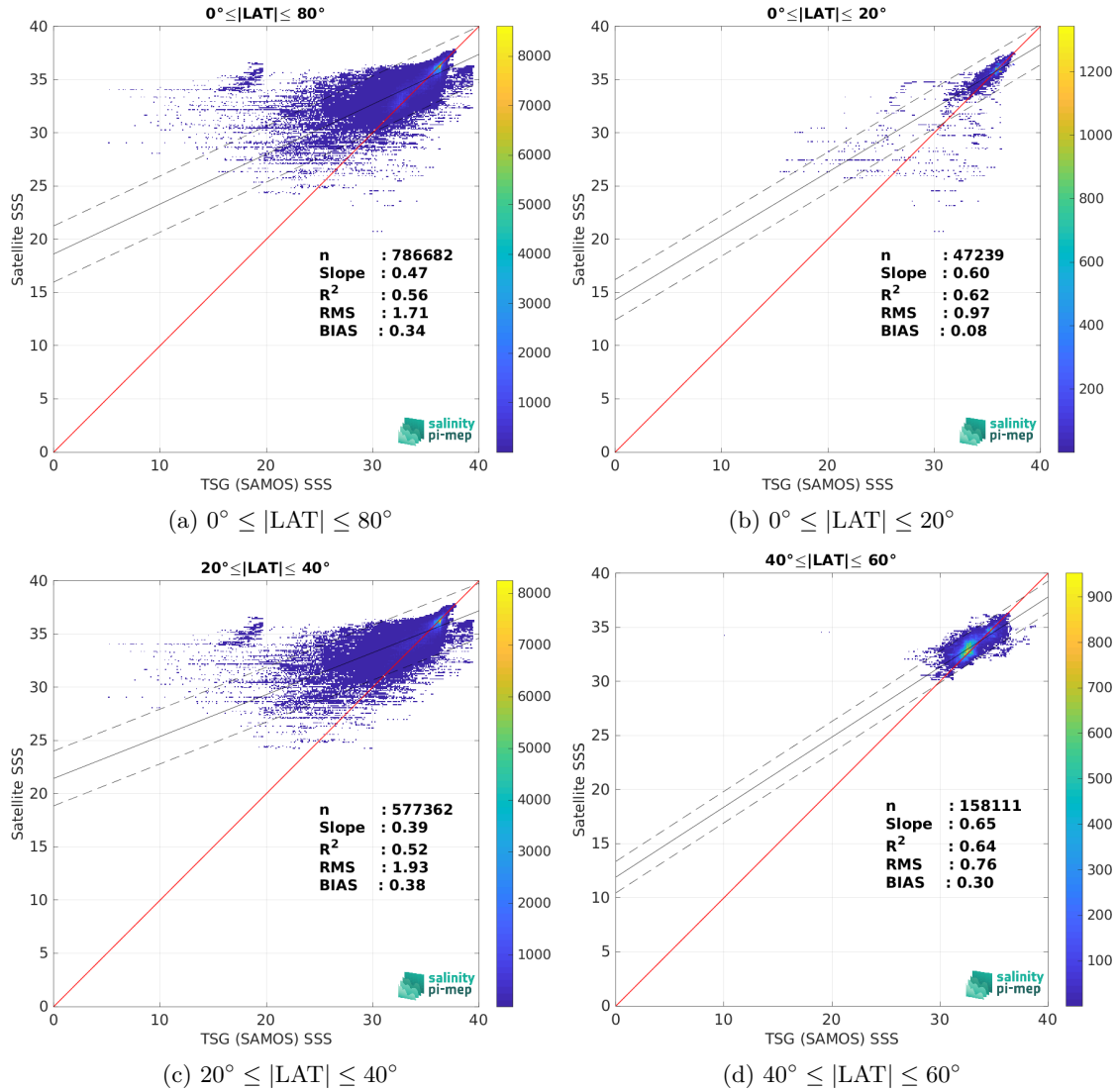
Figure 10: Contour maps of the concentration of SMAP SSS L4 OI v3 - Monthly (ESR) SSS (y-axis) versus TSG (SAMOS) SSS (x-axis) at match-up pairs for different latitude bands. For each plot, the red line shows x=y . The black thin and dashed lines indicate a linear fit through the data cloud and the \pm 95\% confidence levels, respectively. The number match-up pairs n , the slope and R^2 coefficient of the linear fit, the root mean square (RMS) and the mean bias between satellite and in situ data are indicated for each latitude band in each plots.
