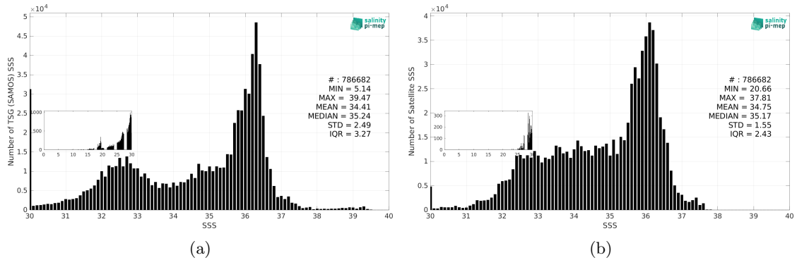
Figure 3: Histograms of SSS from TSG (SAMOS) (a) and SMAP SSS L4 OI v3 - Monthly (ESR) (b) considering all match-up pairs per bins of 0.1 over the Atlantic Ocean Pi-MEP region and for the full satellite product period.
