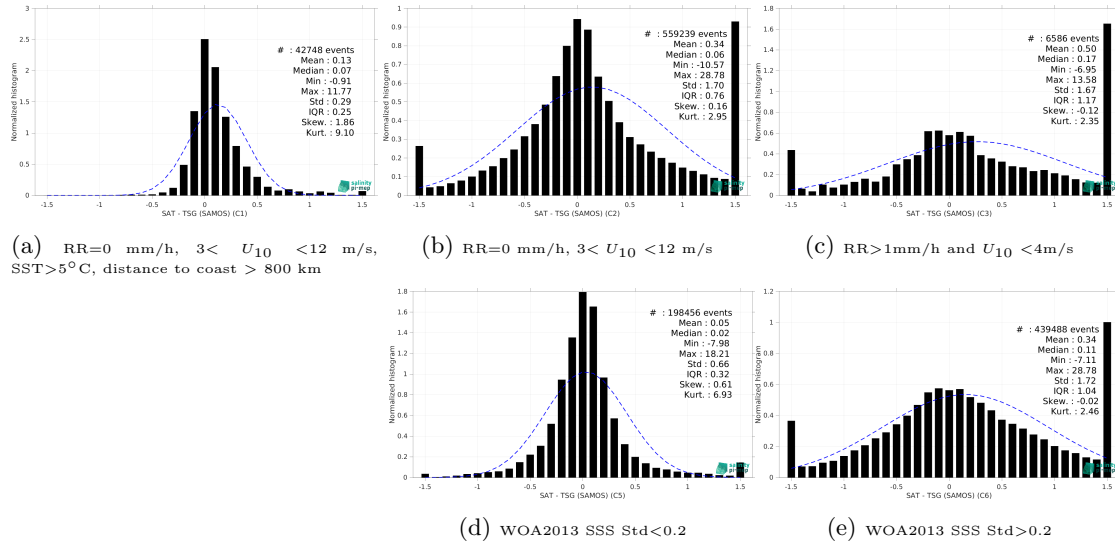
Figure 15: Normalized histogram of \Delta SSS (SMAP SSS L4 OI v3 - Monthly (ESR) - TSG (SAMOS)) for 5 different subdatasets corresponding to: RR=0 mm/h, 3 < U_{10} < 12 m/s, SST>5°C, distance to coast > 800 km (a), RR=0 mm/h, 3 < U_{10} < 12 m/s (b), RR>1mm/h and U_{10} < 4 m/s (c), WOA2013 SSS Std<0.2 (d), WOA2013 SSS Std>0.2 (e).
