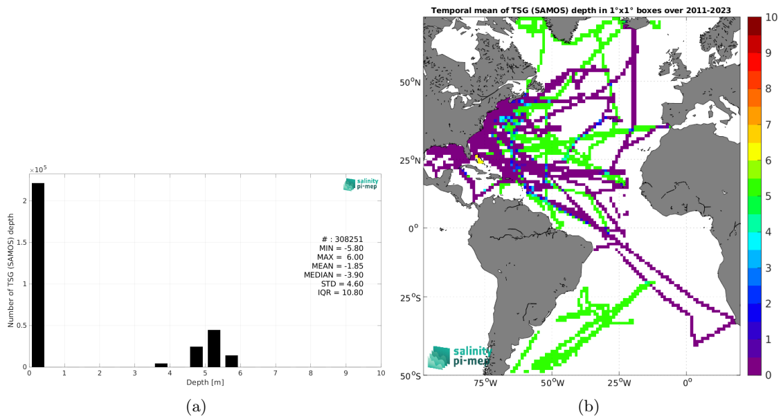
Figure 4: Histograms of the depth of the upper level SSS measurements from TSG (SAMOS) in the Match-up DataBase for the Atlantic Ocean Pi-MEP region (a) and temporal mean spatial distribution of pressure of the in situ SSS data over 1^\circ \times 1^\circ boxes and for the full satellite product period (b).
