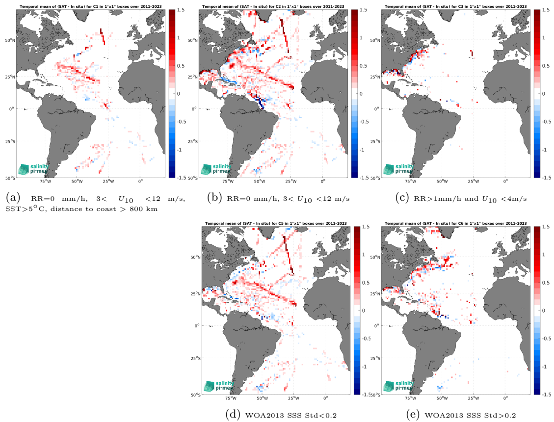
Figure 14: Temporal mean gridded over spatial boxes of size 1^\circ \times 1^\circ of \Delta\text{SSS} (SMAP SSS L4 OI v3 - Monthly (ESR) - TSG (SAMOS)) for 5 different subdatasets corresponding to:RR=0 mm/h, 3 < U_{10} < 12 m/s, SST >5^\circ\text{C} , distance to coast > 800 km (a), RR=0 mm/h, 3 < U_{10} < 12 m/s (b), RR >1 mm/h and U_{10} < 4 m/s (c), WOA2013 SSS Std <0.2 (d), WOA2013 SSS Std >0.2 (e).
