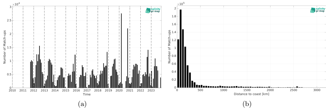
Figure 2: Number of match-ups between TSG (SAMOS) and SMAP SSS L4 OI v3 - Monthly (ESR) SSS as a function of time (a) and as function of the distance to coast (b) over the Atlantic Ocean Pi-MEP region and for the full satellite product period.
