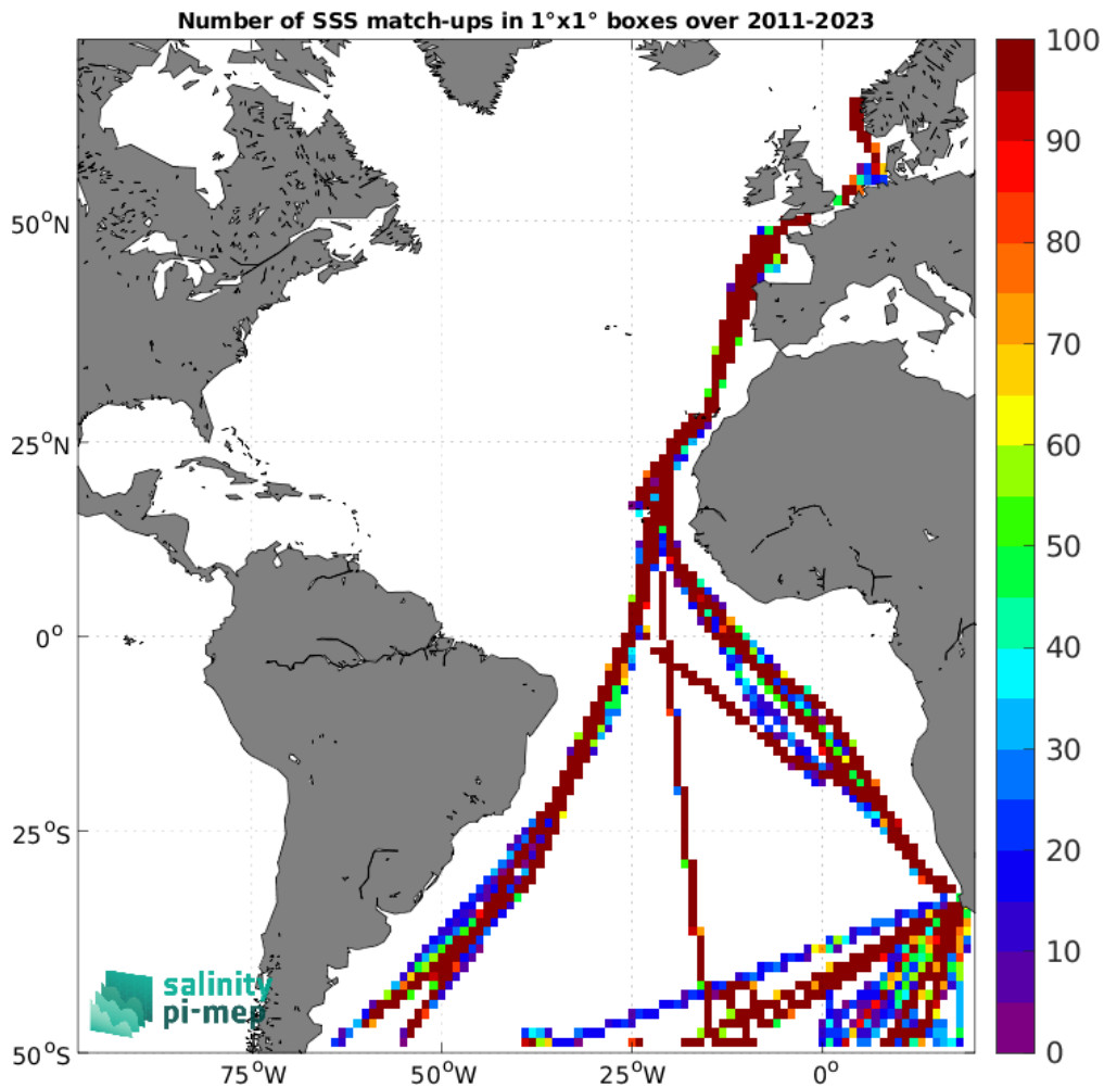
Figure 5: Number of SSS match-ups between TSG (Polarstern) SSS and the SMAP SSS L4 OI v3 - Monthly (ESR) SSS product for the Atlantic Ocean Pi-MEP region over 1°x1° boxes and for the full satellite product period.
