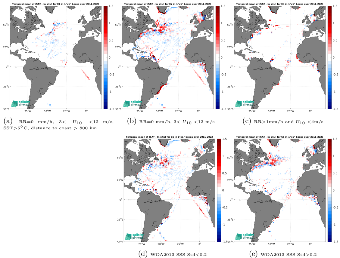
Figure 14: Temporal mean gridded over spatial boxes of size 1^\circ \times 1^\circ of \Delta\text{SSS} (SMAP SSS L4 OI v3 - Monthly (ESR) - TSG (LEGOS-DM)) for 5 different subdatasets corresponding to:RR=0 mm/h, 3 < U_{10} < 12 m/s, SST>5°C, distance to coast > 800 km (a), RR=0 mm/h, 3 < U_{10} < 12 m/s (b), RR>1mm/h and U_{10} < 4 m/s (c), WOA2013 SSS Std<0.2 (d), WOA2013 SSS Std>0.2 (e).
