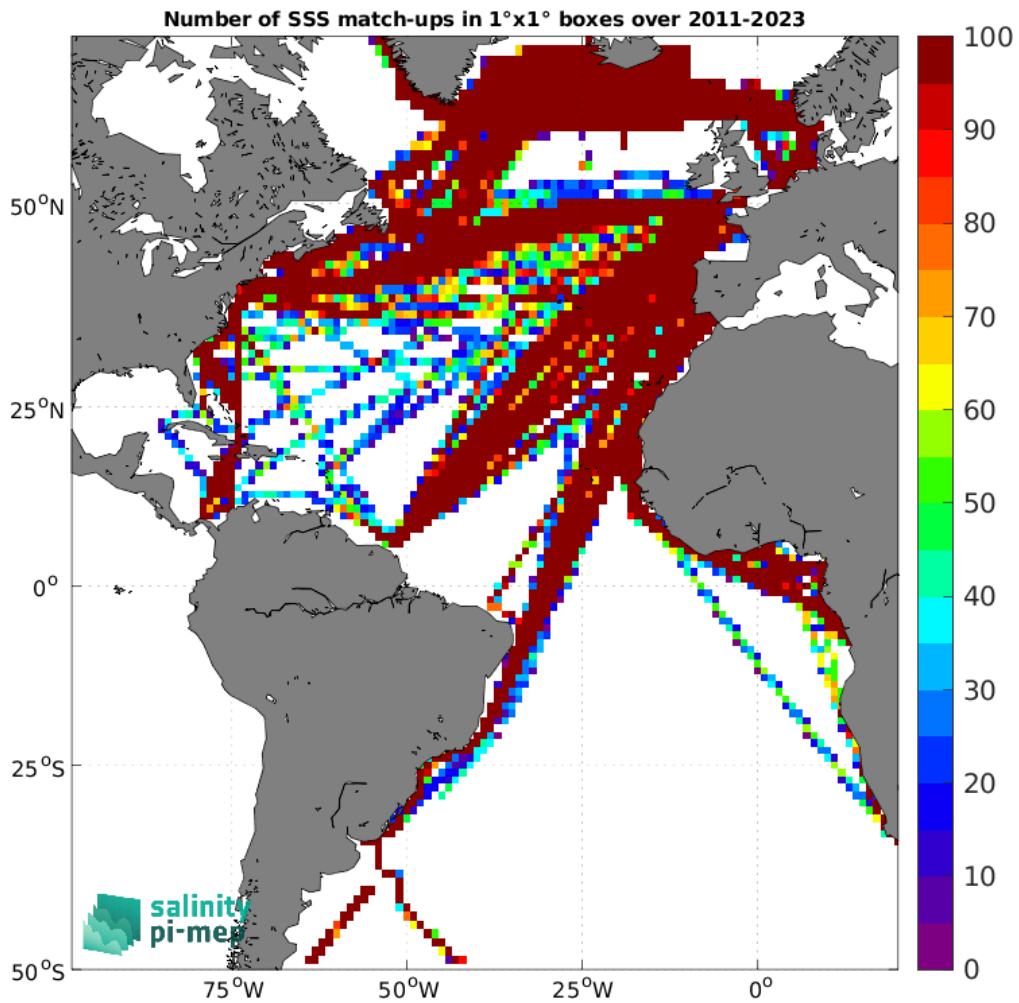
Figure 5: Number of SSS match-ups between TSG (LEGOS-DM) SSS and the SMAP SSS L4 OI v3 - Monthly (ESR) SSS product for the Atlantic Ocean Pi-MEP region over 1^\circ \times 1^\circ boxes and for the full satellite product period.
