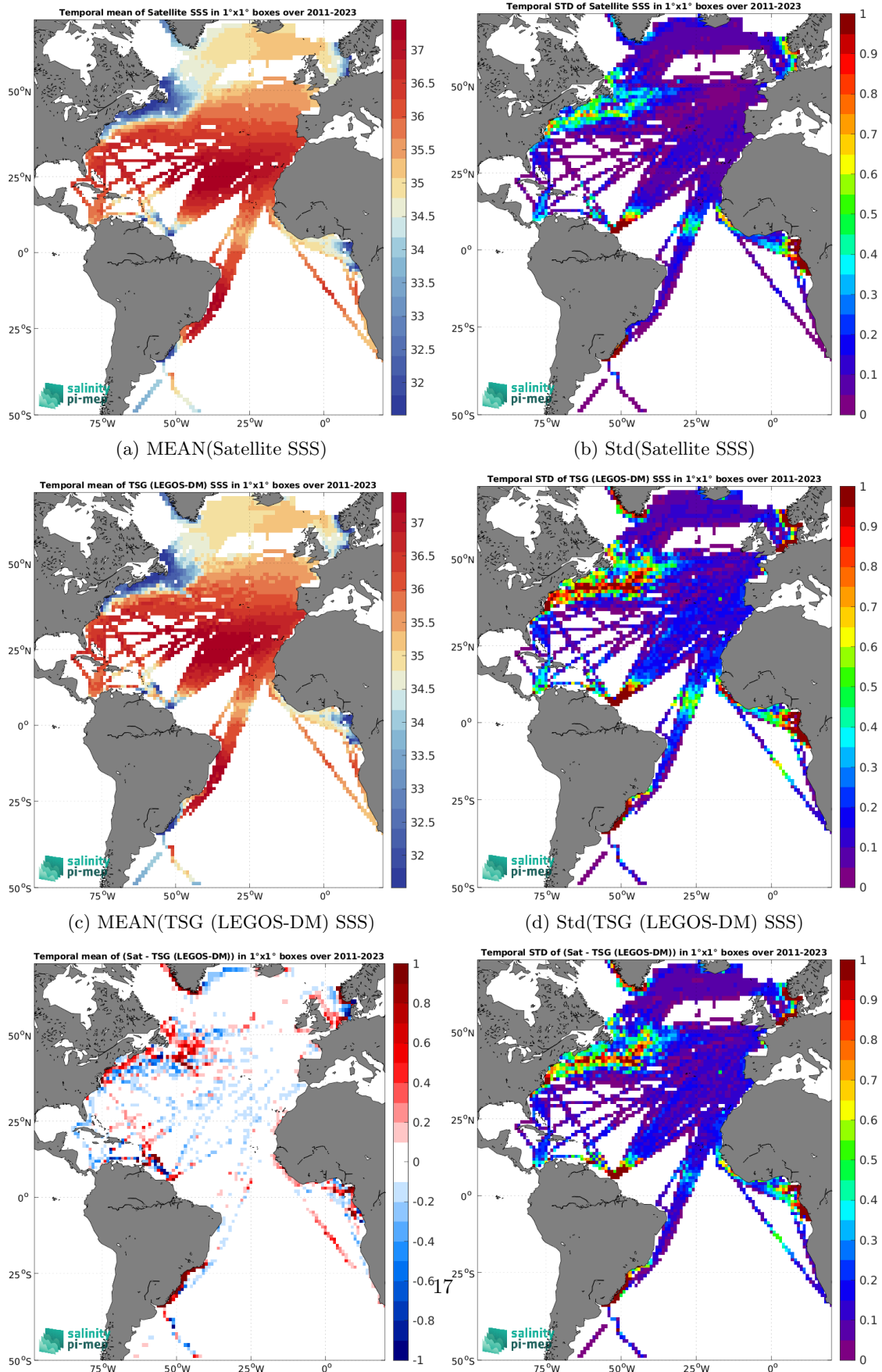
Figure 7: Temporal mean (left) and Std (right) of SSS from SMAP SSS L4 OI v3 - Monthly (ESR) (top), TSG (LEGOS-DM) (middle), and of \Delta SSS (Satellite - TSG (LEGOS-DM)). Only match-up pairs are used to generate these maps.
