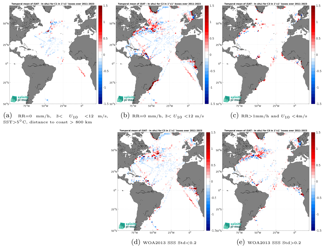
Figure 14: Temporal mean gridded over spatial boxes of size 1^\circ \times 1^\circ of \Delta SSS (SMAP SSS L4 OI v3 - Monthly (ESR) - TSG (LEGOS-DM)) for 5 different subdatasets corresponding to:RR=0 mm/h, 3 < U_{10} < 12 m/s, SST >5^\circ\text{C} , distance to coast > 800 km (a), RR=0 mm/h, 3 < U_{10} < 12 m/s (b), RR >1 mm/h and U_{10} < 4 m/s (c), WOA2013 SSS Std <0.2 (d), WOA2013 SSS Std >0.2 (e).
