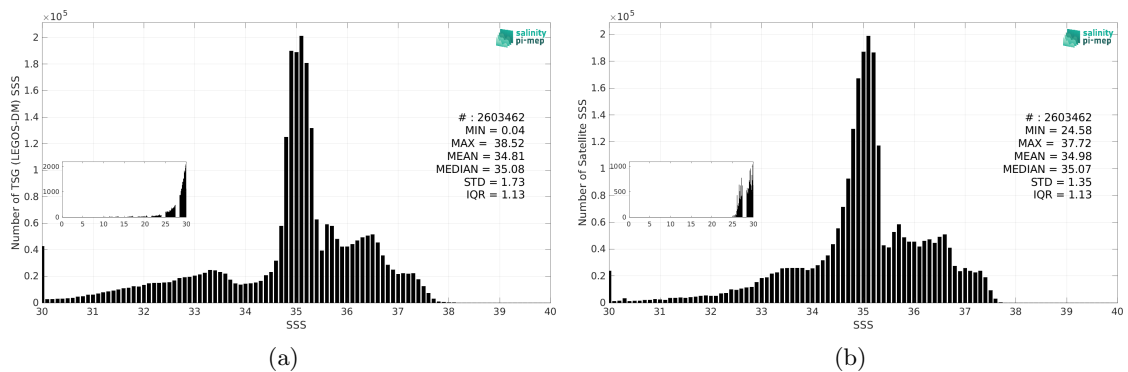
Figure 3: Histograms of SSS from TSG (LEGOS-DM) (a) and SMAP SSS L4 OI v3 - Monthly (ESR) (b) considering all match-up pairs per bins of 0.1 over the Atlantic Ocean Pi-MEP region and for the full satellite product period.
