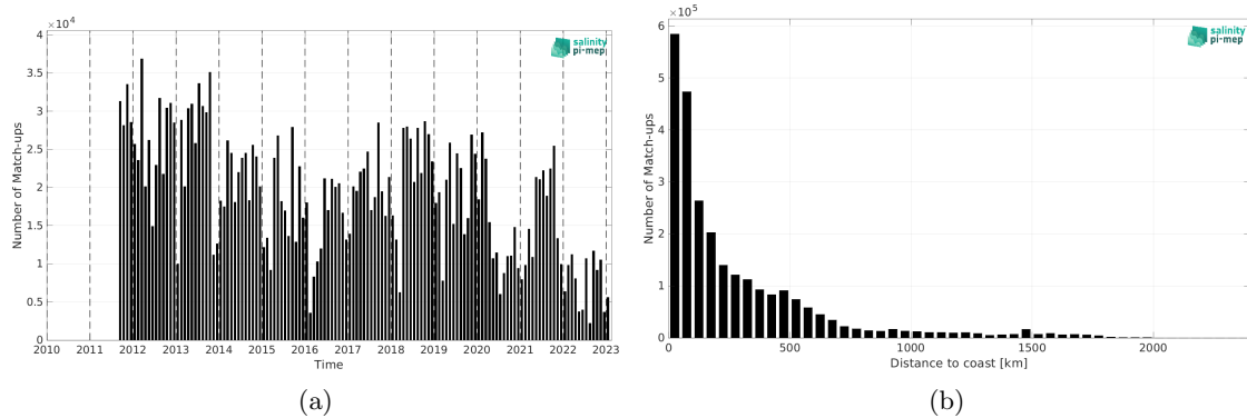
Figure 2: Number of match-ups between TSG (LEGOS-DM) and SMAP SSS L4 OI v3 - Monthly (ESR) SSS as a function of time (a) and as function of the distance to coast (b) over the Atlantic Ocean Pi-MEP region and for the full satellite product period.
