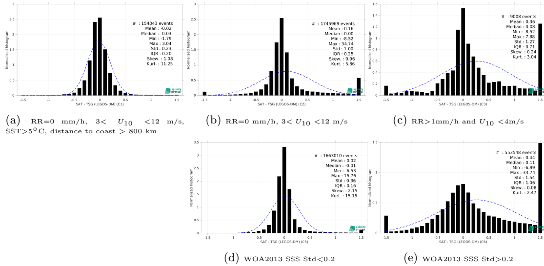
Figure 15: Normalized histogram of \Delta\text{SSS} (SMAP SSS L4 OI v3 - Monthly (ESR) - TSG (LEGOS-DM)) for 5 different subdatasets corresponding to: RR=0 mm/h, 3 < U_{10} < 12 m/s, SST>5°C, distance to coast > 800 km (a), RR=0 mm/h, 3 < U_{10} < 12 m/s (b), RR>1mm/h and U_{10} < 4 m/s (c), WOA2013 SSS Std<0.2 (d), WOA2013 SSS Std>0.2 (e).
