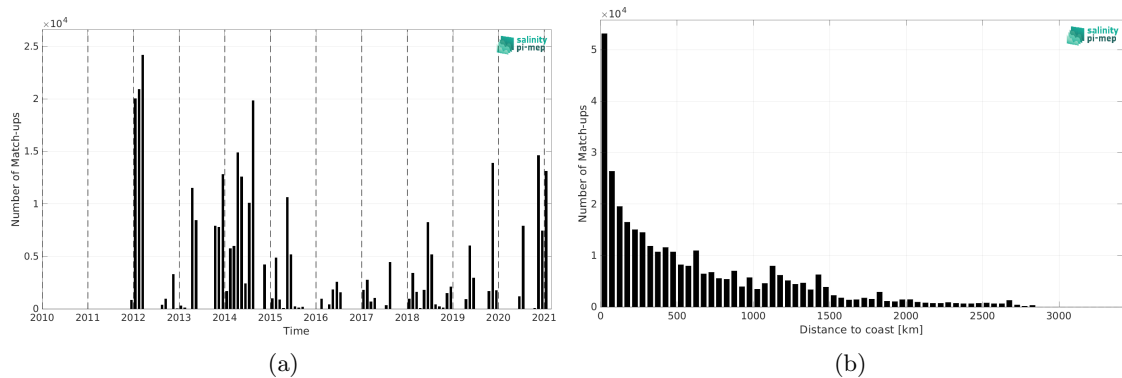
Figure 2: Number of match-ups between TSG (GOSUD-Sailing-ship) and SMAP SSS L4 OI v3 - Monthly (ESR) SSS as a function of time (a) and as function of the distance to coast (b) over the Atlantic Ocean Pi-MEP region and for the full satellite product period.
