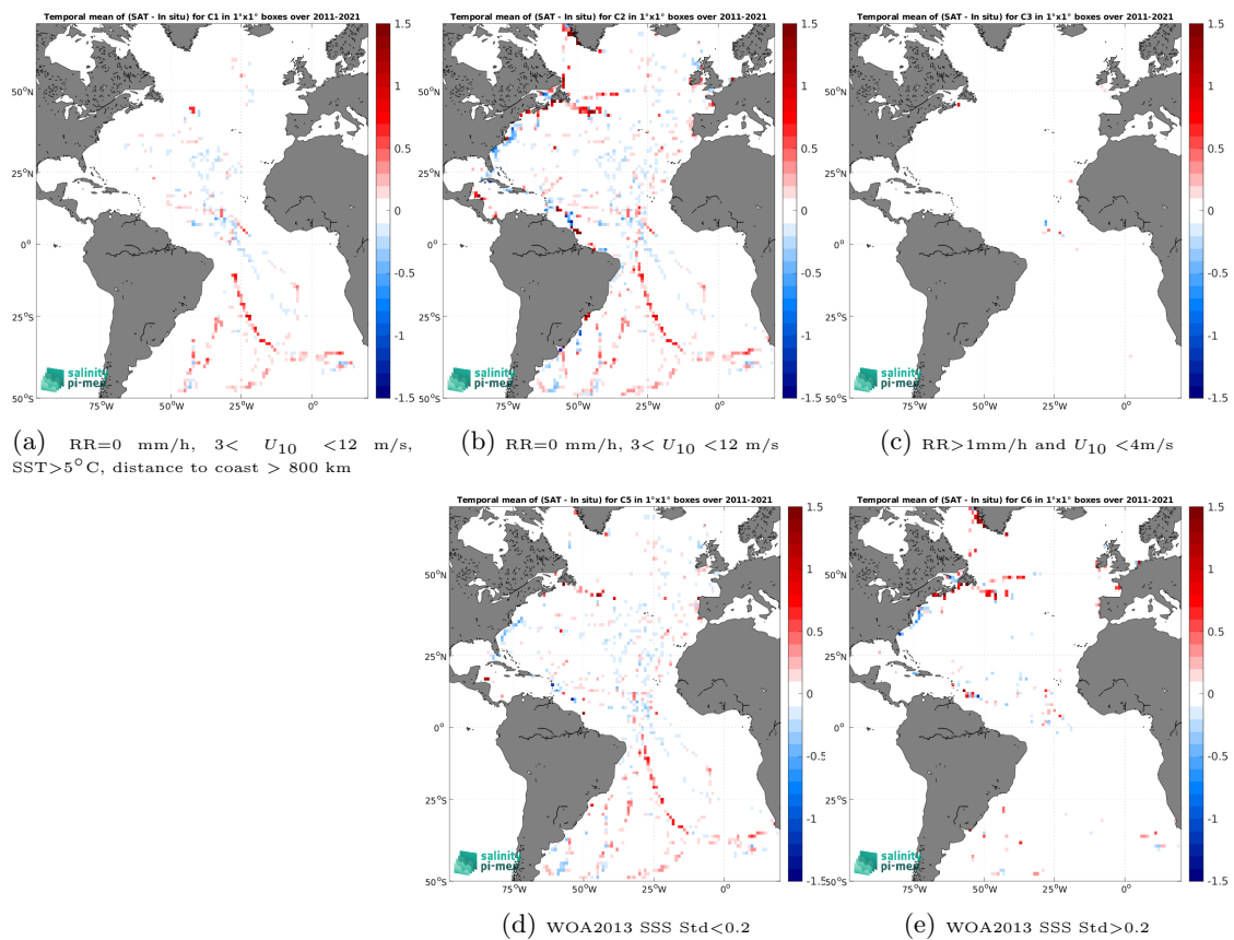
Figure 14: Temporal mean gridded over spatial boxes of size 1^\circ \times 1^\circ of \Delta\text{SSS} (SMAP SSS L4 OI v3 - Monthly (ESR) - TSG (GOSUD-Sailing-ship)) for 5 different subdatasets corresponding to:RR=0 mm/h, 3 < U_{10} < 12 m/s, SST>5°C, distance to coast > 800 km (a), RR=0 mm/h, 3 < U_{10} < 12 m/s (b), RR>1mm/h and U_{10} < 4 m/s (c), WOA2013 SSS Std<0.2 (d), WOA2013 SSS Std>0.2 (e).
