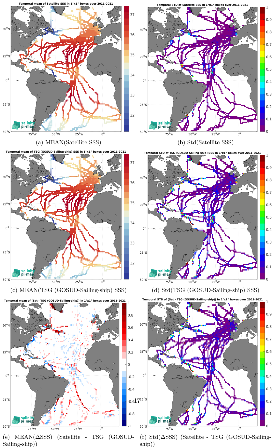
Figure 7: Temporal mean (left) and Std (right) of SSS from SMAP SSS L4 OI v3 - Monthly (ESR) (top), TSG (GOSUD-Sailing-ship) (middle), and of \Delta SSS (Satellite - TSG (GOSUD-Sailing-ship)). Only match-up pairs are used to generate these maps.
