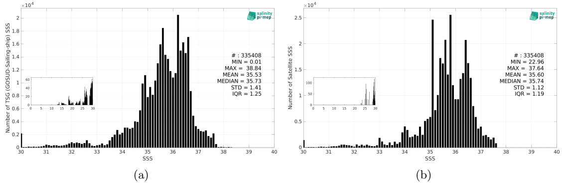
Figure 3: Histograms of SSS from TSG (GOSUD-Sailing-ship) (a) and SMAP SSS L4 OI v3 - Monthly (ESR) (b) considering all match-up pairs per bins of 0.1 over the Atlantic Ocean Pi-MEP region and for the full satellite product period.
