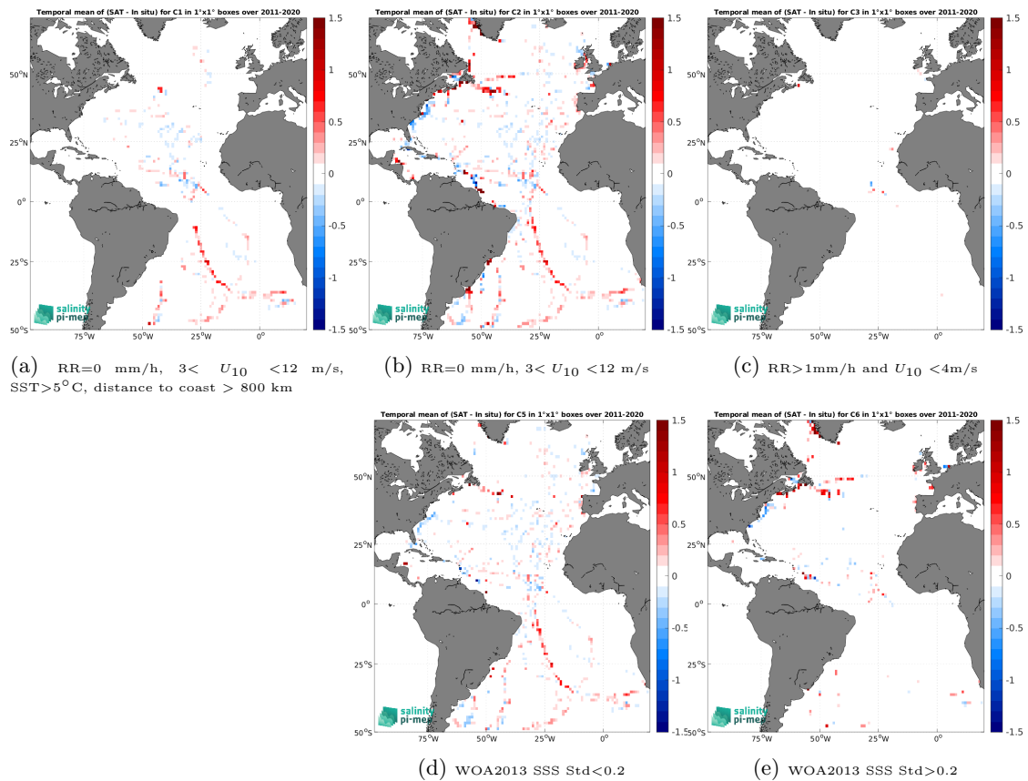
Figure 14: Temporal mean gridded over spatial boxes of size 1^\circ \times 1^\circ of \Delta SSS (SMAP SSS L4 OI v3 - Monthly (ESR) - TSG (GOSUD-Sailing-ship)) for 5 different subdatasets corresponding to:RR=0 mm/h, 3 < U_{10} < 12 m/s, SST >5^\circ\text{C} , distance to coast > 800 km (a), RR=0 mm/h, 3 < U_{10} < 12 m/s (b), RR >1 mm/h and U_{10} < 4 m/s (c), WOA2013 SSS Std <0.2 (d), WOA2013 SSS Std >0.2 (e).
