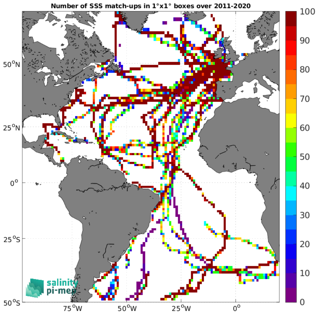
Figure 5: Number of SSS match-ups between TSG (GOSUD-Sailing-ship) SSS and the SMAP SSS L4 OI v3 - Monthly (ESR) SSS product for the Atlantic Ocean Pi-MEP region over 1^\circ \times 1^\circ boxes and for the full satellite product period.
