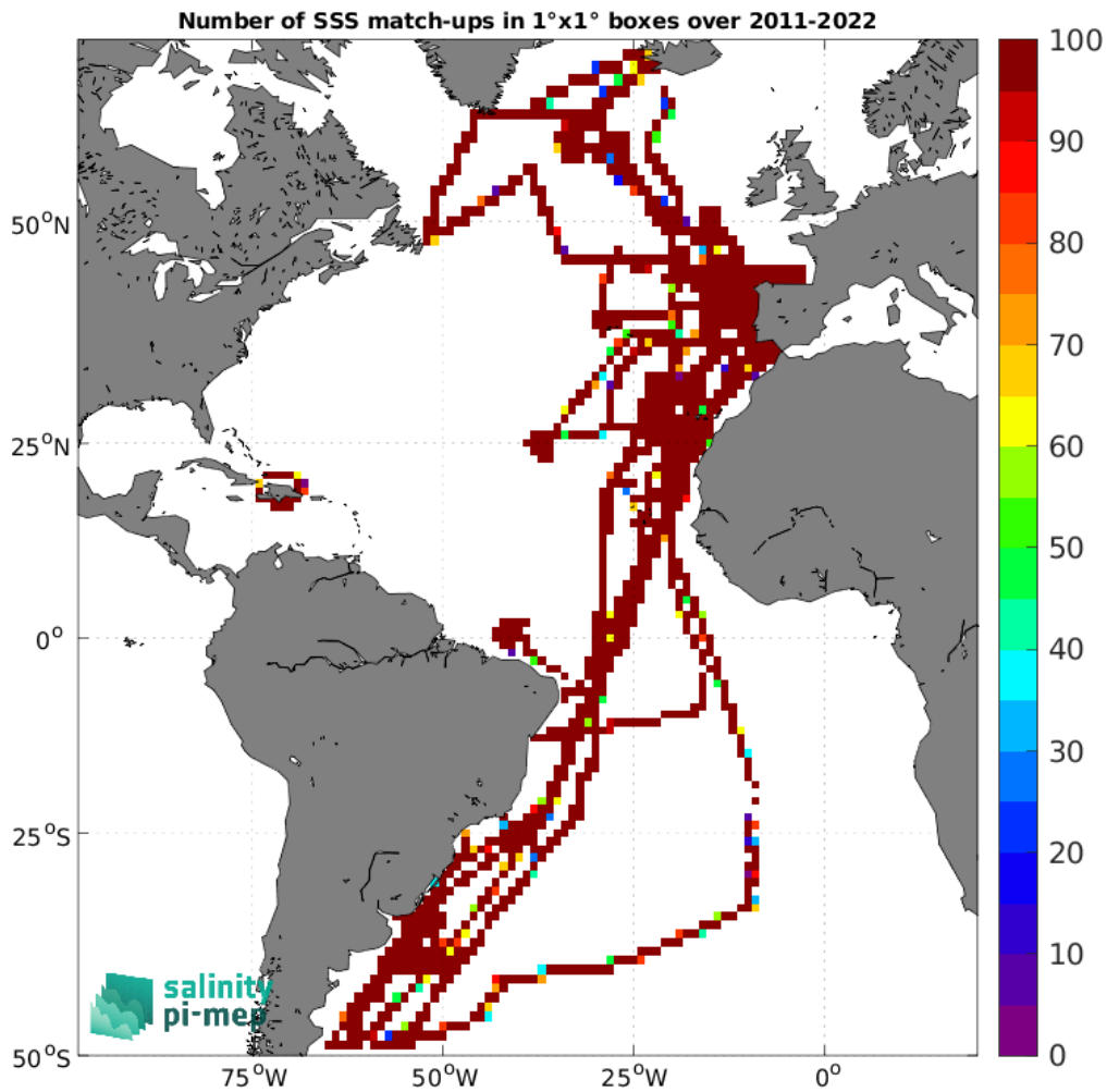
Figure 5: Number of SSS match-ups between TSG (CSIC-UTM) SSS and the SMAP SSS L4 OI v3 - Monthly (ESR) SSS product for the Atlantic Ocean Pi-MEP region over 1°x1° boxes and for the full satellite product period.
