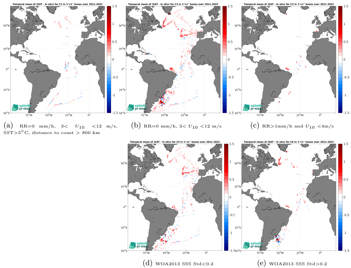
Figure 14: Temporal mean gridded over spatial boxes of size 1^\circ \times 1^\circ of \Delta\text{SSS} (SMAP SSS L4 OI v3 - Monthly (ESR) - TSG (CSIC-UTM)) for 5 different subdatasets corresponding to:RR=0 mm/h, 3 < U_{10} < 12 m/s, SST>5°C, distance to coast > 800 km (a), RR=0 mm/h, 3 < U_{10} < 12 m/s (b), RR>1mm/h and U_{10} < 4 m/s (c), WOA2013 SSS Std<0.2 (d), WOA2013 SSS Std>0.2 (e).
