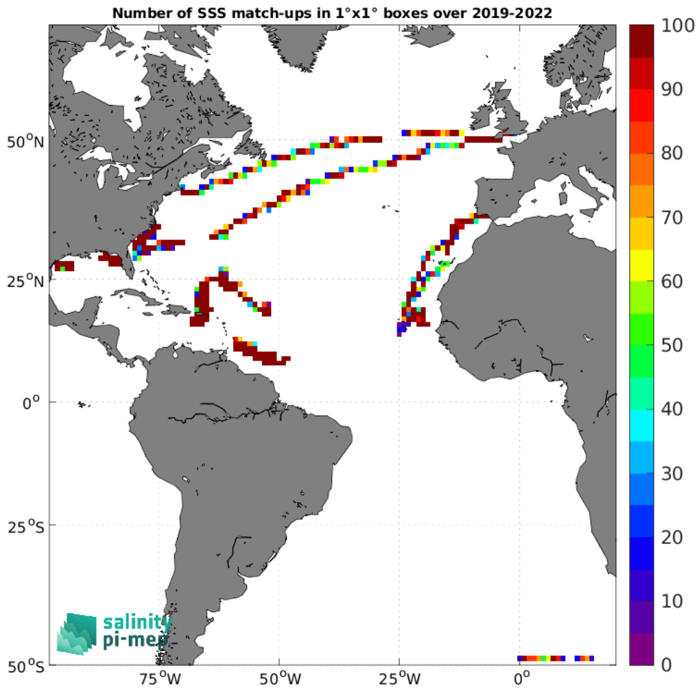
Figure 5: Number of SSS match-ups between Saildrone SSS and the SMAP SSS L4 OI v3 - Monthly (ESR) SSS product for the Atlantic Ocean Pi-MEP region over 1^\circ \times 1^\circ boxes and for the full satellite product period.
