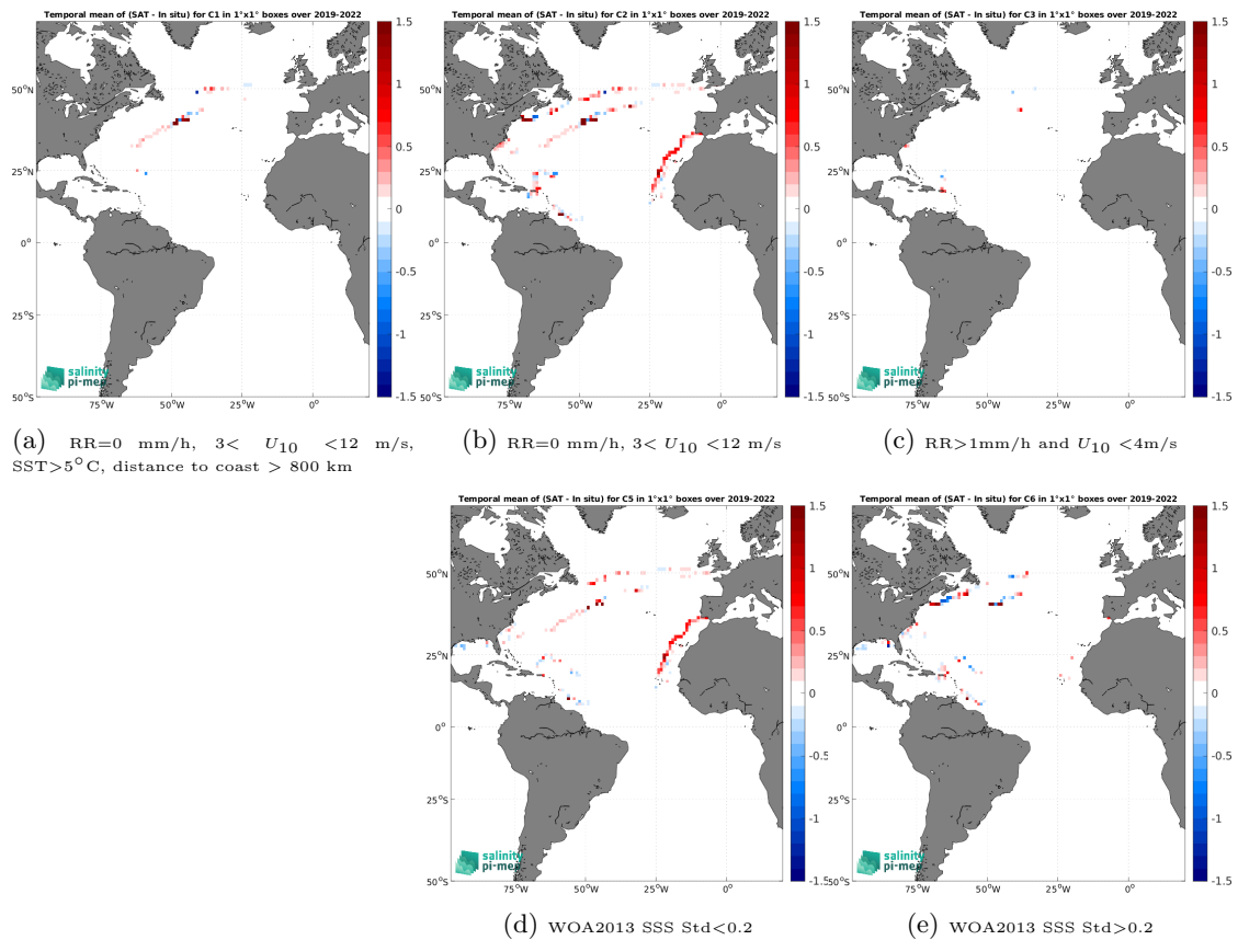
Figure 14: Temporal mean gridded over spatial boxes of size 1^\circ \times 1^\circ of \Delta SSS (SMAP SSS L4 OI v3 - Monthly (ESR) - Saildrone) for 5 different subdatasets corresponding to:RR=0 mm/h, 3 < U_{10} < 12 m/s, SST>5°C, distance to coast > 800 km (a), RR=0 mm/h, 3 < U_{10} < 12 m/s (b), RR>1mm/h and U_{10} < 4 m/s (c), WOA2013 SSS Std<0.2 (d), WOA2013 SSS Std>0.2 (e).
