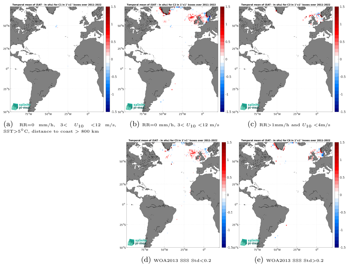
Figure 14: Temporal mean gridded over spatial boxes of size 1^\circ \times 1^\circ of \Delta SSS (SMAP SSS L4 OI v3 - Monthly (ESR) - ICES) for 5 different subdatasets corresponding to:RR=0 mm/h, 3 < U_{10} < 12 m/s, SST >5^\circ\text{C} , distance to coast > 800 km (a), RR=0 mm/h, 3 < U_{10} < 12 m/s (b), RR >1 mm/h and U_{10} < 4 m/s (c), WOA2013 SSS Std <0.2 (d), WOA2013 SSS Std >0.2 (e).
