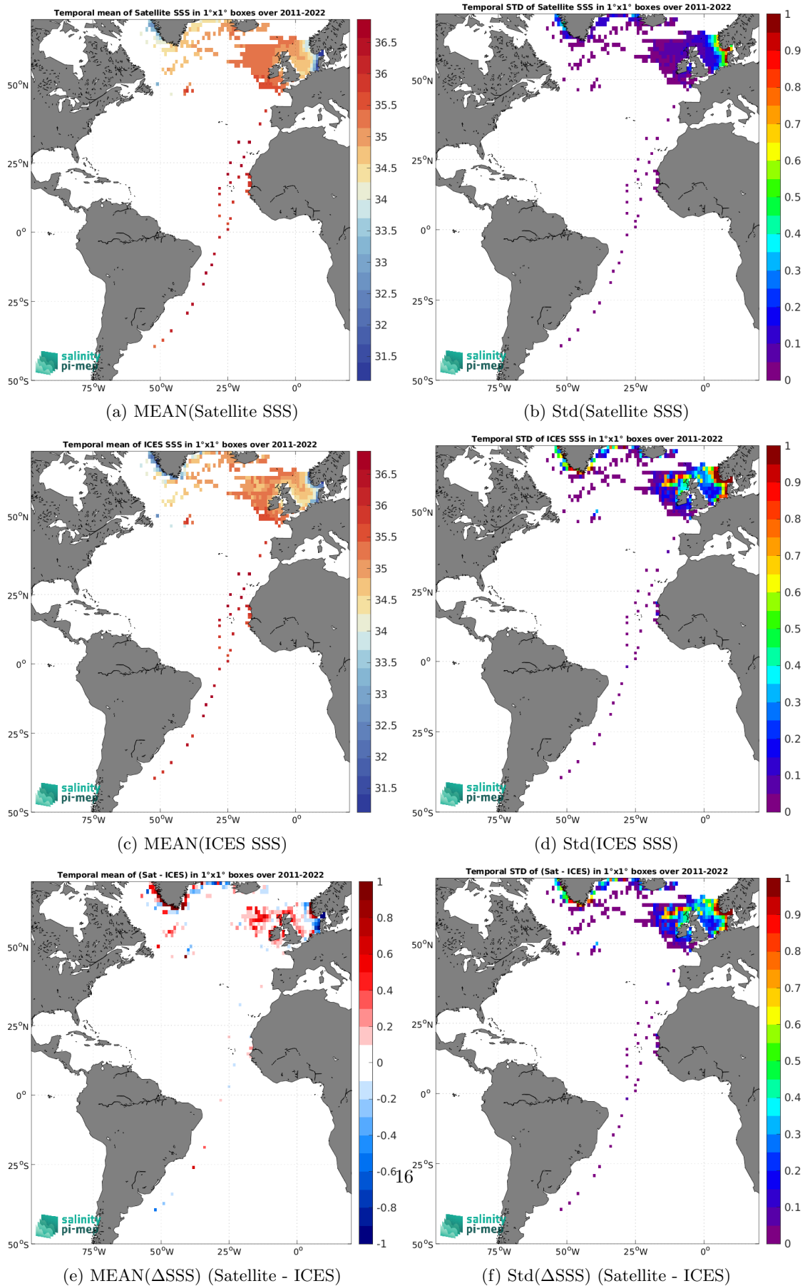
Figure 7: Temporal mean (left) and Std (right) of SSS from SMAP SSS L4 OI v3 - Monthly (ESR) (top), ICES (middle), and of \Delta\text{SSS} (Satellite - ICES). Only match-up pairs are used to generate these maps.
