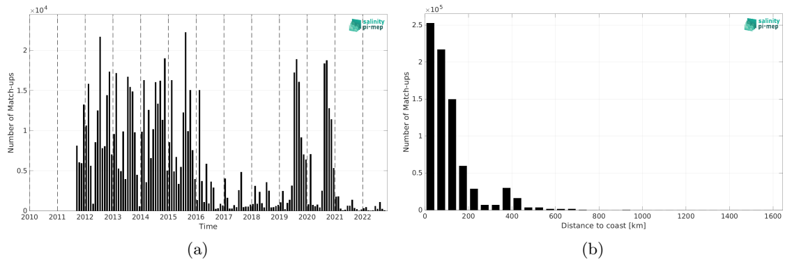
Figure 2: Number of match-ups between ICES and SMAP SSS L4 OI v3 - Monthly (ESR) SSS as a function of time (a) and as function of the distance to coast (b) over the Atlantic Ocean Pi-MEP region and for the full satellite product period.
