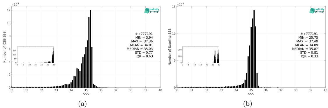
Figure 3: Histograms of SSS from ICES (a) and SMAP SSS L4 OI v3 - Monthly (ESR) (b) considering all match-up pairs per bins of 0.1 over the Atlantic Ocean Pi-MEP region and for the full satellite product period.
