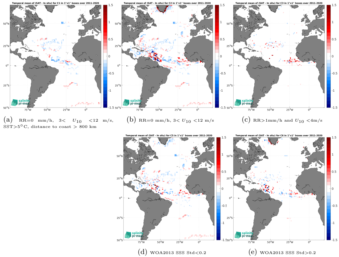
Figure 13: Temporal mean gridded over spatial boxes of size 1^\circ \times 1^\circ of \Delta SSS (SMAP SSS L4 OI v3 - Monthly (ESR) - Surface drifters) for 5 different subdatasets corresponding to:RR=0 mm/h, 3 < U_{10} < 12 m/s, SST >5^\circ\text{C} , distance to coast > 800 km (a), RR=0 mm/h, 3 < U_{10} < 12 m/s (b), RR >1 mm/h and U_{10} < 4 m/s (c), WOA2013 SSS Std <0.2 (d), WOA2013 SSS Std >0.2 (e).
