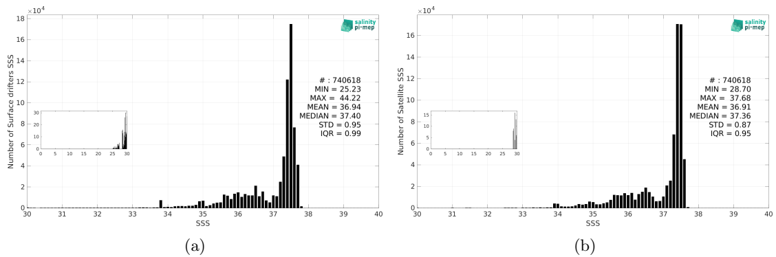
Figure 3: Histograms of SSS from Surface drifters (a) and SMAP SSS L4 OI v3 - Monthly (ESR) (b) considering all match-up pairs per bins of 0.1 over the Atlantic Ocean Pi-MEP region and for the full satellite product period.
