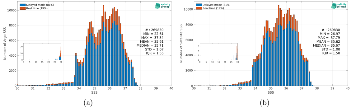
Figure 3: Histograms of SSS from Argo (a) and SMAP SSS L4 OI v3 - Monthly (ESR) (b) considering all match-up pairs per bins of 0.1 over the Atlantic Ocean Pi-MEP region and for the full satellite product period.
