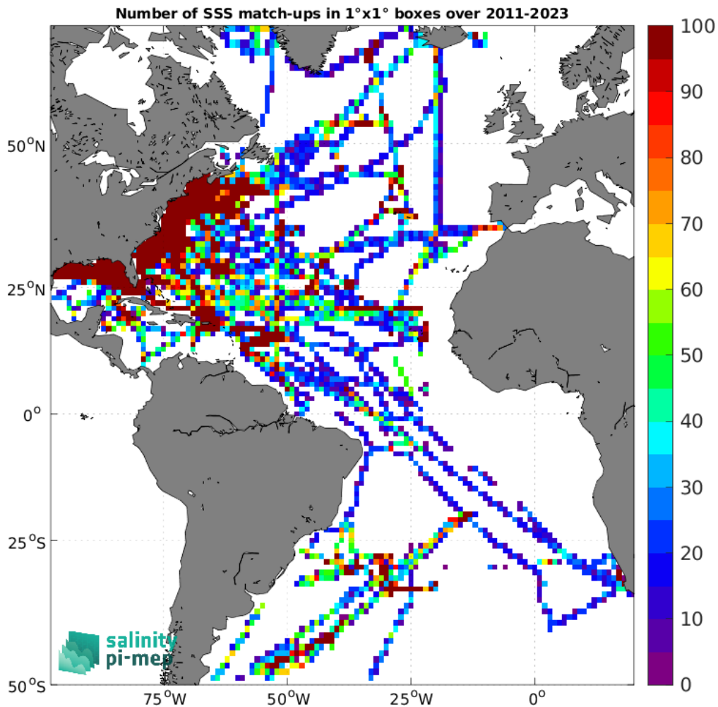
Figure 5: Number of SSS match-ups between TSG (SAMOS) SSS and the SMAP SSS L4 OI v3 - Daily (ESR) SSS product for the Atlantic Ocean Pi-MEP region over 1^\circ \times 1^\circ boxes and for the full satellite product period.
