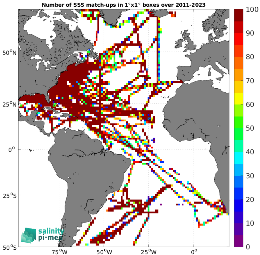
Figure 5: Number of SSS match-ups between TSG (SAMOS) SSS and the SMAP SSS L4 OI v3 - Daily (ESR) SSS product for the Atlantic Ocean Pi-MEP region over 1°×1° boxes and for the full satellite product period.
