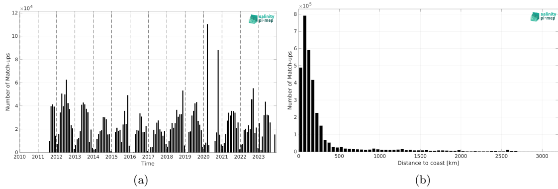
Figure 2: Number of match-ups between TSG (SAMOS) and SMAP SSS L4 OI v3 - Daily (ESR) SSS as a function of time (a) and as function of the distance to coast (b) over the Atlantic Ocean Pi-MEP region and for the full satellite product period.
