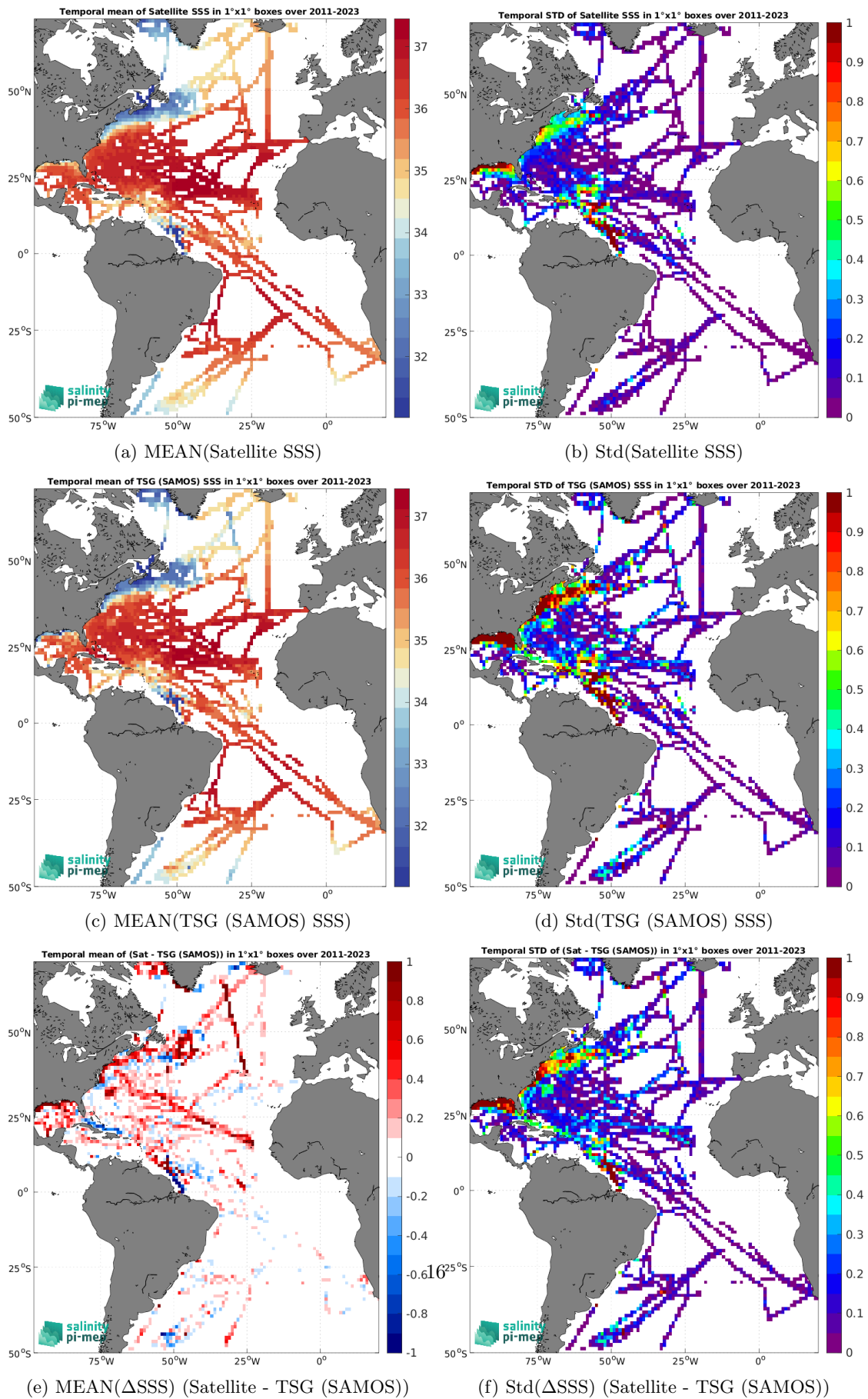
Figure 7: Temporal mean (left) and Std (right) of SSS from SMAP SSS L4 OI v3 - Daily (ESR) (top), TSG (SAMOS) (middle), and of \Delta SSS (Satellite - TSG (SAMOS)). Only match-up pairs are used to generate these maps.
