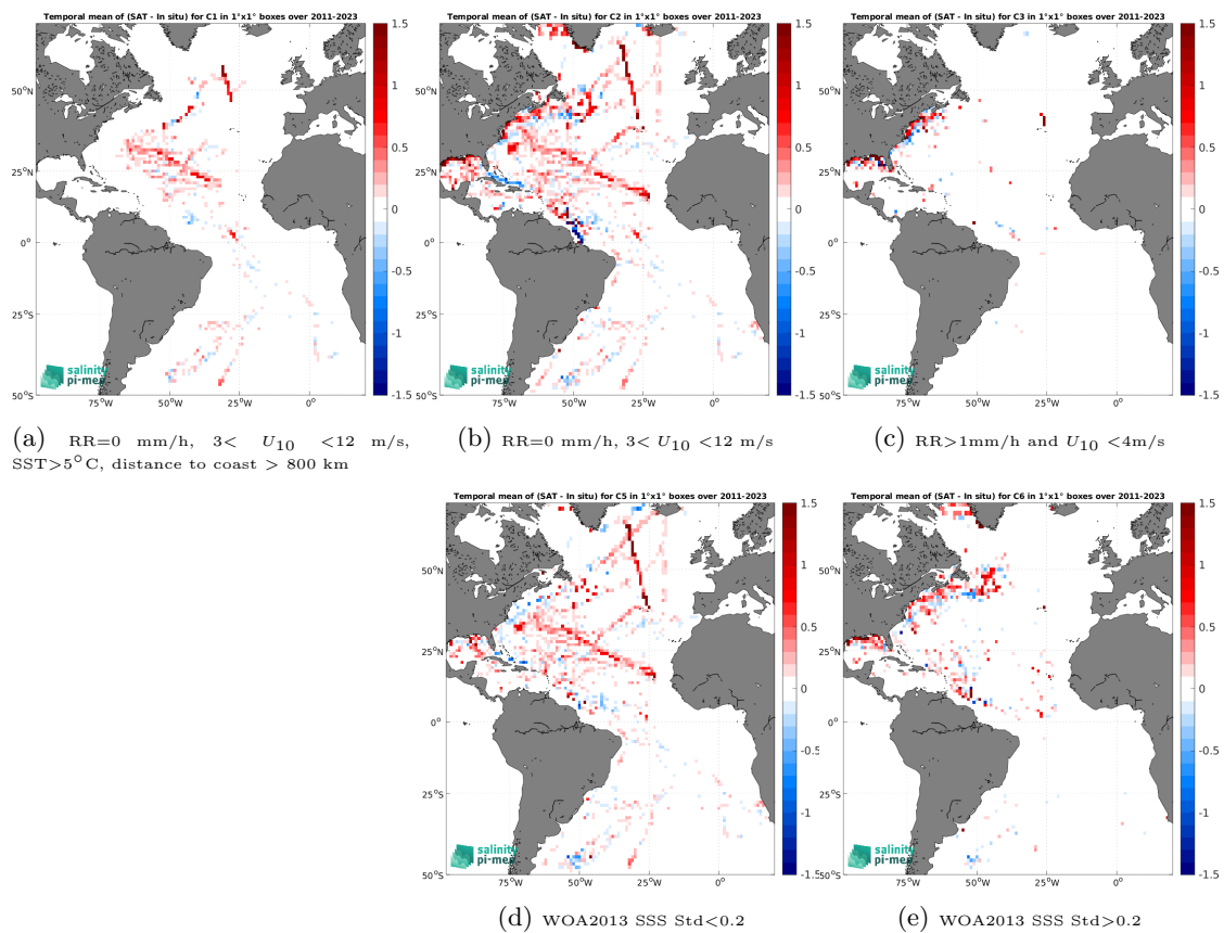
Figure 14: Temporal mean gridded over spatial boxes of size 1^\circ \times 1^\circ of \Delta\text{SSS} (SMAP SSS L4 OI v3 - Daily (ESR) - TSG (SAMOS)) for 5 different subdatasets corresponding to:RR=0 mm/h, 3 < U_{10} < 12 m/s, SST>5°C, distance to coast > 800 km (a), RR=0 mm/h, 3 < U_{10} < 12 m/s (b), RR>1mm/h and U_{10} < 4 m/s (c), WOA2013 SSS Std<0.2 (d), WOA2013 SSS Std>0.2 (e).
