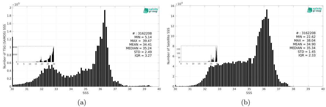
Figure 3: Histograms of SSS from TSG (SAMOS) (a) and SMAP SSS L4 OI v3 - Daily (ESR) (b) considering all match-up pairs per bins of 0.1 over the Atlantic Ocean Pi-MEP region and for the full satellite product period.
