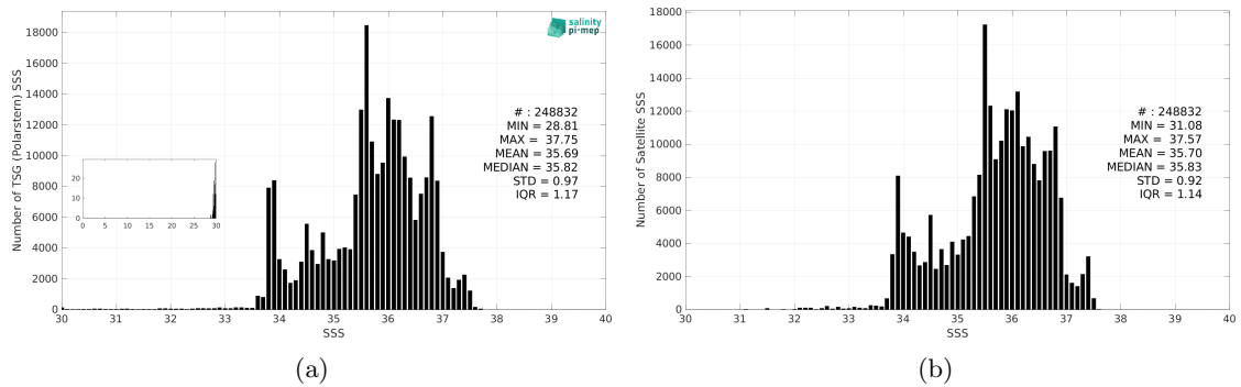
Figure 3: Histograms of SSS from TSG (Polarstern) (a) and SMAP SSS L4 OI v3 - Daily (ESR) (b) considering all match-up pairs per bins of 0.1 over the Atlantic Ocean Pi-MEP region and for the full satellite product period.
