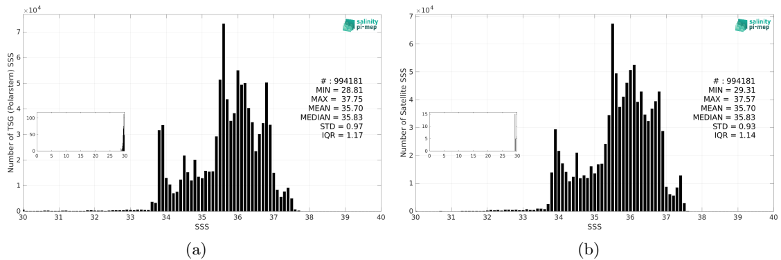
Figure 3: Histograms of SSS from TSG (Polarstern) (a) and SMAP SSS L4 OI v3 - Daily (ESR) (b) considering all match-up pairs per bins of 0.1 over the Atlantic Ocean Pi-MEP region and for the full satellite product period.
