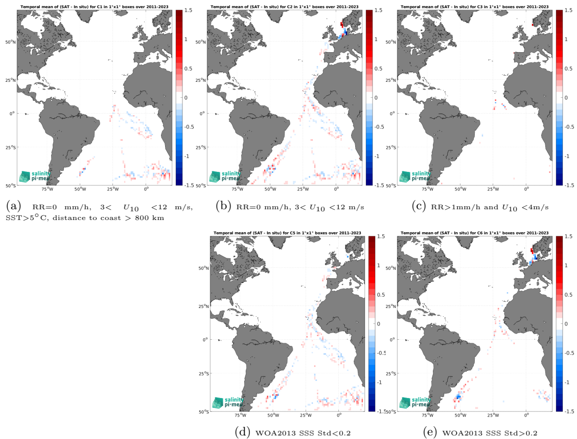
Figure 14: Temporal mean gridded over spatial boxes of size 1^\circ \times 1^\circ of \Delta\text{SSS} (SMAP SSS L4 OI v3 - Daily (ESR) - TSG (Polarstern)) for 5 different subdatasets corresponding to:RR=0 mm/h, 3 < U_{10} < 12 m/s, SST>5°C, distance to coast > 800 km (a), RR=0 mm/h, 3 < U_{10} < 12 m/s (b), RR>1mm/h and U_{10} < 4 m/s (c), WOA2013 SSS Std<0.2 (d), WOA2013 SSS Std>0.2 (e).
