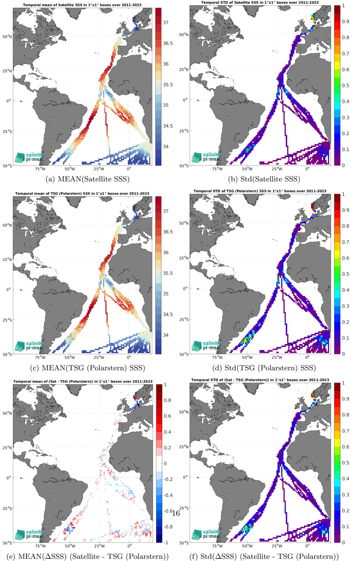
Figure 7: Temporal mean (left) and Std (right) of SSS from SMAP SSS L4 OI v3 - Daily (ESR) (top), TSG (Polarstern) (middle), and of \Delta SSS (Satellite - TSG (Polarstern)). Only match-up pairs are used to generate these maps.
