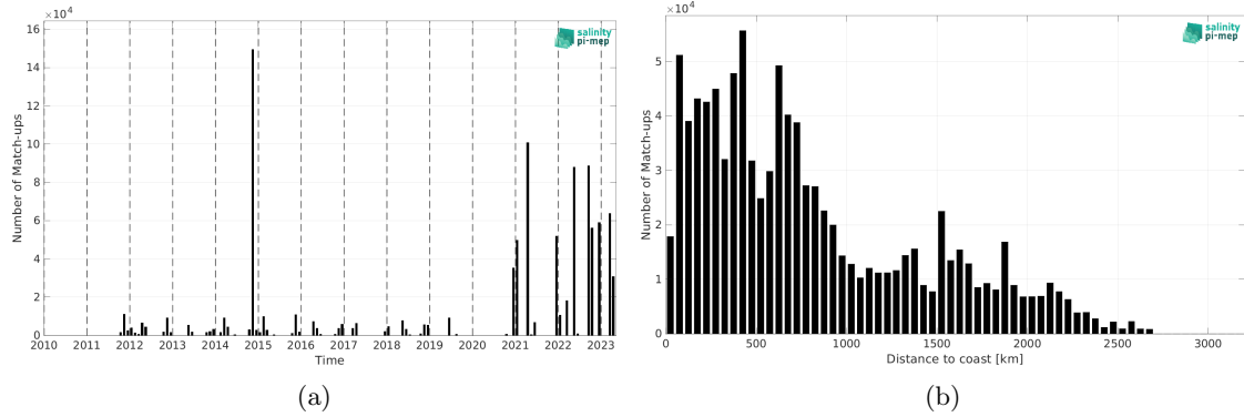
Figure 2: Number of match-ups between TSG (Polarstern) and SMAP SSS L4 OI v3 - Daily (ESR) SSS as a function of time (a) and as function of the distance to coast (b) over the Atlantic Ocean Pi-MEP region and for the full satellite product period.
