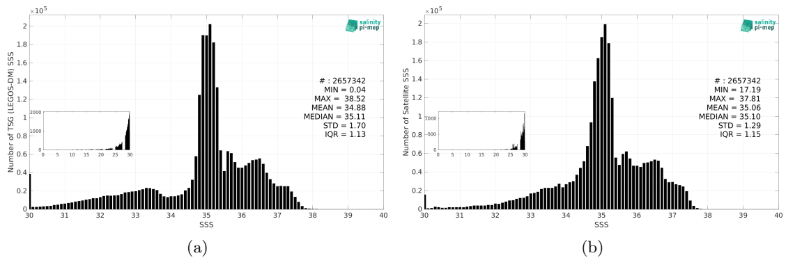
Figure 3: Histograms of SSS from TSG (LEGOS-DM) (a) and SMAP SSS L4 OI v3 - Daily (ESR) (b) considering all match-up pairs per bins of 0.1 over the Atlantic Ocean Pi-MEP region and for the full satellite product period.
