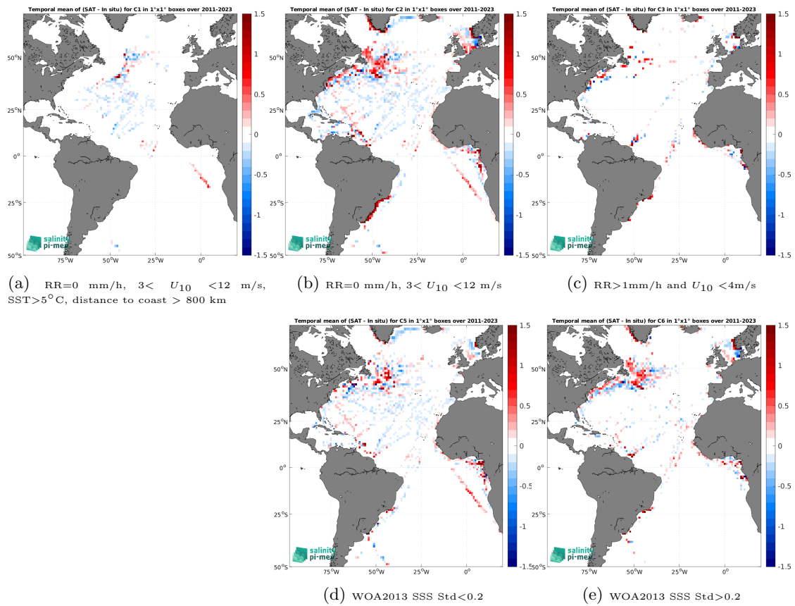
Figure 14: Temporal mean gridded over spatial boxes of size 1^\circ \times 1^\circ of \Delta\text{SSS} (SMAP SSS L4 OI v3 - Daily (ESR) - TSG (LEGOS-DM)) for 5 different subdatasets corresponding to:RR=0 mm/h, 3 < U_{10} < 12 m/s, SST>5°C, distance to coast > 800 km (a), RR=0 mm/h, 3 < U_{10} < 12 m/s (b), RR>1mm/h and U_{10} < 4 m/s (c), WOA2013 SSS Std<0.2 (d), WOA2013 SSS Std>0.2 (e).
