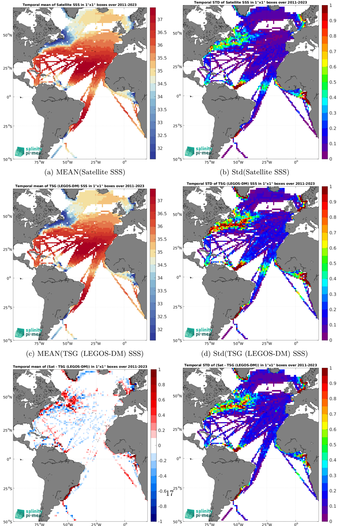
(e) MEAN( \Delta SSS) (Satellite - TSG (LEGOS-DM)) (f) Std( \Delta SSS) (Satellite - TSG (LEGOS-DM)) Figure 7: Temporal mean (left) and Std (right) of SSS from SMAP SSS L4 OI v3 - Daily (ESR) (top), TSG (LEGOS-DM) (middle), and of \Delta SSS (Satellite - TSG (LEGOS-DM)). Only match-up pairs are used to generate these maps.
