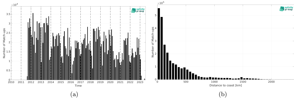
Figure 2: Number of match-ups between TSG (LEGOS-DM) and SMAP SSS L4 OI v3 - Daily (ESR) SSS as a function of time (a) and as function of the distance to coast (b) over the Atlantic Ocean Pi-MEP region and for the full satellite product period.
