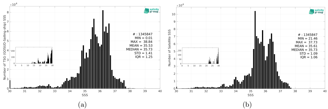
Figure 3: Histograms of SSS from TSG (GOSUD-Sailing-ship) (a) and SMAP SSS L4 OI v3 - Daily (ESR) (b) considering all match-up pairs per bins of 0.1 over the Atlantic Ocean Pi-MEP region and for the full satellite product period.
