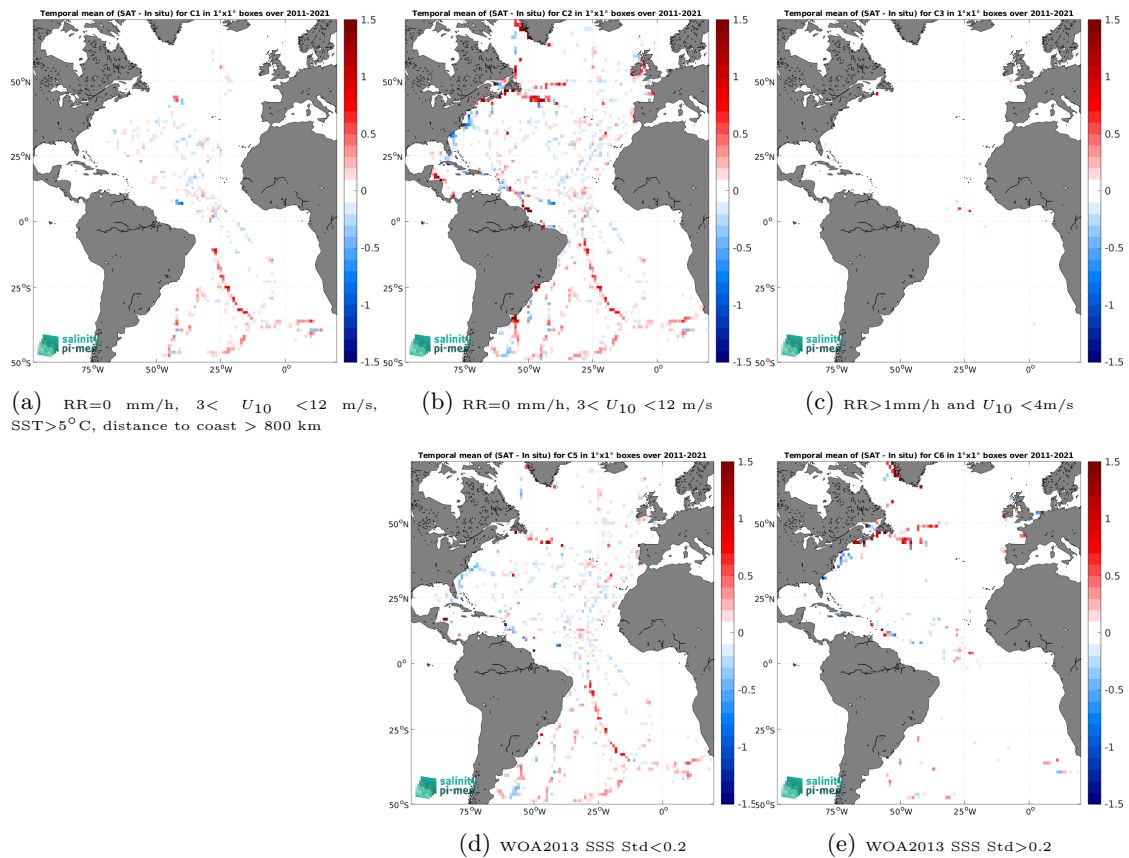
Figure 14: Temporal mean gridded over spatial boxes of size 1^\circ \times 1^\circ of \Delta\text{SSS} (SMAP SSS L4 OI v3 - Daily (ESR) - TSG (GOSUD-Sailing-ship)) for 5 different subdatasets corresponding to:RR=0 mm/h, 3 < U_{10} < 12 m/s, SST>5°C, distance to coast > 800 km (a), RR=0 mm/h, 3 < U_{10} < 12 m/s (b), RR>1mm/h and U_{10} < 4 m/s (c), WOA2013 SSS Std<0.2 (d), WOA2013 SSS Std>0.2 (e).
