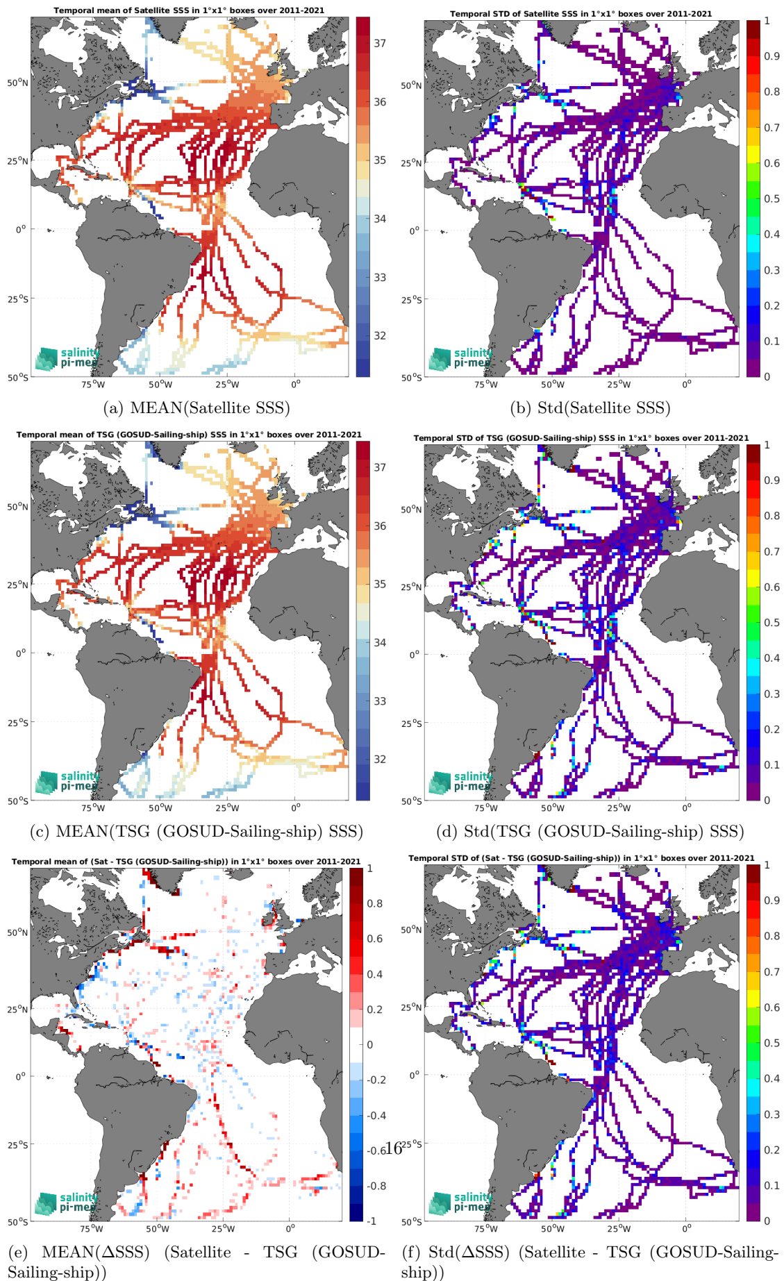
Figure 7: Temporal mean (left) and Std (right) of SSS from SMAP SSS L4 OI v3 - Daily (ESR) (top), TSG (GOSUD-Sailing-ship) (middle), and of \Delta SSS (Satellite - TSG (GOSUD-Sailing-ship)). Only match-up pairs are used to generate these maps.
