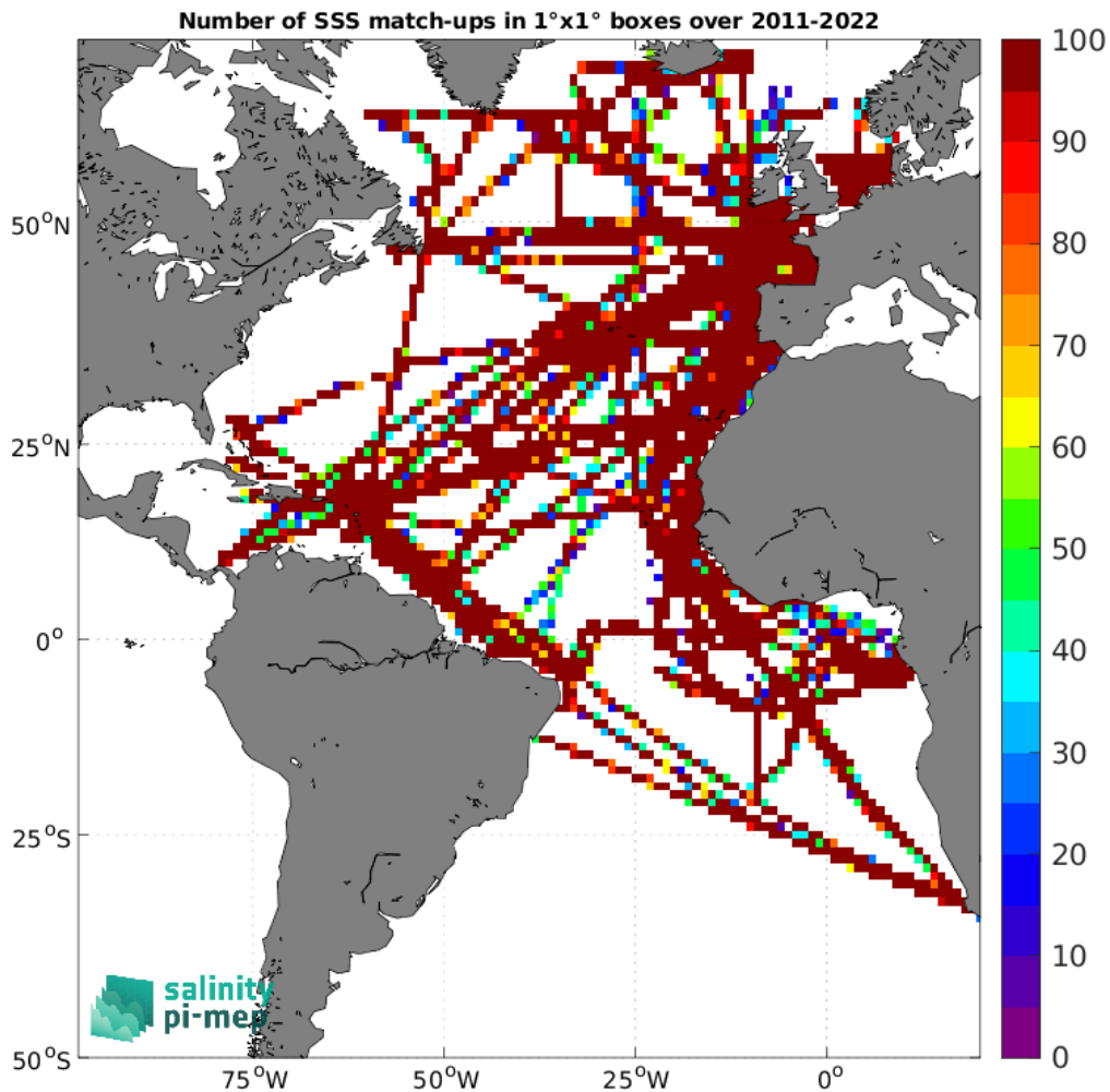
Figure 5: Number of SSS match-ups between TSG (GOSUD-Research-vessel) SSS and the SMAP SSS L4 OI v3 - Daily (ESR) SSS product for the Atlantic Ocean Pi-MEP region over 1^\circ \times 1^\circ boxes and for the full satellite product period.
