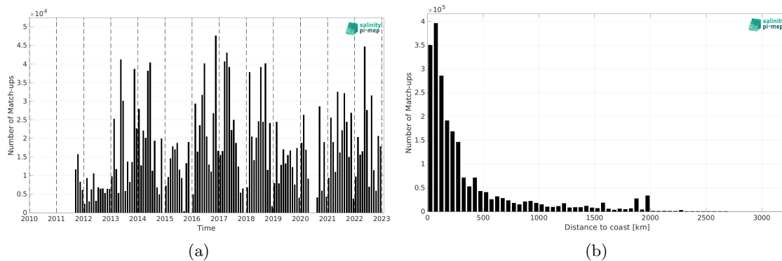
Figure 2: Number of match-ups between TSG (GOSUD-Research-vessel) and SMAP SSS L4 OI v3 - Daily (ESR) SSS as a function of time (a) and as function of the distance to coast (b) over the Atlantic Ocean Pi-MEP region and for the full satellite product period.
