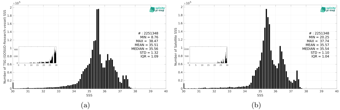
Figure 3: Histograms of SSS from TSG (GOSUD-Research-vessel) (a) and SMAP SSS L4 OI v3 - Daily (ESR) (b) considering all match-up pairs per bins of 0.1 over the Atlantic Ocean Pi-MEP region and for the full satellite product period.
