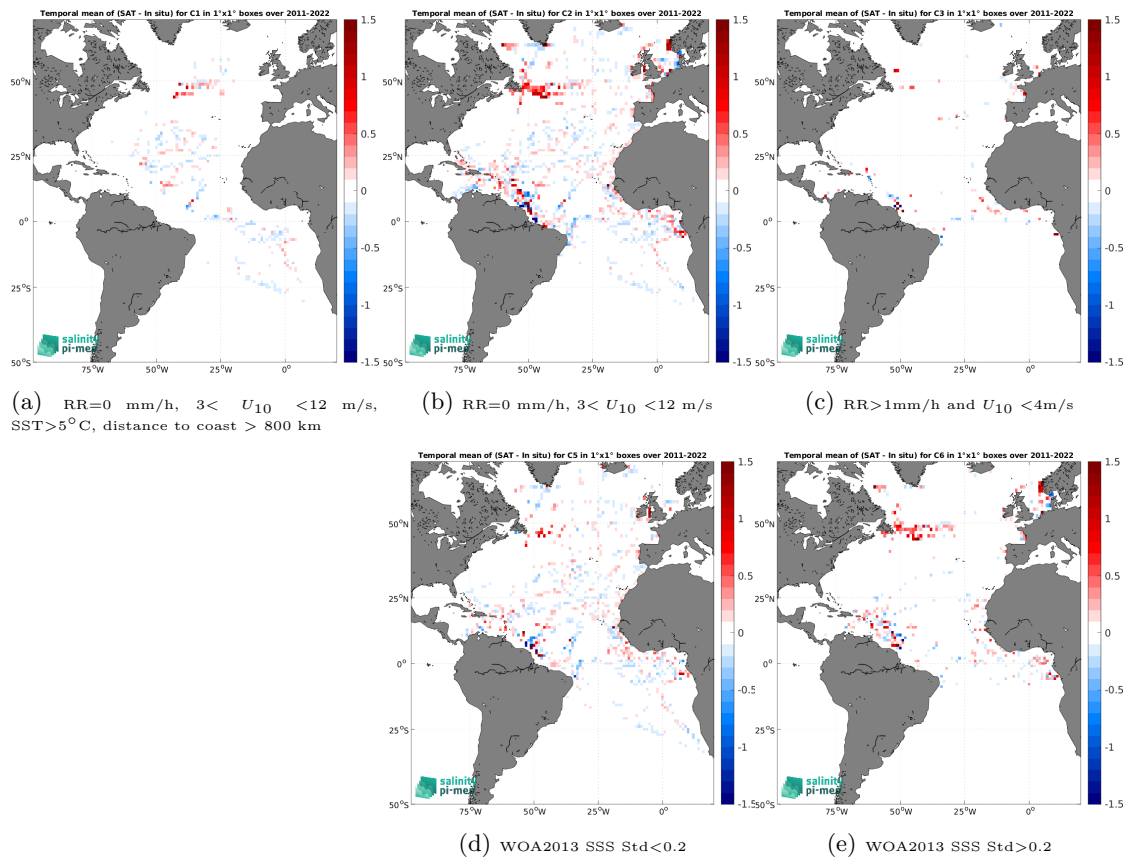
Figure 14: Temporal mean gridded over spatial boxes of size 1^\circ \times 1^\circ of \Delta SSS (SMAP SSS L4 OI v3 - Daily (ESR) - TSG (GOSUD-Research-vessel)) for 5 different subdatasets corresponding to:RR=0 mm/h, 3 < U_{10} < 12 m/s, SST>5°C, distance to coast > 800 km (a), RR=0 mm/h, 3 < U_{10} < 12 m/s (b), RR>1mm/h and U_{10} < 4 m/s (c), WOA2013 SSS Std<0.2 (d), WOA2013 SSS Std>0.2 (e).
