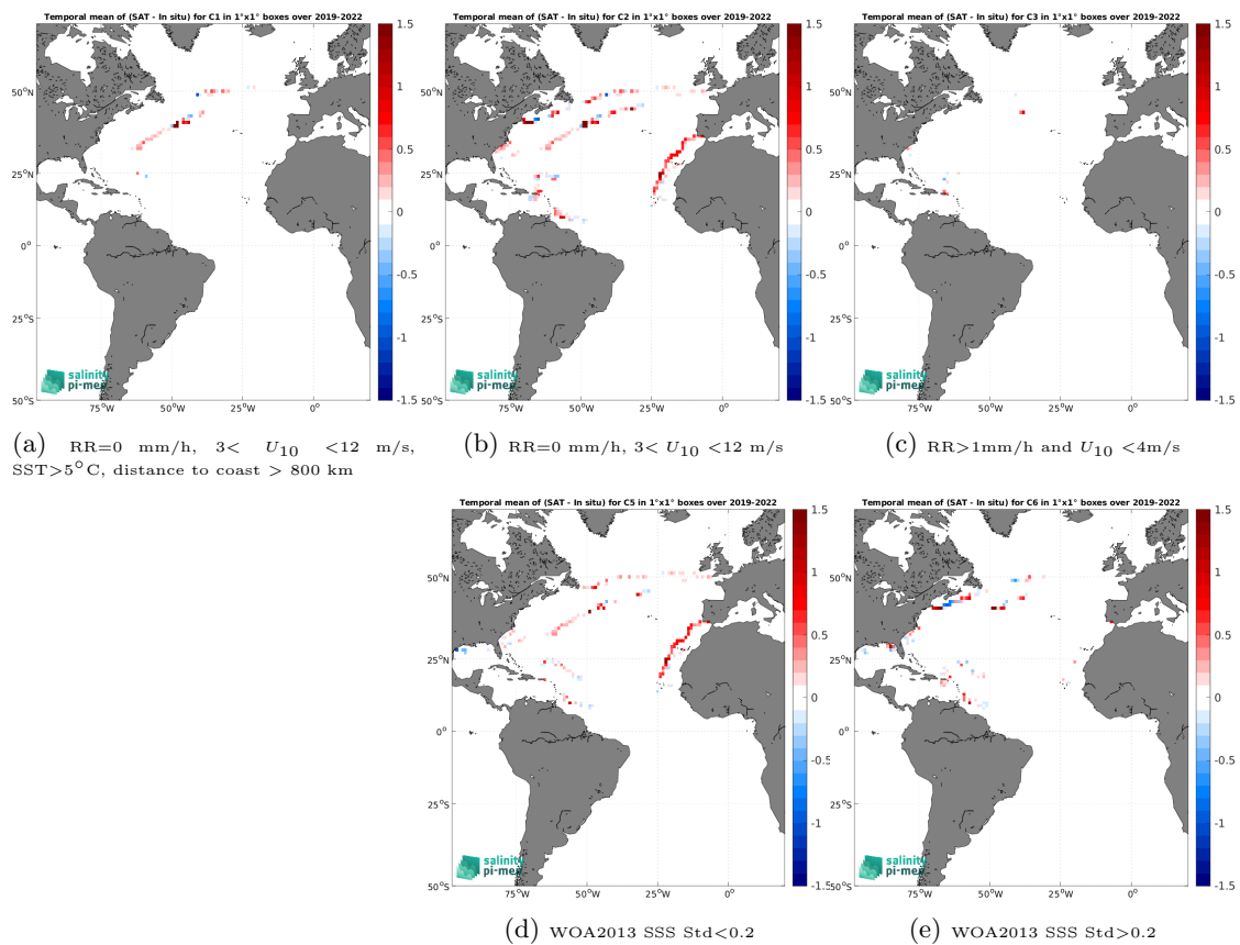
Figure 14: Temporal mean gridded over spatial boxes of size 1^\circ \times 1^\circ of \Delta\text{SSS} (SMAP SSS L4 OI v3 - Daily (ESR) - Saildrone) for 5 different subdatasets corresponding to:RR=0 mm/h, 3 < U_{10} < 12 m/s, SST >5^\circ\text{C} , distance to coast > 800 km (a), RR=0 mm/h, 3 < U_{10} < 12 m/s (b), RR >1 mm/h and U_{10} < 4 m/s (c), WOA2013 SSS Std <0.2 (d), WOA2013 SSS Std >0.2 (e).
