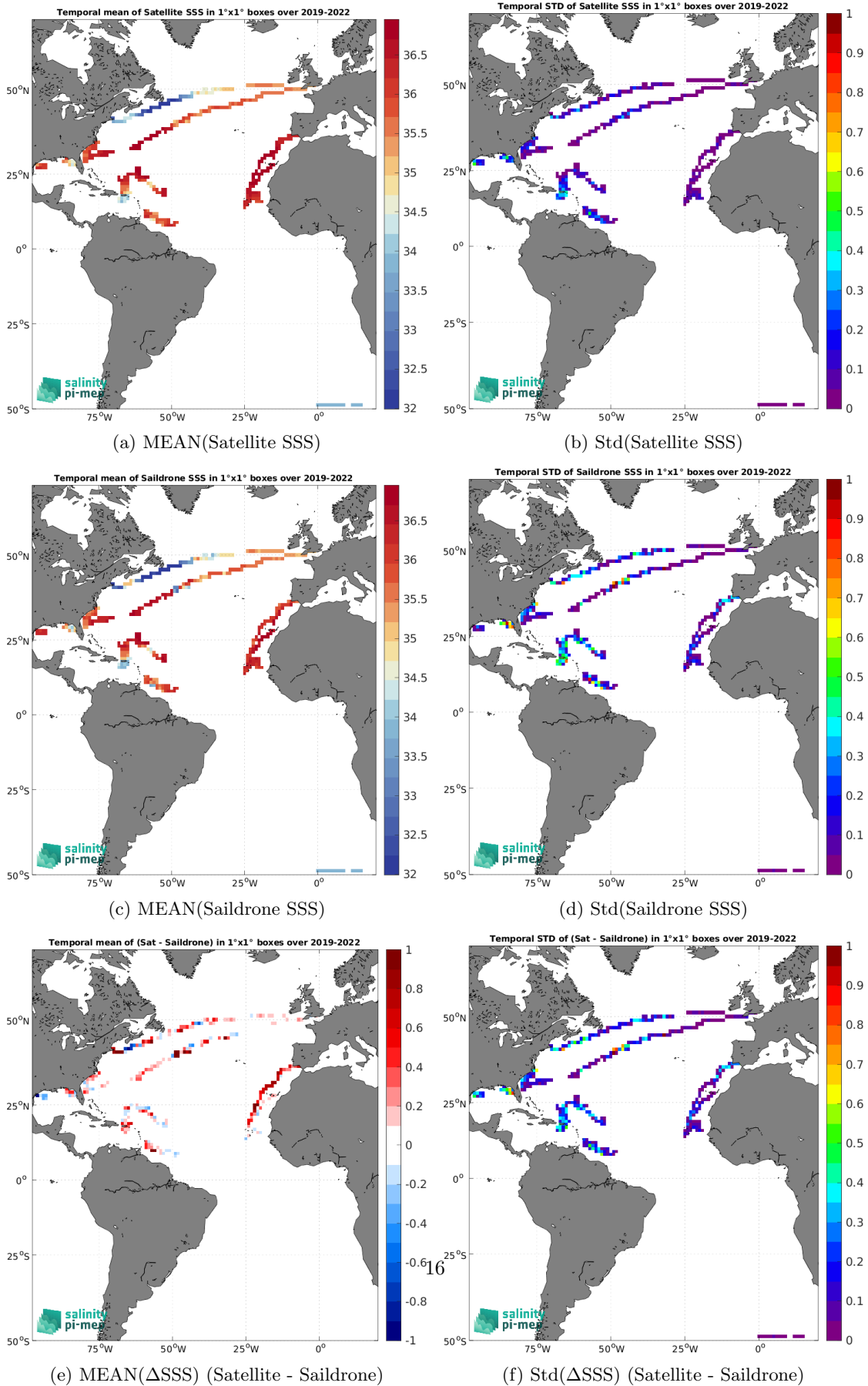
Figure 7: Temporal mean (left) and Std (right) of SSS from SMAP SSS L4 OI v3 - Daily (ESR) (top), Saildrone (middle), and of \Delta SSS (Satellite - Saildrone). Only match-up pairs are used to generate these maps.
