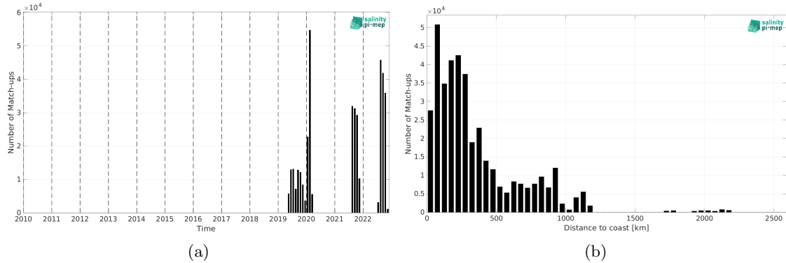
Figure 2: Number of match-ups between Saildrone and SMAP SSS L4 OI v3 - Daily (ESR) SSS as a function of time (a) and as function of the distance to coast (b) over the Atlantic Ocean Pi-MEP region and for the full satellite product period.
