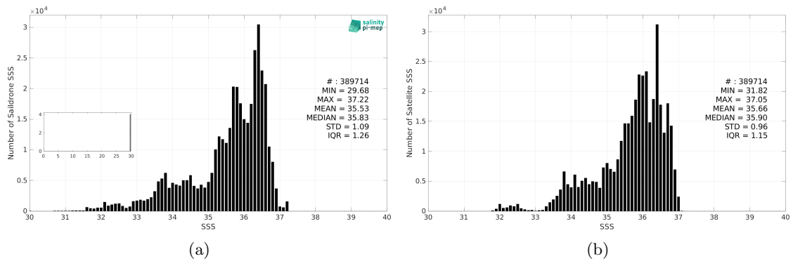
Figure 3: Histograms of SSS from Saildrone (a) and SMAP SSS L4 OI v3 - Daily (ESR) (b) considering all match-up pairs per bins of 0.1 over the Atlantic Ocean Pi-MEP region and for the full satellite product period.
