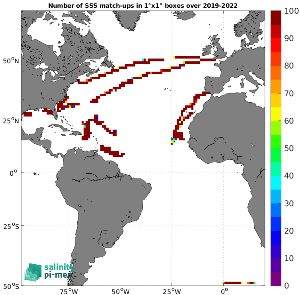
Figure 5: Number of SSS match-ups between Saildrone SSS and the SMAP SSS L4 OI v3 - Daily (ESR) SSS product for the Atlantic Ocean Pi-MEP region over 1^\circ \times 1^\circ boxes and for the full satellite product period.
