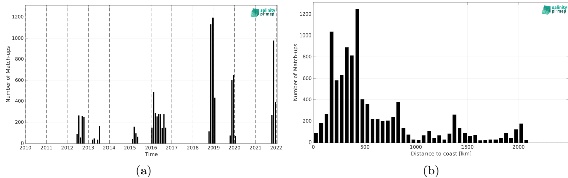
Figure 2: Number of match-ups between Marine mammals and SMAP SSS L4 OI v3 - Daily (ESR) SSS as a function of time (a) and as function of the distance to coast (b) over the Atlantic Ocean Pi-MEP region and for the full satellite product period.
