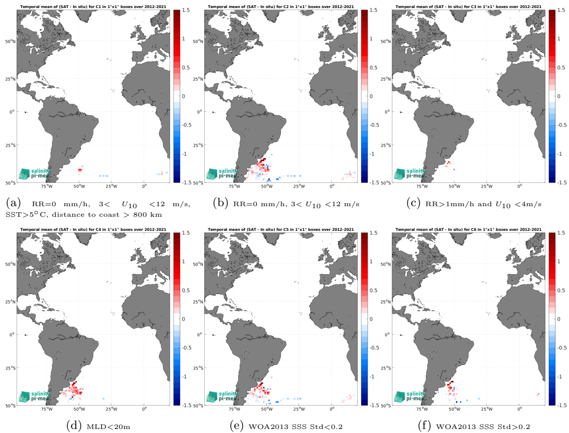
Figure 14: Temporal mean gridded over spatial boxes of size 1^\circ \times 1^\circ of \Delta SSS (SMAP SSS L4 OI v3 - Daily (ESR) - Marine mammals) for 6 different subdatasets corresponding to:RR=0 mm/h, 3 < U_{10} < 12 m/s, SST > 5^\circ\text{C} , distance to coast > 800 km (a), RR=0 mm/h, 3 < U_{10} < 12 m/s (b), RR > 1 mm/h and U_{10} < 4 m/s (c),MLD < 20 m (d),WOA2013 SSS Std < 0.2 (e),WOA2013 SSS Std > 0.2 (f).
