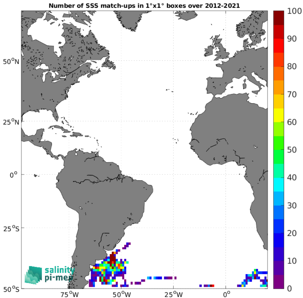
Figure 5: Number of SSS match-ups between Marine mammals SSS and the SMAP SSS L4 OI v3 - Daily (ESR) SSS product for the Atlantic Ocean Pi-MEP region over 1°×1° boxes and for the full satellite product period.
