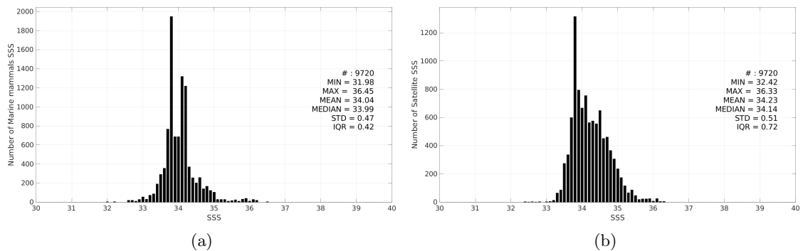
Figure 3: Histograms of SSS from Marine mammals (a) and SMAP SSS L4 OI v3 - Daily (ESR) (b) considering all match-up pairs per bins of 0.1 over the Atlantic Ocean Pi-MEP region and for the full satellite product period.
