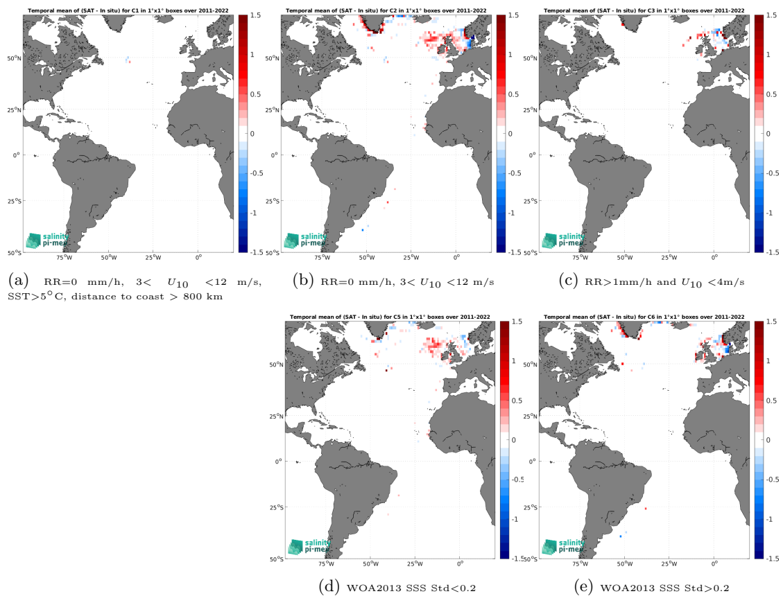
Figure 14: Temporal mean gridded over spatial boxes of size 1^\circ \times 1^\circ of \Delta\text{SSS} (SMAP SSS L4 OI v3 - Daily (ESR) - ICES) for 5 different subdatasets corresponding to:RR=0 mm/h, 3 < U_{10} < 12 m/s, SST>5°C, distance to coast > 800 km (a), RR=0 mm/h, 3 < U_{10} < 12 m/s (b), RR>1mm/h and U_{10} < 4 m/s (c), WOA2013 SSS Std<0.2 (d), WOA2013 SSS Std>0.2 (e).
