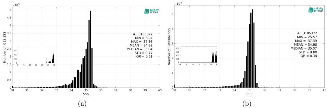
Figure 3: Histograms of SSS from ICES (a) and SMAP SSS L4 OI v3 - Daily (ESR) (b) considering all match-up pairs per bins of 0.1 over the Atlantic Ocean Pi-MEP region and for the full satellite product period.
