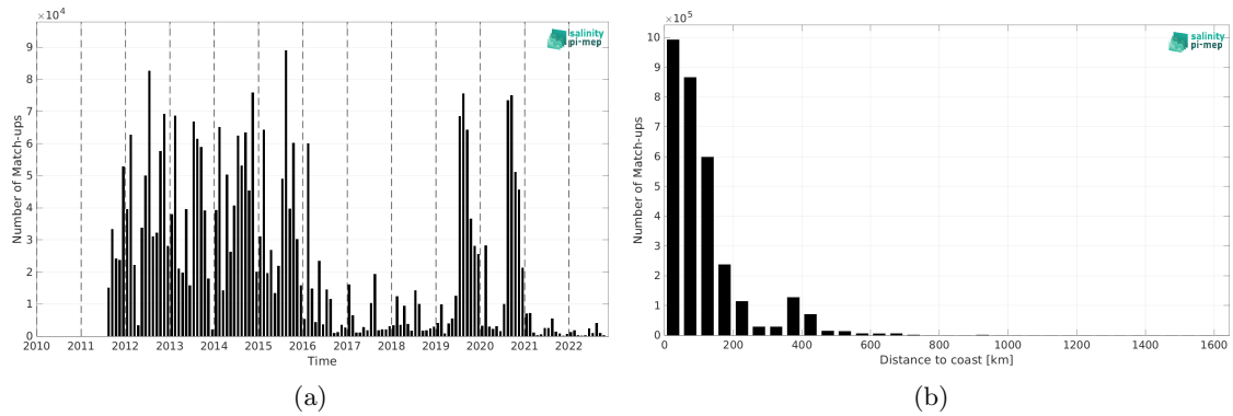
Figure 2: Number of match-ups between ICES and SMAP SSS L4 OI v3 - Daily (ESR) SSS as a function of time (a) and as function of the distance to coast (b) over the Atlantic Ocean Pi-MEP region and for the full satellite product period.
