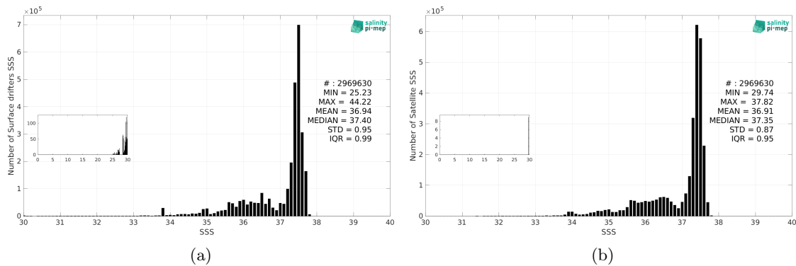
Figure 3: Histograms of SSS from Surface drifters (a) and SMAP SSS L4 OI v3 - Daily (ESR) (b) considering all match-up pairs per bins of 0.1 over the Atlantic Ocean Pi-MEP region and for the full satellite product period.
