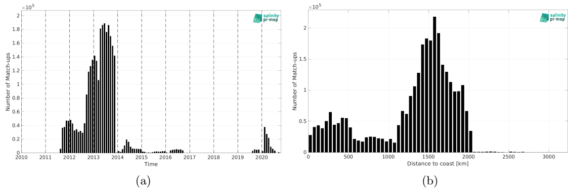
Figure 2: Number of match-ups between Surface drifters and SMAP SSS L4 OI v3 - Daily (ESR) SSS as a function of time (a) and as function of the distance to coast (b) over the Atlantic Ocean Pi-MEP region and for the full satellite product period.
