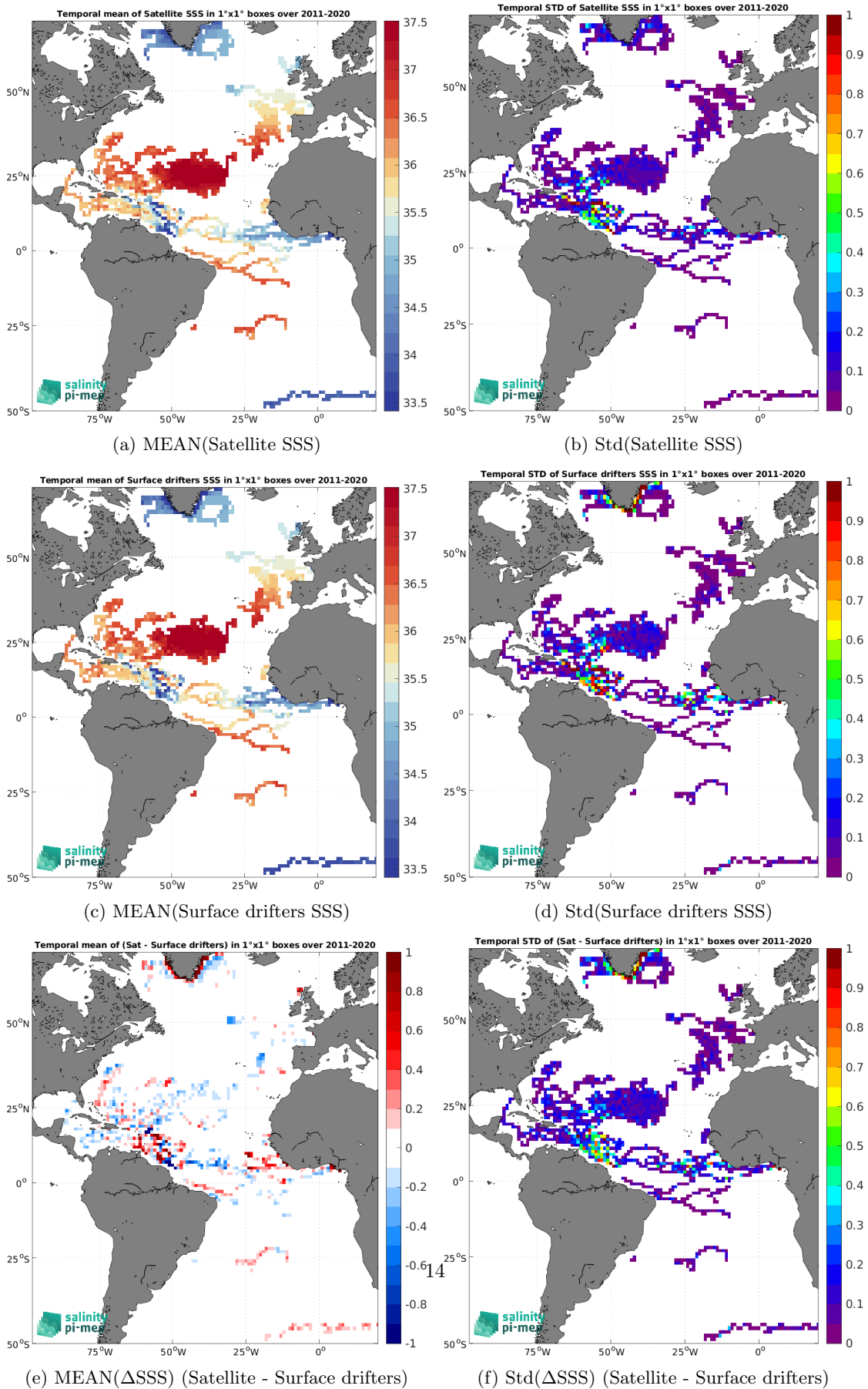
Figure 6: Temporal mean (left) and Std (right) of SSS from SMAP SSS L4 OI v3 - Daily (ESR) (top), Surface drifters (middle), and of \Delta SSS (Satellite - Surface drifters). Only match-up pairs are used to generate these maps.
