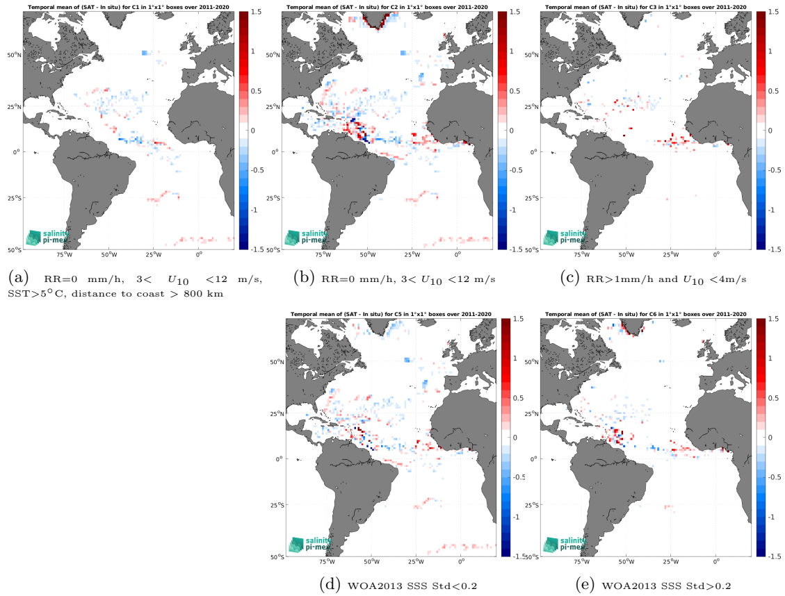
Figure 13: Temporal mean gridded over spatial boxes of size 1^\circ \times 1^\circ of \Delta SSS (SMAP SSS L4 OI v3 - Daily (ESR) - Surface drifters) for 5 different subdatasets corresponding to:RR=0 mm/h, 3 < U_{10} < 12 m/s, SST >5^\circ\text{C} , distance to coast > 800 km (a), RR=0 mm/h, 3 < U_{10} < 12 m/s (b), RR >1 mm/h and U_{10} < 4 m/s (c), WOA2013 SSS Std <0.2 (d), WOA2013 SSS Std >0.2 (e).
