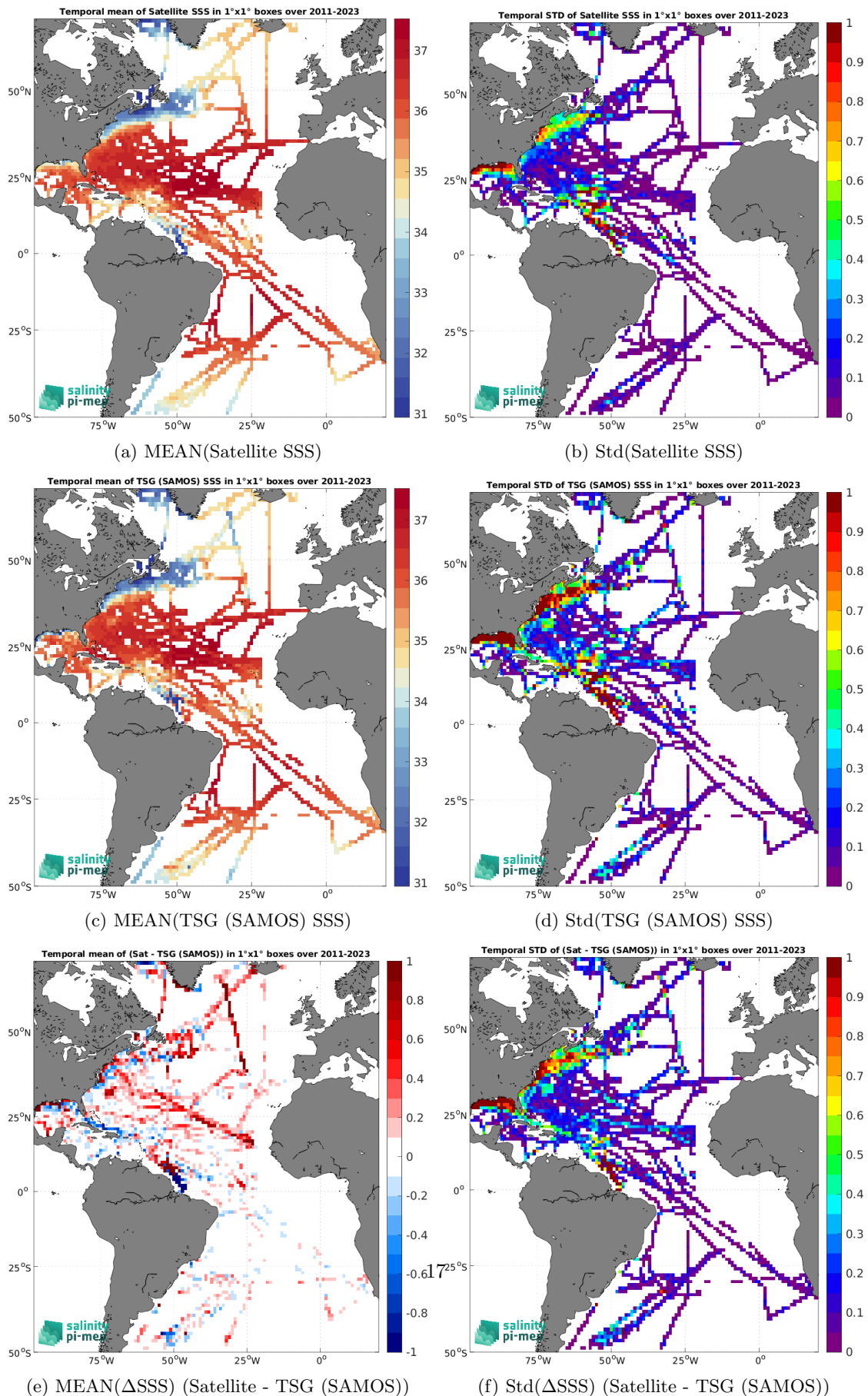
Figure 6: Temporal mean (left) and Std (right) of SSS from SMAP SSS L4 OI v2 - 7 Days (ESR) (top), TSG (SAMOS) (middle), and of \Delta SSS (Satellite - TSG (SAMOS)). Only match-up pairs are used to generate these maps.
