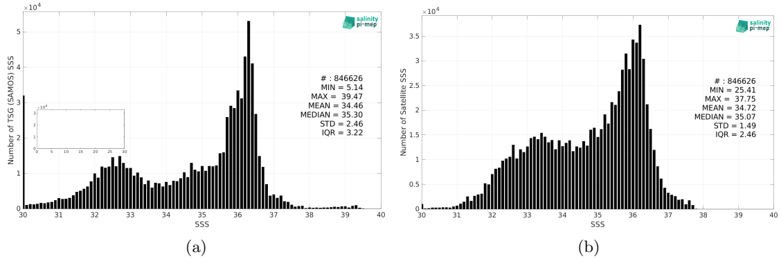
Figure 2: Histograms of SSS from TSG (SAMOS) (a) and SMAP SSS L4 OI v2 - 7 Days (ESR) (b) considering all match-up pairs per bins of 0.1 over the Atlantic Ocean Pi-MEP region and for the full satellite product period.
