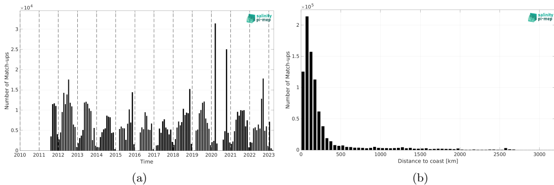
Figure 1: Number of match-ups between TSG (SAMOS) and SMAP SSS L4 OI v2 - 7 Days (ESR) SSS as a function of time (a) and as function of the distance to coast (b) over the Atlantic Ocean Pi-MEP region and for the full satellite product period.
