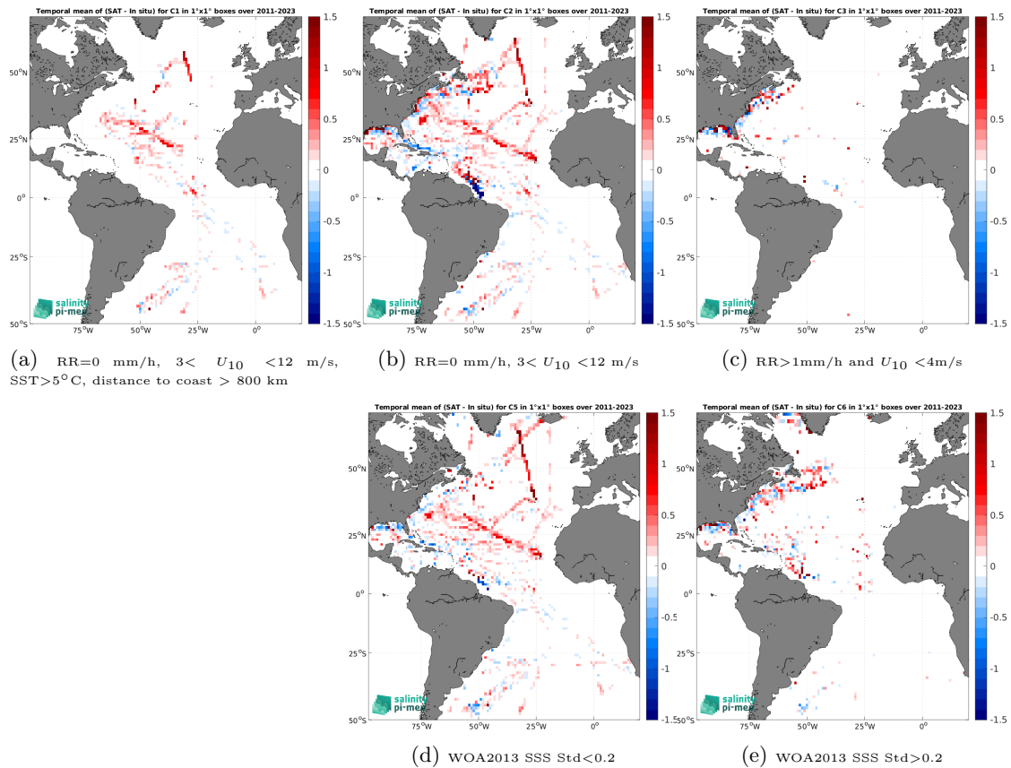
Figure 12: Temporal mean gridded over spatial boxes of size 1^\circ \times 1^\circ of \Delta SSS (SMAP SSS L4 OI v2 - 7 Days (ESR) - TSG (SAMOS)) for 5 different subdatasets corresponding to:RR=0 mm/h, 3 < U_{10} < 12 m/s, SST >5^\circ\text{C} , distance to coast > 800 km (a), RR=0 mm/h, 3 < U_{10} < 12 m/s (b), RR >1 mm/h and U_{10} < 4 m/s (c), WOA2013 SSS Std <0.2 (d), WOA2013 SSS Std >0.2 (e).
