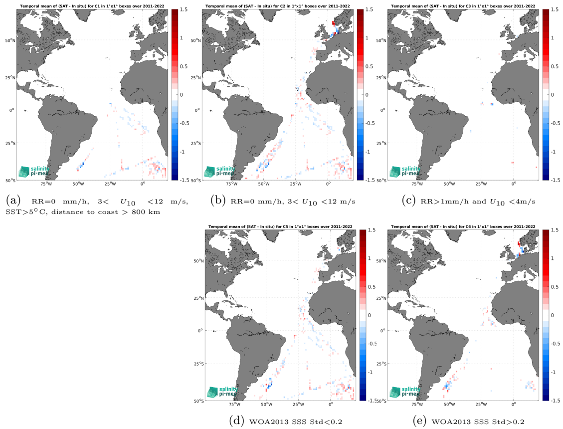
Figure 12: Temporal mean gridded over spatial boxes of size 1^\circ \times 1^\circ of \Delta\text{SSS} (SMAP SSS L4 OI v2 - 7 Days (ESR) - TSG (Polarstern)) for 5 different subdatasets corresponding to:RR=0 mm/h, 3 < U_{10} < 12 m/s, SST >5^\circ\text{C} , distance to coast > 800 km (a), RR=0 mm/h, 3 < U_{10} < 12 m/s (b), RR >1 mm/h and U_{10} < 4 m/s (c), WOA2013 SSS Std <0.2 (d), WOA2013 SSS Std >0.2 (e).
