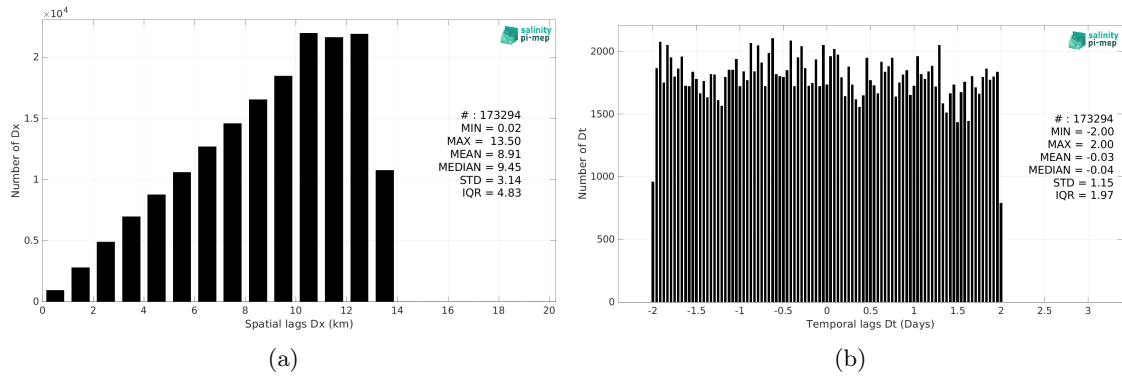
Figure 5: Histograms of the spatial (a) and temporal (b) lags between the location/time of the TSG (Polarstern) measurement and the date of the corresponding SMAP SSS L4 OI v2 - 7 Days (ESR) SSS pixel.
