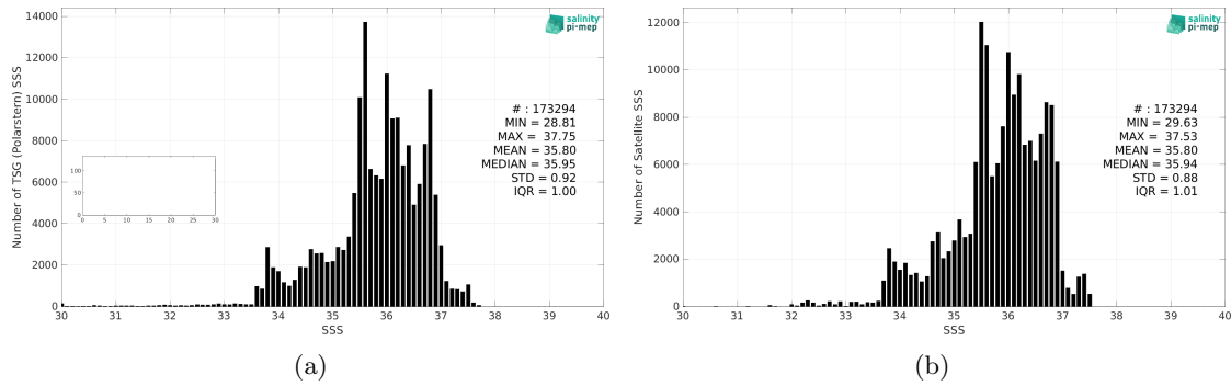
Figure 2: Histograms of SSS from TSG (Polarstern) (a) and SMAP SSS L4 OI v2 - 7 Days (ESR) (b) considering all match-up pairs per bins of 0.1 over the Atlantic Ocean Pi-MEP region and for the full satellite product period.
